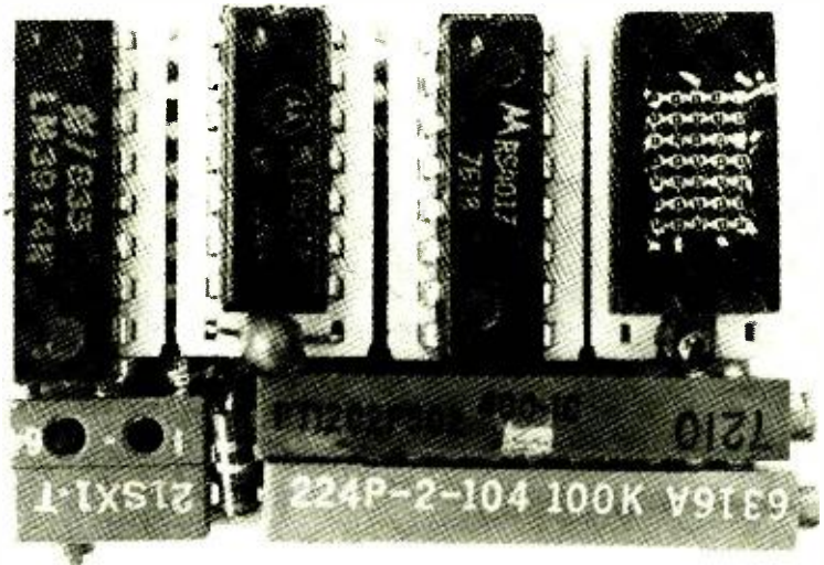
Fig. 2. Photograph of the wrapped-wire prototype LED oscilloscope assembled on a small piece of perforated board about 1.2'' \times 1.2'' .
