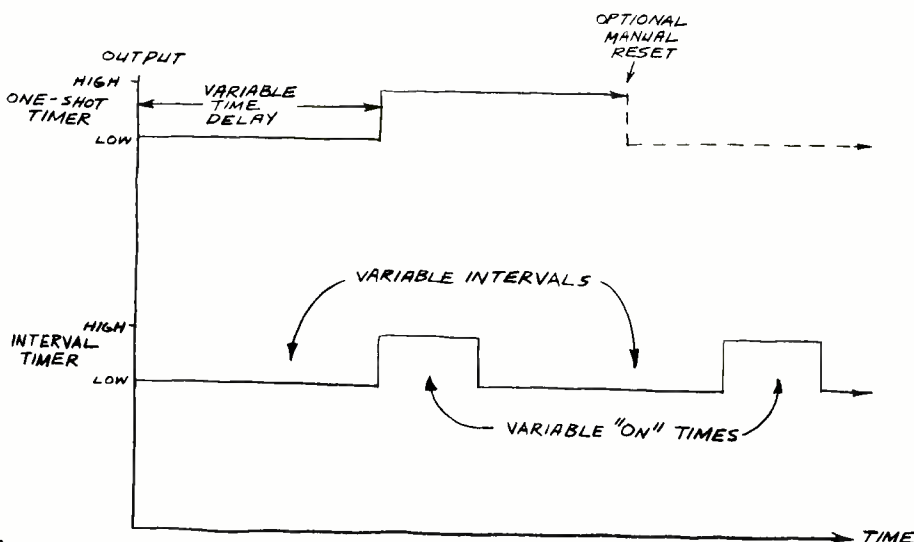
Fig. 1. Timing diagrams of the output waveforms generated by monostable multivibrator or one-shot (top) and interval timer (bottom).
