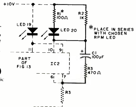
Fig. 16 Tachometer add-on is used to identify critical cruising speed.
