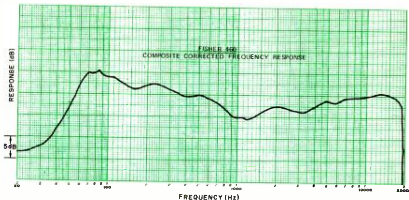
Composite corrected frequency response for ST460 Speaker System.
