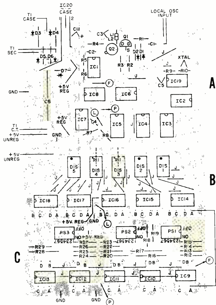
Fig. 5. Parts placement guides for main (top), display (center), and counter (bottom) pc boards.
