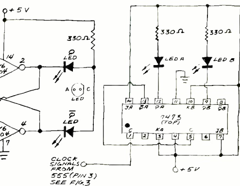
Fig. 4. Two-bit counter made from 7473 dual flip-flop.
