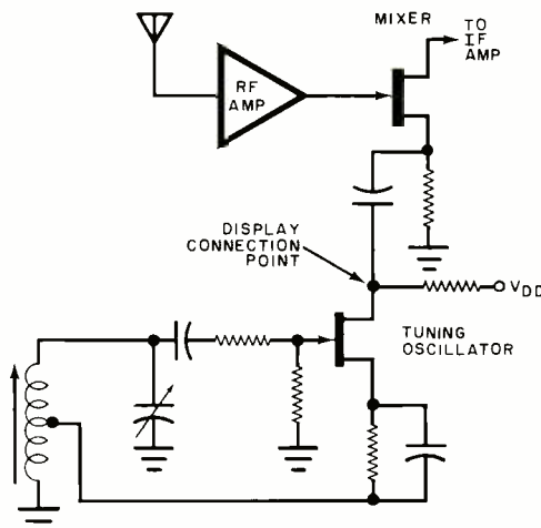
Fig. 6. Typical local oscillator circuit
