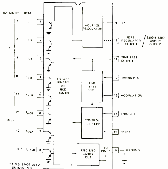
Fig. 1. Pin connections for 8240/50/60.
