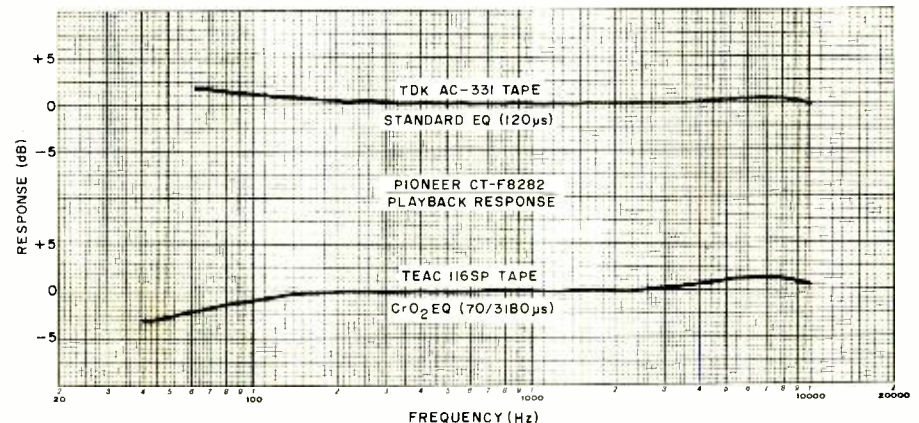
Playback response with two tapes at different equalization settings.
