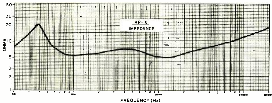
Impedance curve shows peak slightly below rated system resonance.
