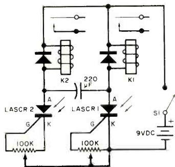
Fig. 5. Circuit for a remote light-operated switch.
