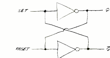
Fig. 1. The basic flip-flop.
