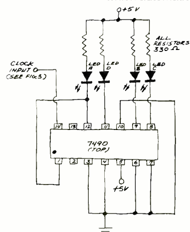
Fig. 5. 7490 four-bit counter.
