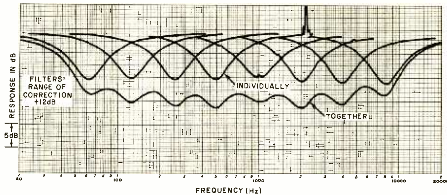
Fig. 5. Combining filters used individually and in concert. Note that the effect of all controls exceeds that of only one.
