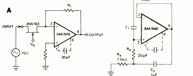
Fig. 1. Op amp applications: (A) gain-controlled amplifier; (B) notch filter.
