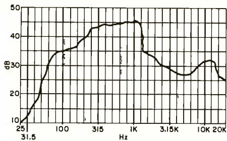
Fig. 2. Dynamic spectrum of a popular recording, measured on the same analyzer as Fig. 1.
