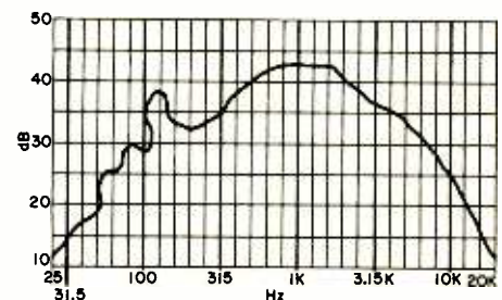
Fig. 1. Dynamic spectrum of a classical recording, measured on a real-time analyzer.
