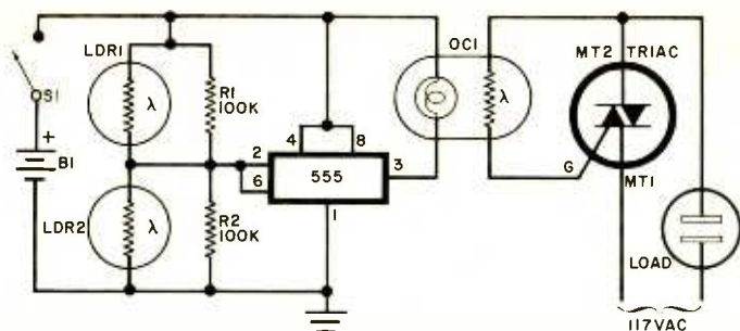
Fig. 3. An opto-coupler controls triac gate current.
