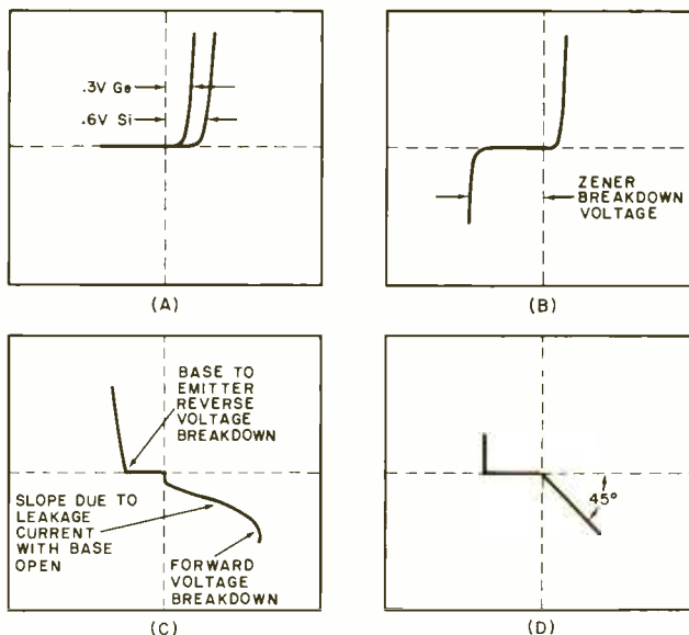
Fig. 2. Typical scope traces: (A) identification of silicon or germanium junction; (B) zener diode curve; (C) transistor with leakage, forward breakdown voltage, reverse breakdown; (D) transistor with a gain of 100.
