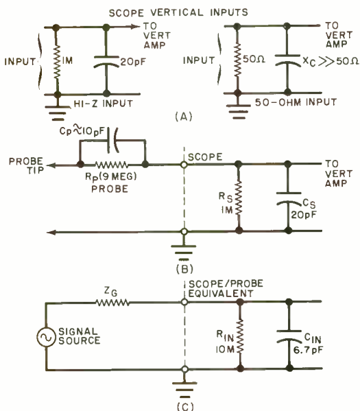
Fig. 1. Typical scope inputs: (A) for high- and low-impedance scopes; (B) with a passive divider probe; (C) equivalent circuit of combination in (B).
