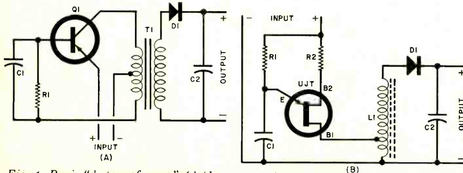
Fig. 1. Basic "dc transformer" (dc/dc converter) circuits using a transistor (A) and a UJT (B).
