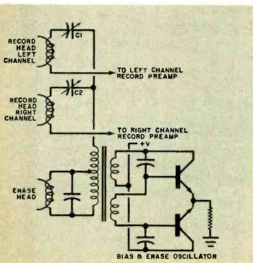
Fig. 5. Partial schematic shows how bias is adjusted by trimming C1 and C2 .
