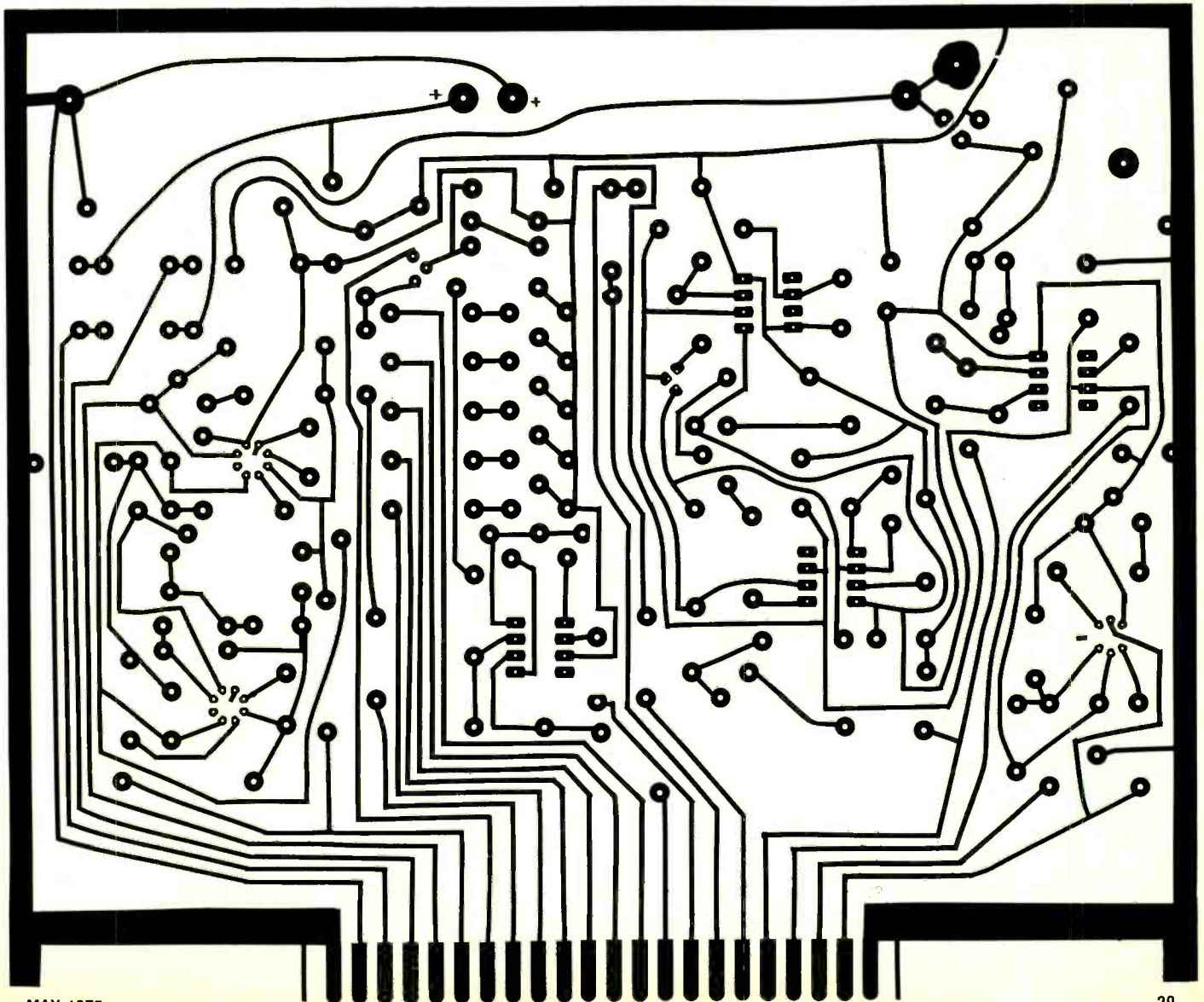
Fig. 2. Actual-size foil pattern for pc board is below, component layout on opposite page.
