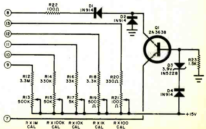
Fig. G. Constant-current generator for resistance tests.
