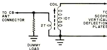
Fig. 1. CB-to-scope coupler. The resistive dummy load and adjustable r-f transformer are easily made from "junk-box" parts.
