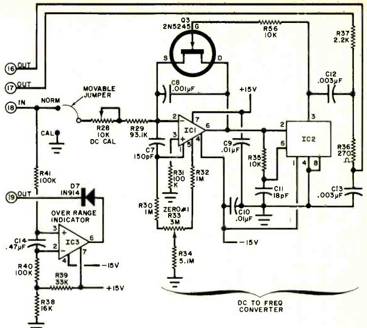
Fig. C. Over-range indicator circuit drives LED1.
