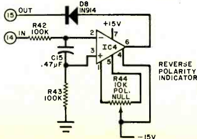
Fig. E. Reverse-polarity indicator.
