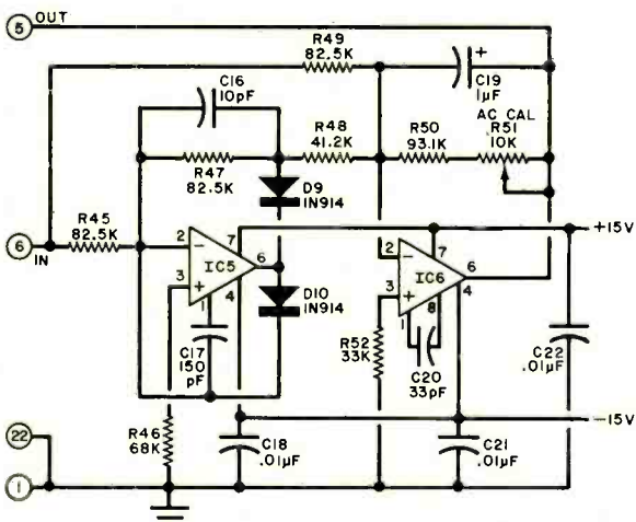
Fig. D. Ac-to-dc converter is a rectifier.
