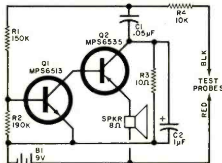
Schematic of easy-to-build tester.
