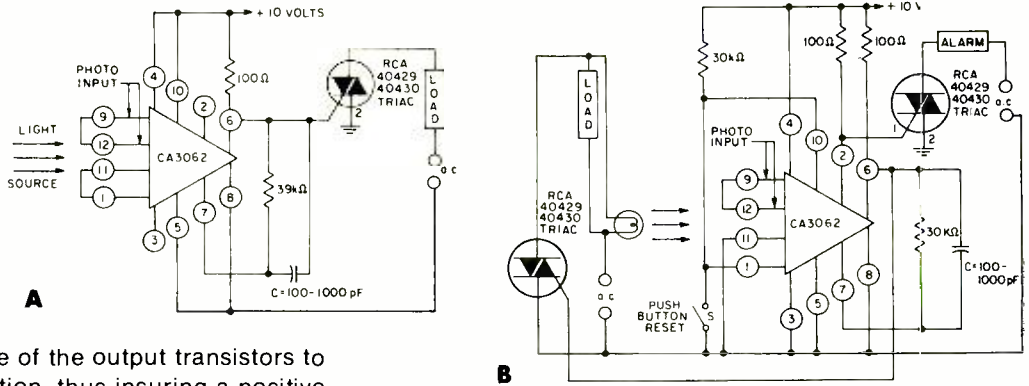
Fig. 2. Typical applications for the CA3062. (A) is a light-activated triac control; while (B) is triac control with automatic shutoff.
