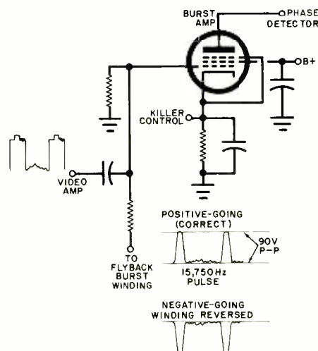
Burst amplifier has video input plus spike from the flyback.
