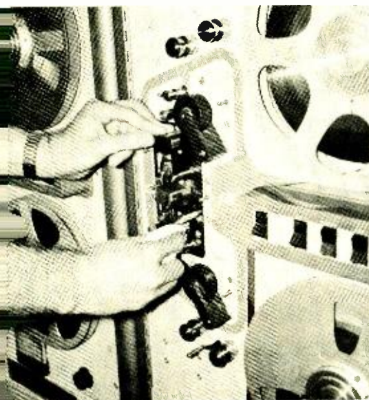
Technician checks ten-channel tape recorder used to make semi-permanent record of communications between controllers and aircraft.
