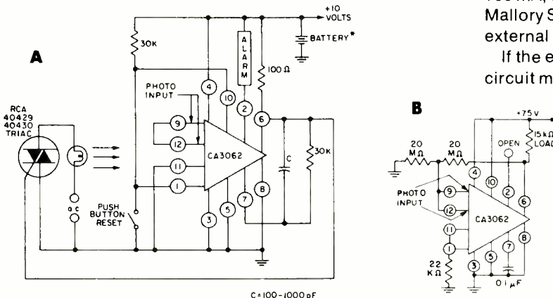
Fig. 3. Circuit shown at (A) is a modification of Fig. 2B to provide an intrusion alarm. A linear photoelectric amplifier can be built as shown at (B).
