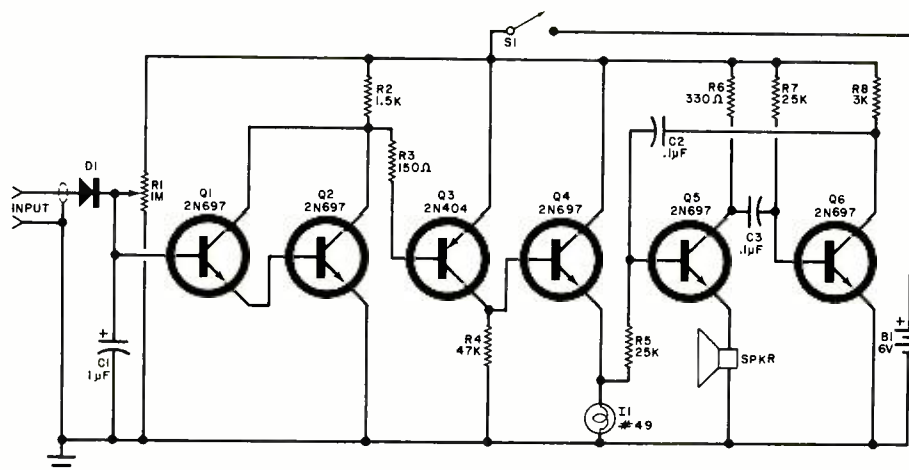
Fig. 5. Circuit to forecast storms uses discrete devices.
