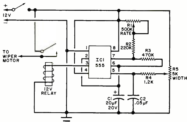
Fig. 4. Slow-sweep wiper control.
