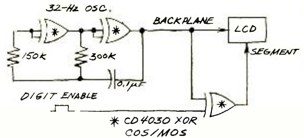
Fig. 4. Standard driver configuration for an LC display.
