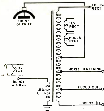
Flyback transformer has special winding to generate spikes.
