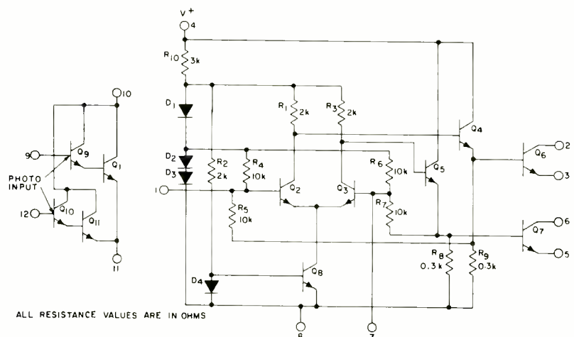
Fig. 1. The CA3062 photo detector and power amplifier consists of a photo-Darlington pair and a differential amplifier coupled to uncommitted output transistors.
