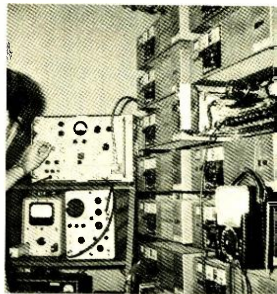
Some of the test equipment used to check a 70-MHz i-f strip in a 6-channel radar information microwave link repeater site.
