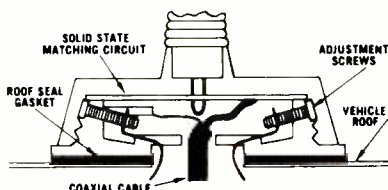
Hy-Gain rooftop mounting system.
