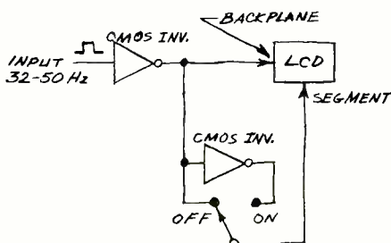
Fig. 3. Practical circuit for driving an LC display.
