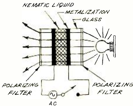
Fig. 2. Basic theory of how liquid crystal display works.
