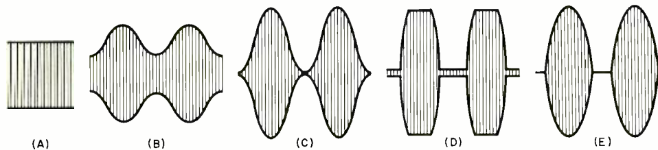
Fig. 2. R-f envelopes of an AM transmitter: (A) unmodulated; (B) 50% modulation; (C) 100%. Clipping (D) and overmodulation (E) cause station interference.
