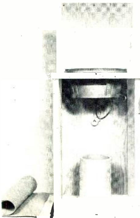
Fig. 3. With top panel temporarily in place, strike leading-edge line of reflector.
