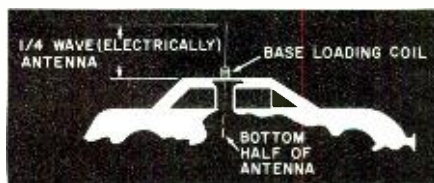
Fig. 1. Loading antenna improves impedance match and shortens length. Automobile provides ground plane and bottom half of the antenna.
