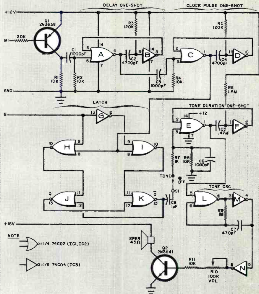
Fig. 2. The beeper circuit uses CMOS equivalents of conventional TTL chips. Inputs are units of minutes (M1), and minutes readout of B segment. The beep occurs on 4/5 transition.
