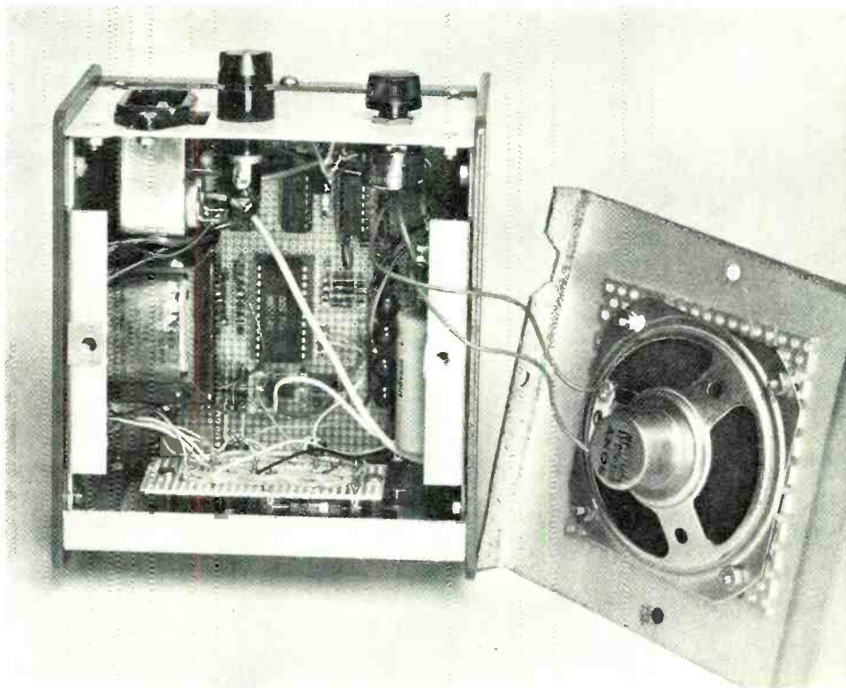
Photo shows internal arrangement of the prototype.
