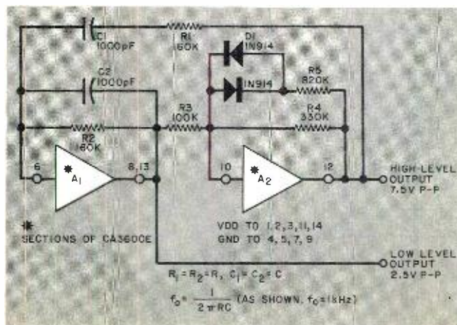
Fig. 4. Wien bridge sine-wave oscillator uses a pair of conventional CMOS inverters.
