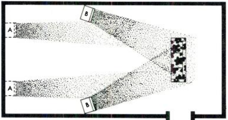
Fig. 2. "Toeing in" the speakers and moving them from locations A to locations B increases the level of high-frequency energy at the listening area. Precise positioning depends on room-mode activity.
