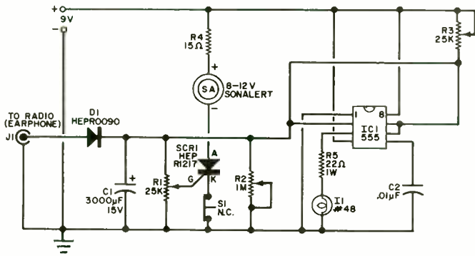
Fig. 3. A reader's version of the low-cost Stormcaster project using a 555 IC timer.
