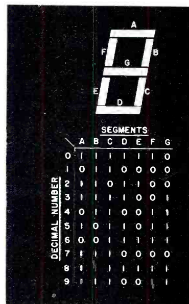
Fig. 3. Signals required for each digit of a 7-segment readout.
