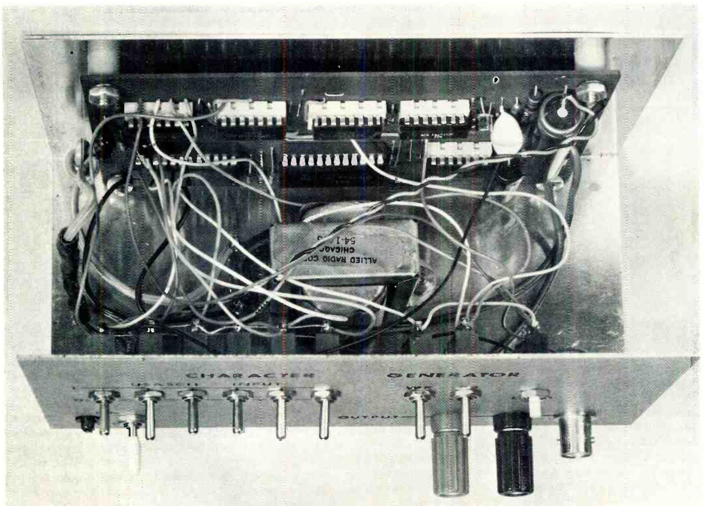
This photo shows how the prototype of the character generator was assembled.
