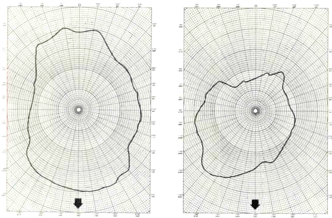
Fig. 2. Typical horizontal radiation patterns when a vertical whip antenna is mounted on the roof (at
