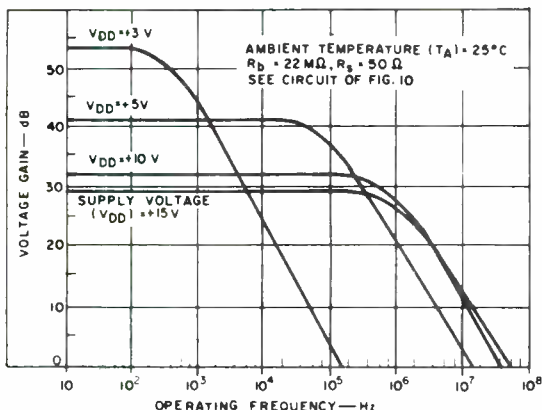
Fig. 2. Gain and bandwidth of RCA CMOS inverter vary with supply voltage.
