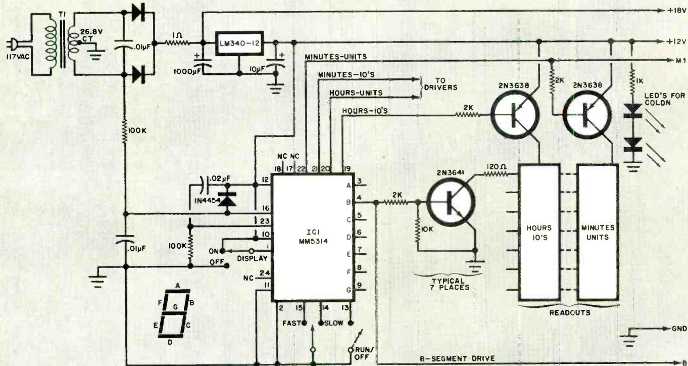
Fig. 1. A basic 24-hour digital clock circuit using an MM5314 IC. Other digital clock circuits could be used with the beeper. Note that only the units-of-minutes driver signal and the readout B-segment signal are used to drive the beeper circuit. If interference is too bad, an r-f decoupling filter can be used.
