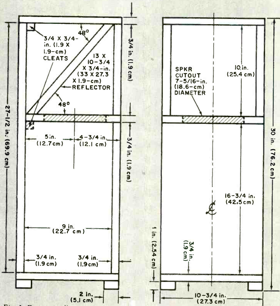
Fig. 1. Drawings illustrate how enclosure goes together and details of reflector assembly.
