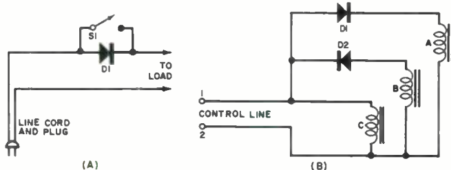
Fig. 2. Circuit (A) shows use of diode in a dual level power control; (B) is simple remote control.
