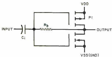
Fig. 1. A CMOS inverter biased for linear operation.
