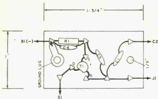
Fig. 2. Diagram shows how components are laid out on a perforated phenolic board.
