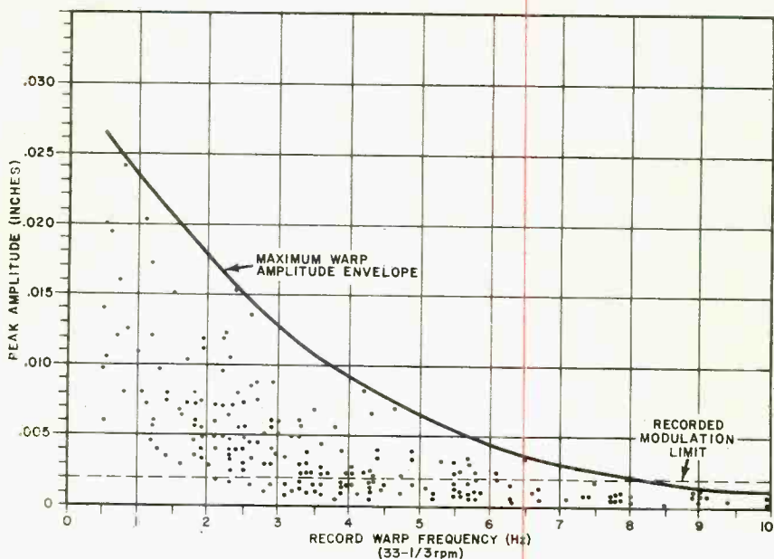
Fig. 1. The distribution of the warps measured by Shure on 67 LP records. Each dot indicates the amplitude and frequency of one of the warps that was found. The dashed line indicates typical maximum recorded amplitudes (about 2 mils).
