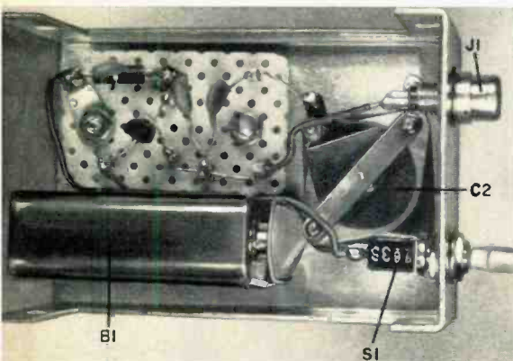
Fig. 3. Photo of prototype showing how the board and components go into chassis.
