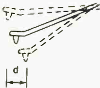
Fig. 2. Warp problems can produce severe vertical deflections of stylus assemblies, causing the tip to move forward and back in the groove over distance d . This imposes a "wow" modulation on music. Tone arms, especially shorter ones, are also subject to the effect.
