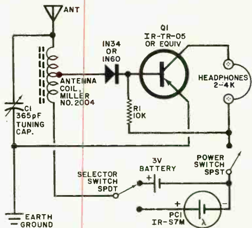
Fig. 6. Sun-powered emergency radio receiver.
