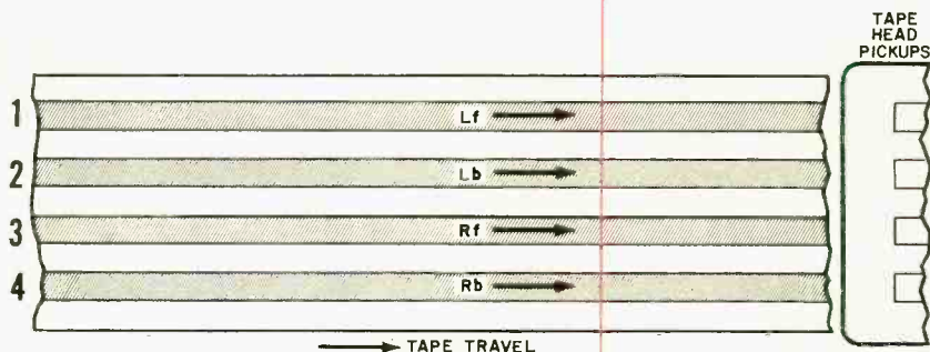
Fig. 2. In 4-channel open-reel, all four tracks are played at once.
