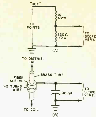
Checking ignition with an oscilloscope.
