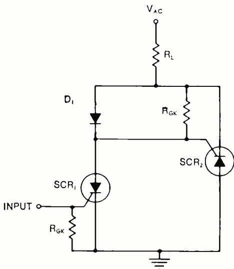
Fig. 3. SCR triac replacement circuit.
