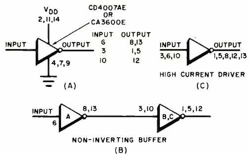
Fig. 1. Using the CMOS as a triple inverter (A), a noninverting buffer (B), and (C) as high-current driver with units in parallel.
