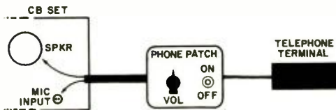
Fig. 2. Diagram of how a phone-patch installation is connected at CB base station.
