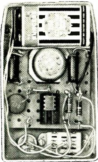
Photo shows how author's prototype, using perf board, fits in transistor radio case.
