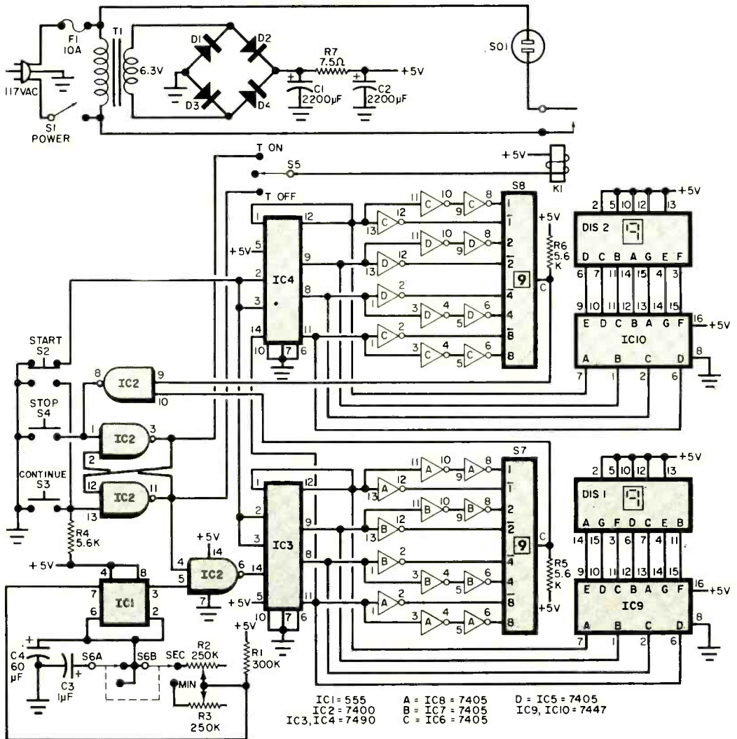
Fig. 1. The basic timing interval is generated by IC1, while IC3 and IC4 are decade counters. The displays are driven by IC9 and IC10. Thumbwheel switches S7 and S8 form a value detector for individual numeric selections.
