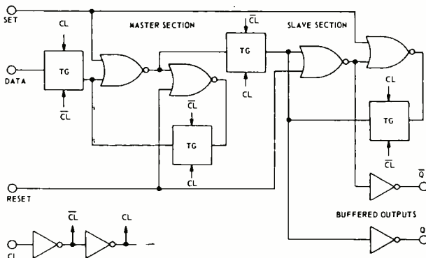
Fig. 6. Block diagram of one section of an RCA CD4013AE COS/MOS type D flip-flop unit.
