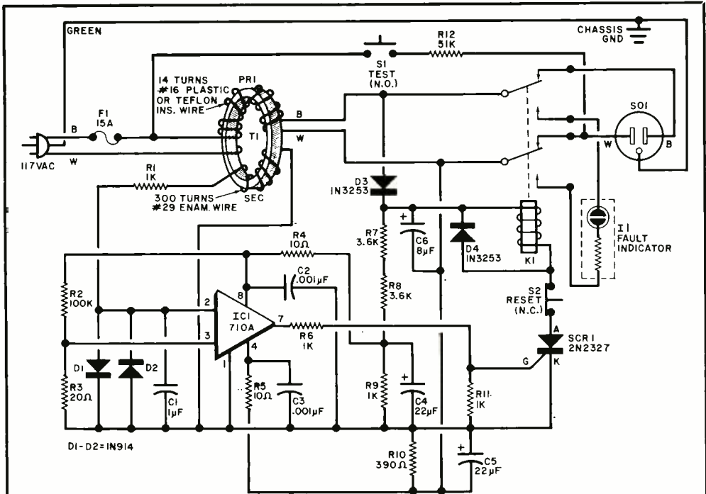
Fig. 1. When the secondary of T1 senses an imbalance in the two power-line feeds, the difference is amplified and turns on SCR1, which cuts the power to the socket.
