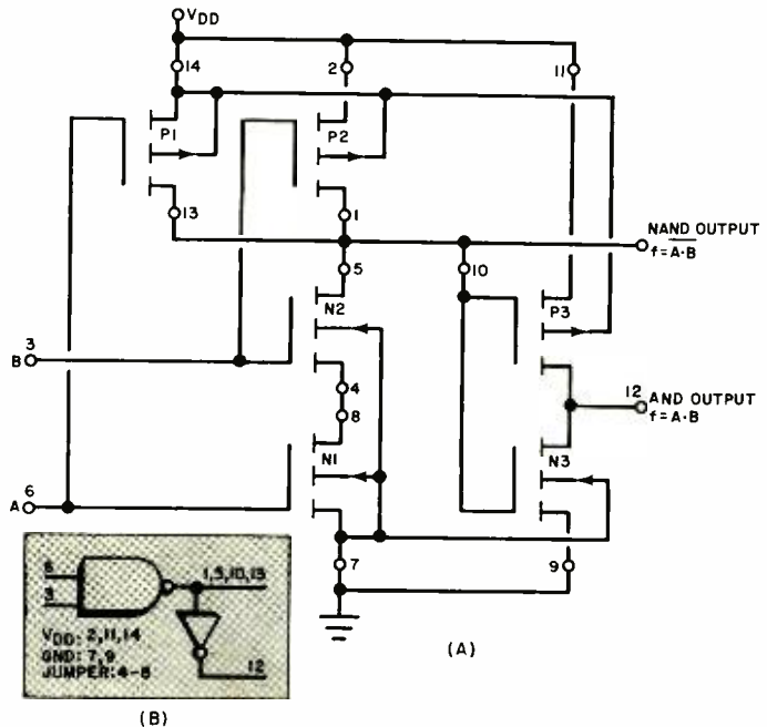
Fig. 3. The interconnections for a NAND or AND circuit are similar to those in Fig. 2, with units upside down. Symbol is at (B).
