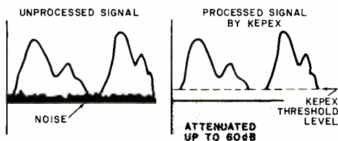
Fig. 4. Waveforms show how Kepex device effectively cancels leakage between mikes.
