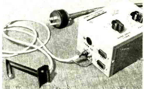
Fig. 3. Overall view of controller. Bracket which holds the LDR sensor is extreme left.
