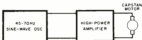
Fig. 1. A sine-wave oscillator and amplifier circuit control speed of tape recorder motor.
