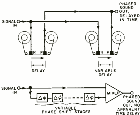
Fig. 2. Phasing (to get "spacey" effects) was formerly accomplished by running the signal through two tape decks, with different delays (top diagram). Now, a series of electronic stages with variable shifts accomplishes same thing (bottom diagram).
