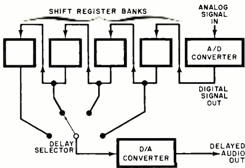
Fig. 3. Schematic of digital delay line that is used for phasing and effects such as reverb.
