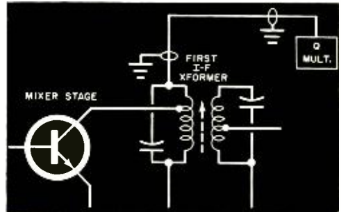
Fig. 3. Diagram shows how to connect the Q multiplier into your receiver using coax.
