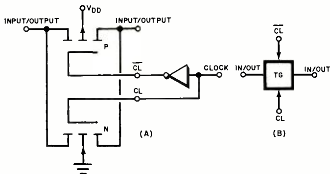
Fig. 4. A CMOS transmission gate (TG) has both pass transistors on or off together when driven by clock signals (A). The logic diagram is at (B).
