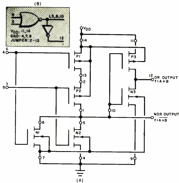
Fig. 2. A CD4007AE or CA3600E can be interconnected as shown to create NOR or OR logic (A). Symbol is at (B).
