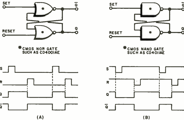
Fig. 5. Cross-coupled NOR gates respond to positive-going input signals (A) while cross-coupled NAND gates respond to negative-going.
