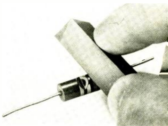
Fig. 4. The resistance of an ordinary carbon resistor can be trimmed by using a file.
