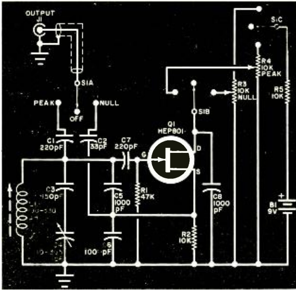
Fig. 1. The circuit is essentially a Colpitts oscillator which is adjusted by R3, R4.
