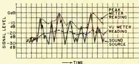
Fig. 1. Response of two meters to dynamic profile of typical music signal (solid line). The VU meter (dashed line) roughly indicates average level. Because of fast attack and slow release, the peak-reading meter (dotted line) follows contour of the peak levels.
