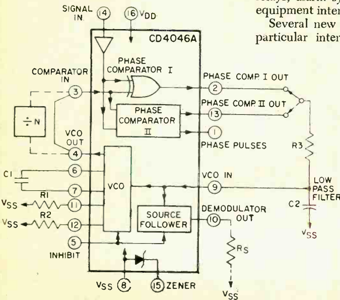
Fig. 3. Block diagram of RCA's new CD4046A COS/MOS micropower phase-locked loop IC device.
