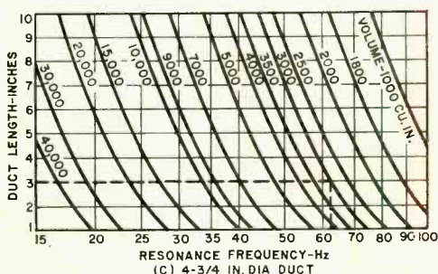
Fig. 4. Design charts for cardboard tube ducted enclosures developed by J. F. Novak, Chief Engineer, Jensen Sound Laboratories. Various tubing diameters are inside measurements; duct length is measured from cabinet front. Tubes can be obtained from business supply houses, stationery stores, or ordered from Service Manager, Jensen Sound Labs., 4310 Transworld Rd., Schiller Park, IL 60176.
