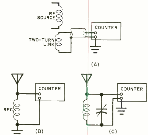
Using a counter in r-f measurements.
