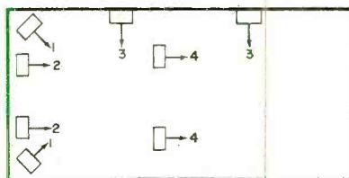
Fig. 1. Speaker placements at floor level. (1) Maximum bass, severest standing waves. (2) Excellent bass, moderate standing waves. (3) Moderate bass, and smoother response. (4) Has fairly thin bass, smooth response.
