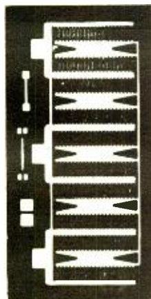
Fig. 17. At very high frequencies, power transistors take on some very complex geometries to prevent current crowding. Characteristics of structures are at right.
