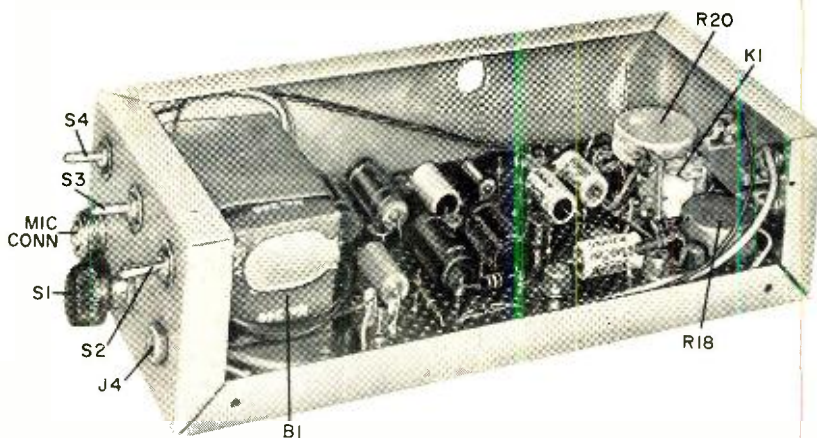
Photo shows layout of the prototype, though any type of chassis can be used.
