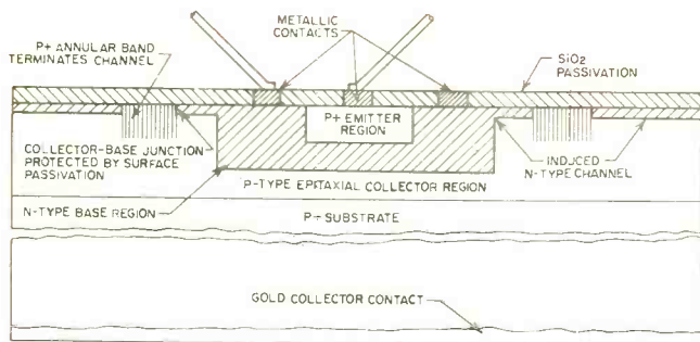
Fig. 15. Latest process is epitaxial planar with annular ring.
