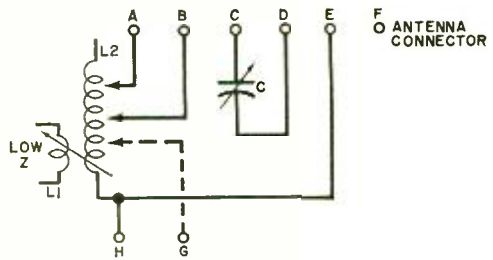
Fig. 8. A flexible type of antenna impedance matching circuit used with various antennas.
