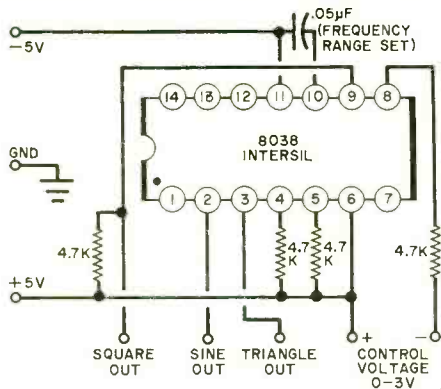
Fig. 2. The simple vco, above, offers sine, square, and triangle waveforms.
