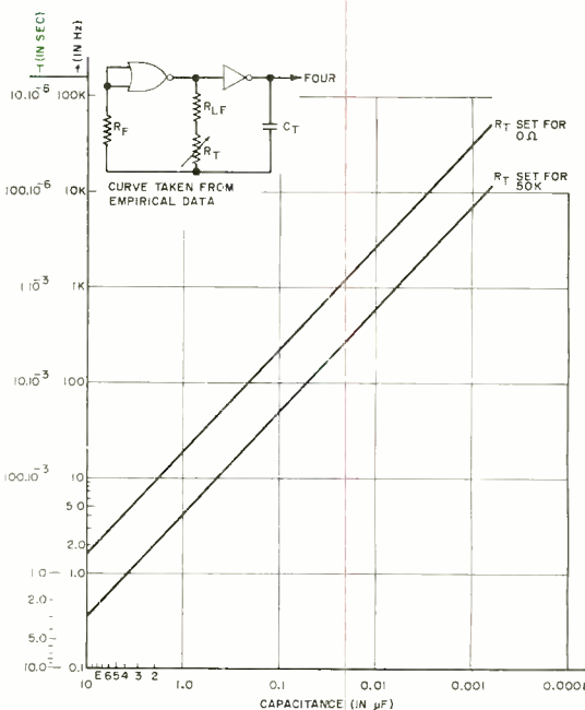
Fig. 1. Capacitance versus frequency or period to determine output of the oscillator.
