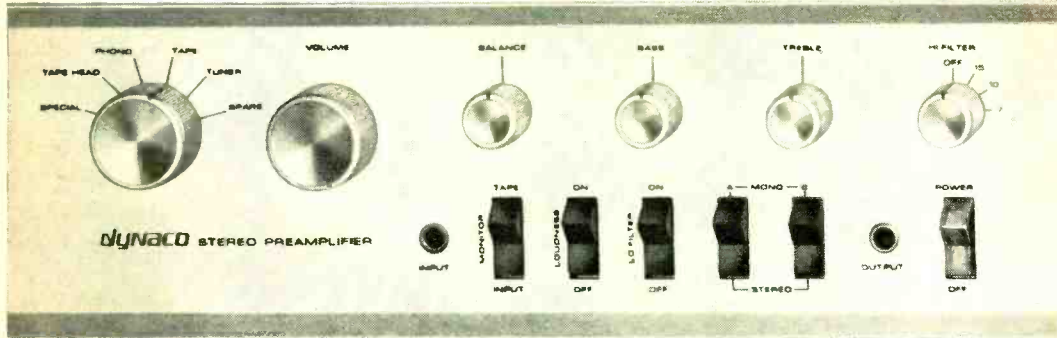
PAT-4 Preamplifier
