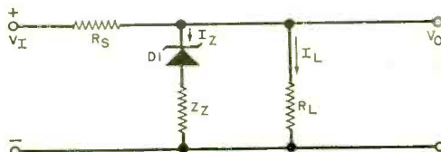
Fig. 5. Basic zener regulator circuit.
