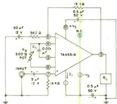
Fig. 4. Test circuit using TA8651A.
