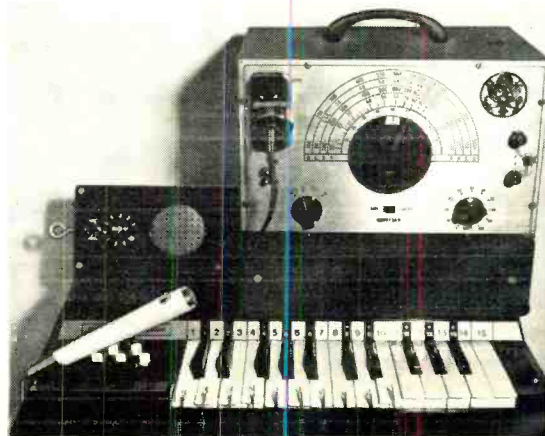
Fig. 5. Special effects setup for an electronic organ. Audio generator and keyboard at right; controls for cadence timer, mixer and mike at left.
