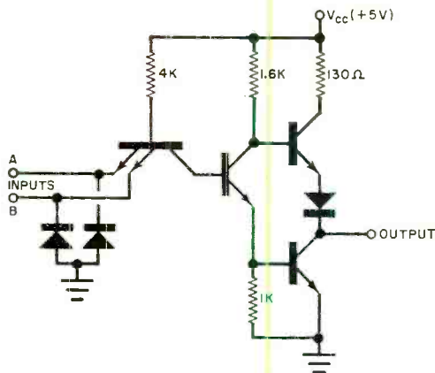
Fig. 1. Basic 7400 TTL gate circuit.
