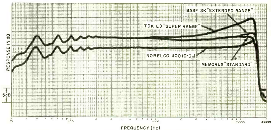
Typical frequency response curves of four distinctly different tapes.
