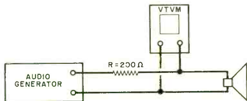
Fig. 3. Test setup for determining free air resonance using an audio generator.
