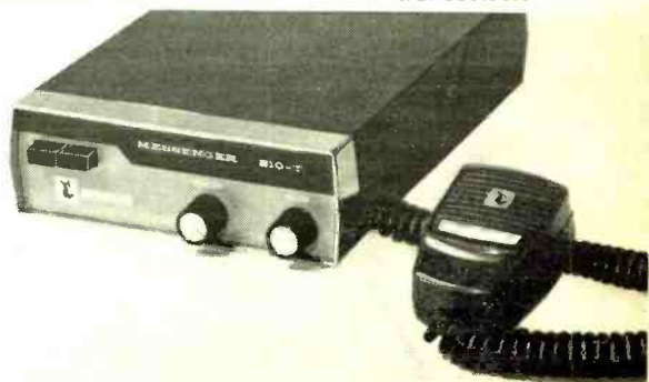
Johnson 210-T Business Radio transceiver.
