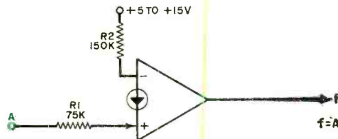
Fig. 16. Simple non-inverting buffer.
