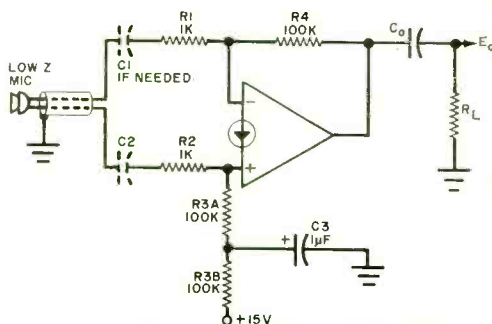
Fig. 6. Inverting amplifier using CDA.
