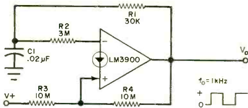
Fig. 10. Square wave generator using CDA.
