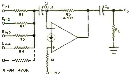
Fig. 4. Mixing amplifier using CDA.
