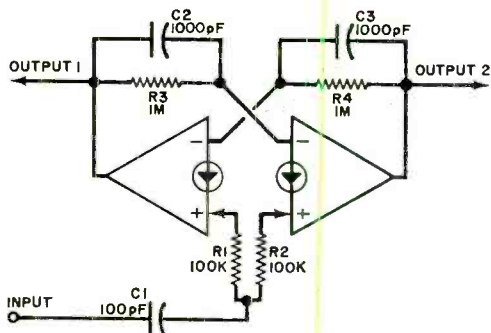
Fig. 15. Toggle flip-flop uses two CDA's.
