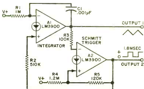
Fig. 11. A CDA triangle wave generator.
