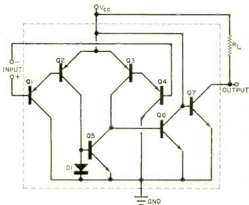
Fig. 2. One section of a quad comparator.
