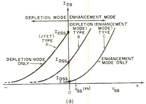
Fig. 3. (A) Static characteristics of type C FET; (B) transfer characteristics of 3 types.
