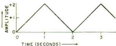
Fig. 4. Waveform of a triangle wave used to control output of amplifier.
