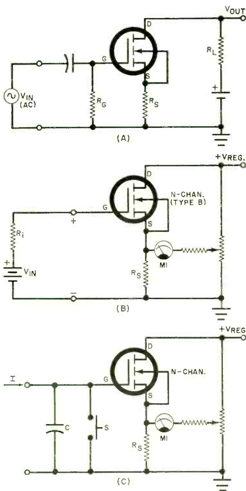
Fig. 4. Some typical MOSFET applications.
