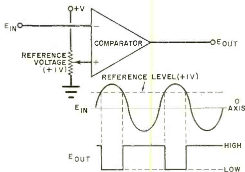
Fig. 1. Basic action of a comparator.
