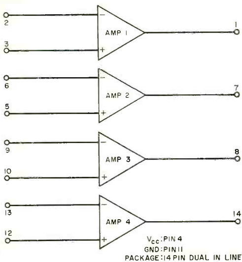
Fig. 3. Pin connections for op amps.
