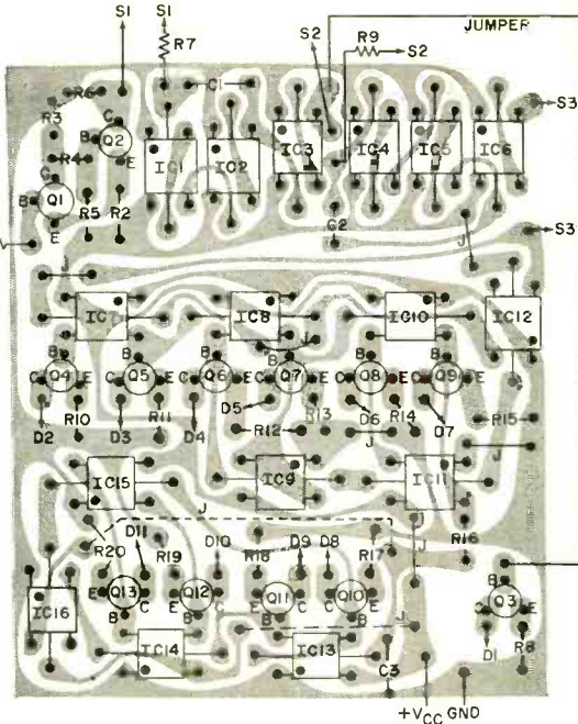
Fig. 2. Upper right are foil patterns. Component layouts above and at right.
