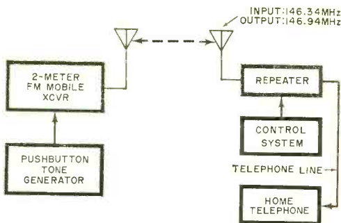
Fig. 3. Basic auto-patch communication system for the 2-meter amateur band.
