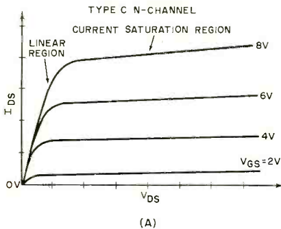
Fig. 3. (A) Static characteristics of type C FET; (B) transfer characteristics of 3 types.
