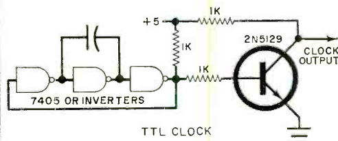
Two digital test circuits you can try.
