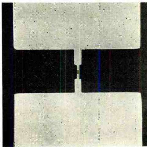
Small bounded oval at center of this photomicrograph is a Josephson junction, measuring 1.25 by 3 microns. Broad white areas are 50-ohm transmission lines connecting junction to the external time-measuring circuitry.
