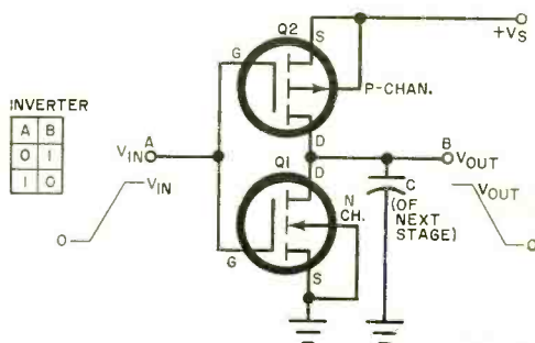
Fig. 5. Low-power complementary inverter.
