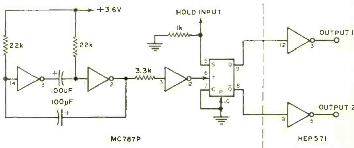
Fig. 2. Variation of circuit shown in Fig. 1 uses JK flip-flop as shaper and hold gate. Outputs are buffered.
