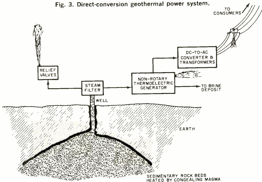
Fig. 3. Direct-conversion geothermal power system.
