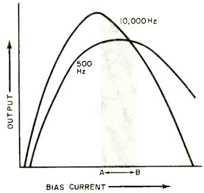
How bias current affects mid- and high-frequency signal output from a cassette tape. Note that, for the current range between A and B, 500-Hz output hardly varies at all, but 10-kHz output varies substantially.
