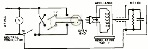
Circuit suggested by American National Standards to check leakage current.
