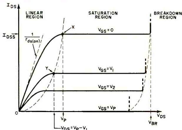
Fig. 2. Static characteristics of the JFET showing the linear, or triode, region and the saturation, or pentode, region of the vacuum tube.
