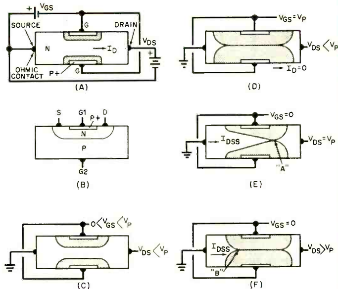
Fig. 1. A bar junction FET is shown at (A), a planar junction FET at (B). At (C), channel height is reduced by increase of depletion zone height. Channel is cut off (D) by merged depletion zones. At (E) is shown onset of saturation region with the drain voltage equal to pinch-off voltage. With high drain voltage, the saturation current remains constant in (F).
