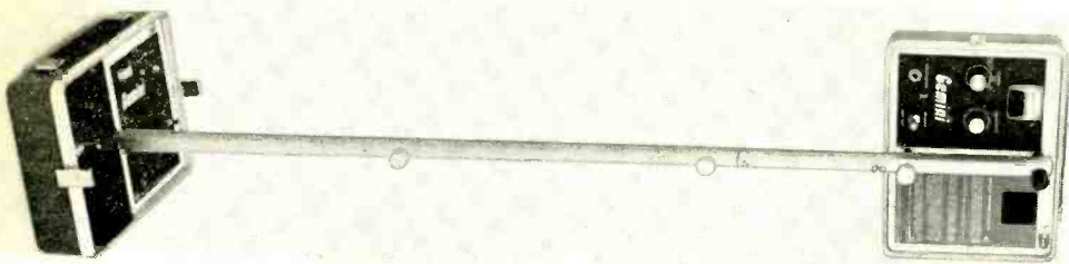
Fig. 4. Fischer's Gemini has a pulsed r-f transmitter and receiver at opposite ends.
