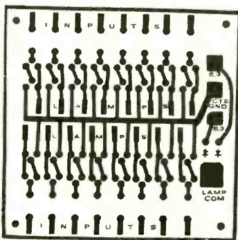
Fig. 2. Actual size foil pattern (above) and component installation (left) for a 16-terminal tester. If you need only 14 terminals, two end circuits are removed and two leads remain from 16-wire cable.
