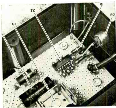
Fig. 2. Simplicity of circuit is responsible for easy layout of components on perforated board. Note that, since line voltages are exposed in several places in circuit, insulating Bakelite box should be used for the chassis enclosure.
