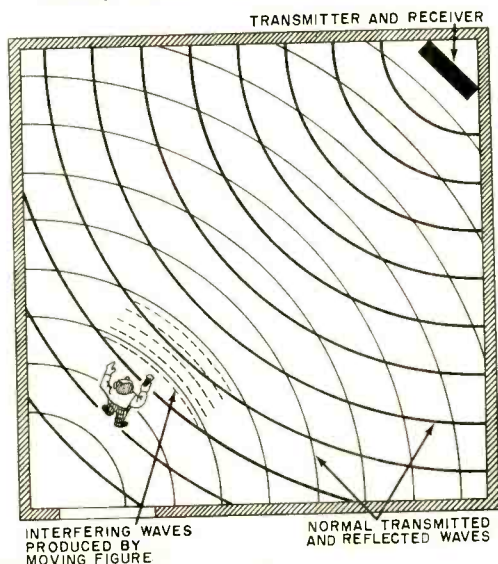
Fig. 3. Doppler effect systems detect moving objects from reflected waves.
