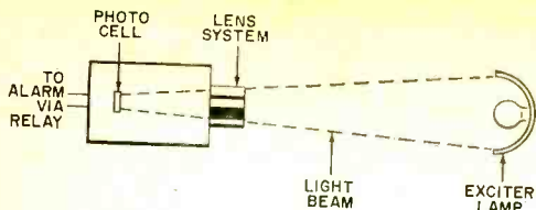
Fig. 2. Operation of photocell system.
