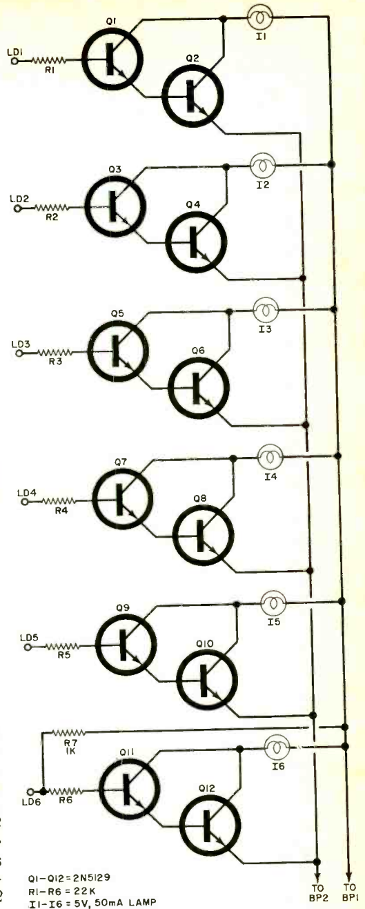
Fig. 3. Lamp drivers with high input impedance display the final result.
