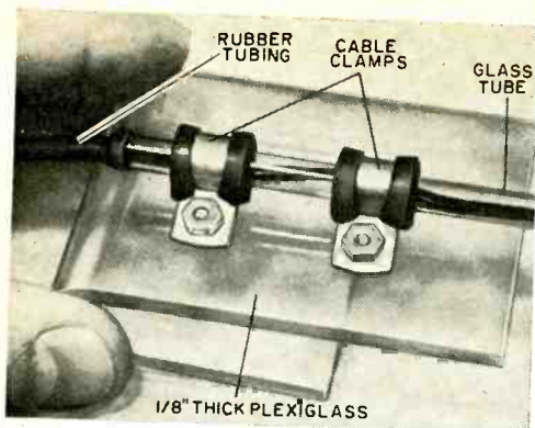
Fig. 3. Sensing probe assembly mounts on plastic bracket with cable clamps and #6 hardware. Do not overtighten clamps or the glass tube will break.
