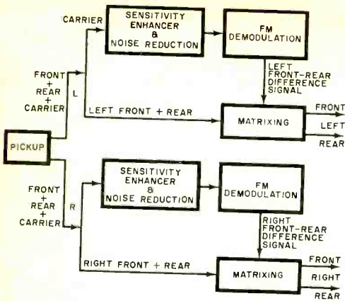
Fig. 2. Diagram of CD4 playback system.
