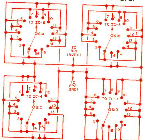
Fig. 1. Wire S1 as shown here with connections to the IC, BP1 and BP2.
