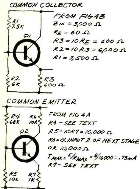
Fig. 6. Determine the resistor values.
