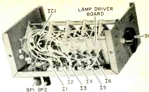
The computer is simple to build when wired in sections as in Figs. 1 to 4.
