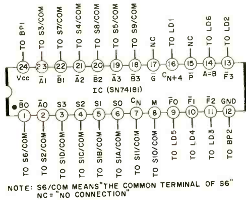
Fig. 2. Top view of connections to the IC. It is best to use a socket.
