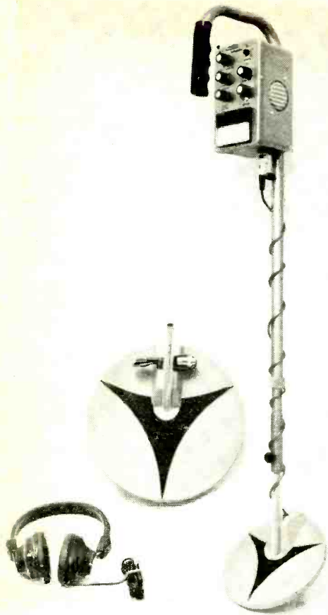
Fig. 3. Compass Electronics Yukon units.
