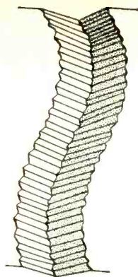
Fig. 1. Audio signal (large undulation) and ultrasonic carrier (small undulations) in a single disc groove.
