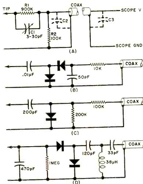
Fig. 1. Circuits of various probe types.
