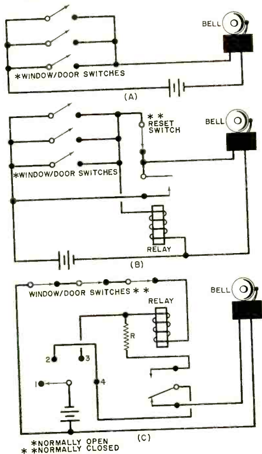
Fig. 1. Basic electric alarm systems.
