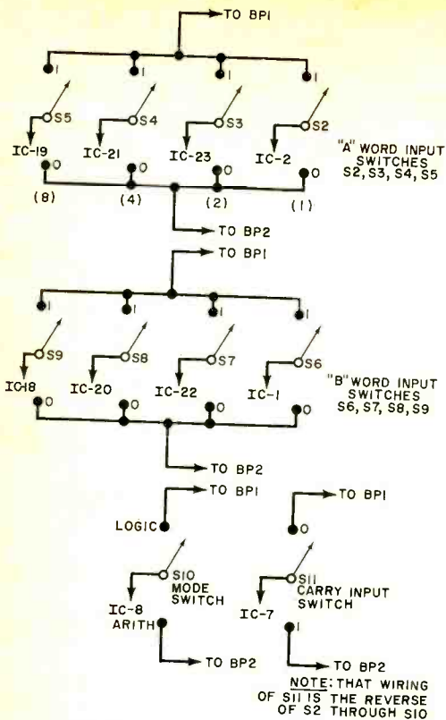
Fig. 4. Wiring of mode of operation switches and those for word inputs.
