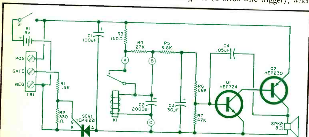
Fig. 1. The siren-like wail is produced by the changing voltage on capacitor C3, which is controlled by the operation of K1. Operation of SCR1 turns on the system.
