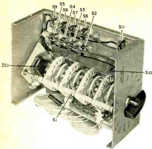
This shows how the prototype was assembled. Note mounting of IC board.
