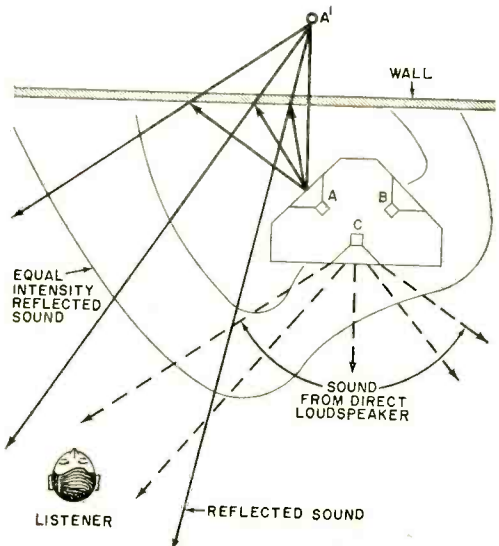
Fig. 5. This diagram shows how the direct-reflecting loudspeaker works.
