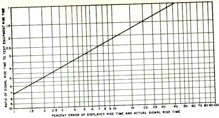
Fig. 2. Measurement error is inversely proportional to the rise-time ratio.
