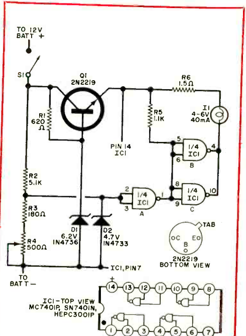
Fig. 1. When level at R2/R3 drops below 1.7 volts, warning light goes on.
