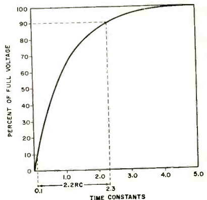
Fig. 3. This is time constant curve for charging capacitor in series RC circuit.
