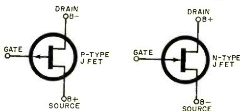
Fig. 2. Shown here are the schematic symbols for a p-type (left) and an n-type junction field-effect transistor.
