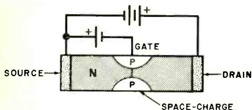
Fig. 1. FET acts as variable resistor in which the gate field has a direct effect on source-to-drain current flow.
