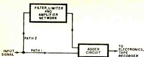
Fig. 1. Input to Dolby network for a tape recorder goes through two paths, one being the special filter network.
