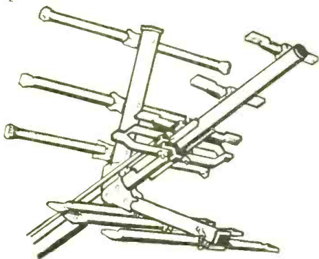
Fig. 1. Winegard uhf section fits in front of other companies' vhf units.
