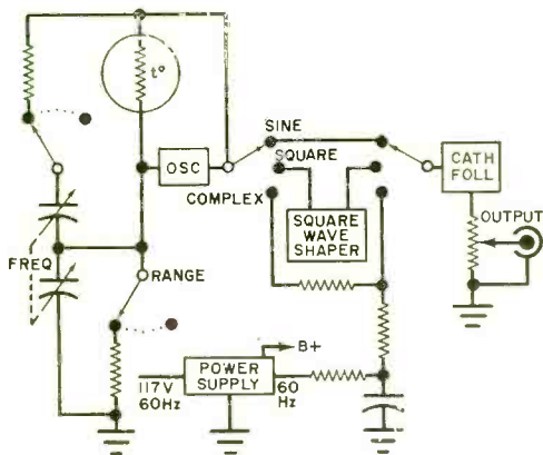
Feedback thermistor maintains good amplitude stability and reduces distortion.
