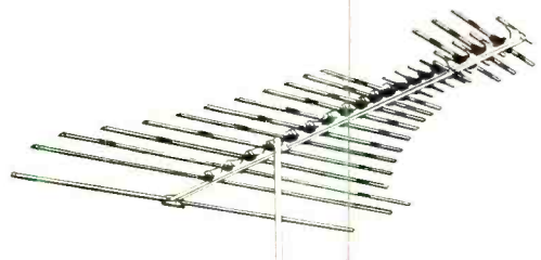
Fig. 4. Element lengths follow exponential formula in GC Audiotex design.
