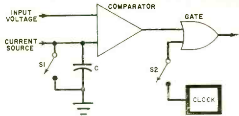
Fig. 1. Elementary capacitor-discharge analog-to-digital converter is typical of those used in digital instruments.
