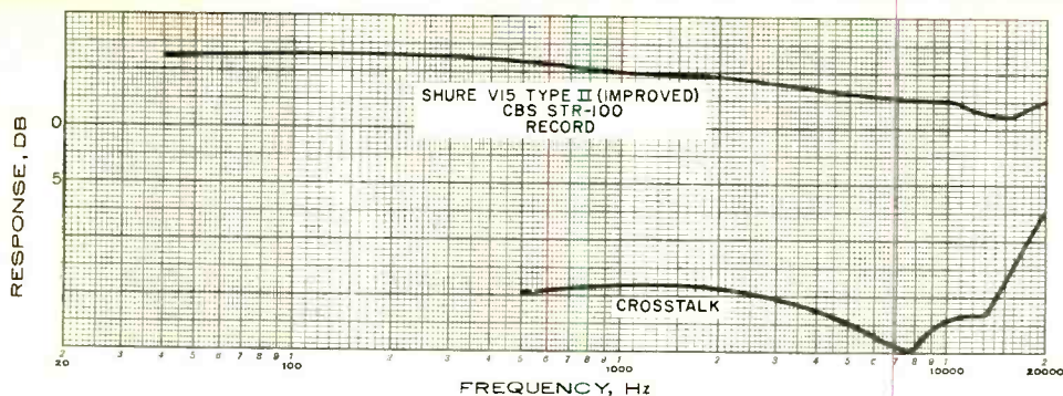
Frequency response and crosstalk curves for Shure V15 Type II (Improved) phono cartridge were obtained using CBS STR-100 record.
