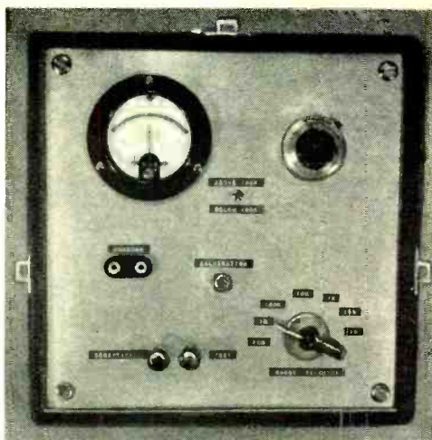
Although the prototype was built in a wood case, any type of construction may be used. Note the 10-turn dial.
