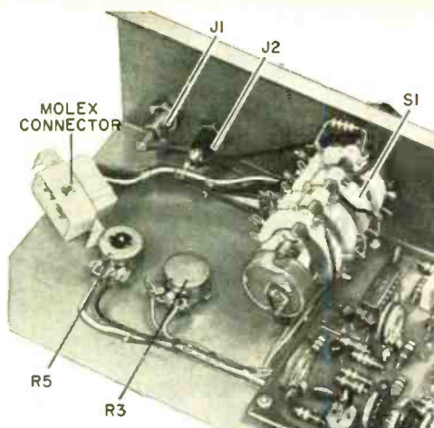
Fig. 6. Photo shows parts mounting details for off-board components.
