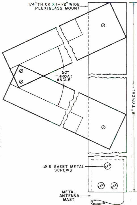
Fig. 3. Use non-metallic mount (Plexiglass or fiberglass) to fasten antenna to mast. Do not substitute metal for mount or mount antenna directly to mast.
