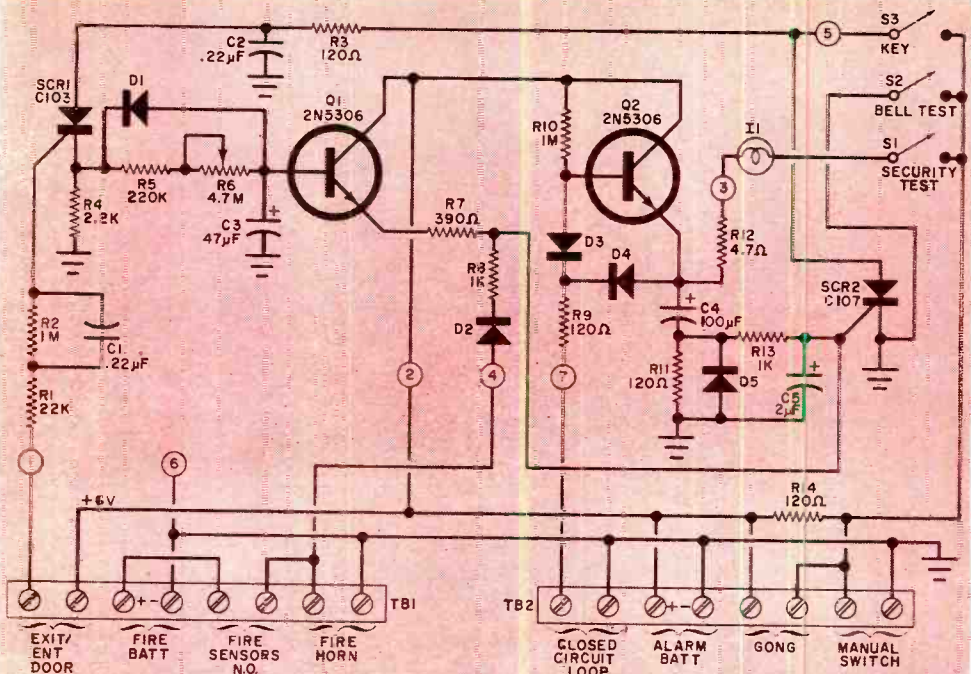
Fig. 1. Unlike other alarms, this one features a 5- to 50-second delay to allow legitimate entry without ringing the gong. This same circuit is also used for fire warning when used with the appropriate sensors.
