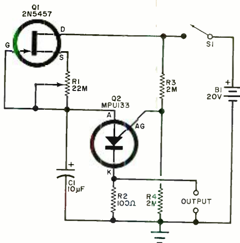
Fig. 2. Using a PUT and a FET, you can make a timer delivering an output pulse of a few seconds to 20 minutes.
