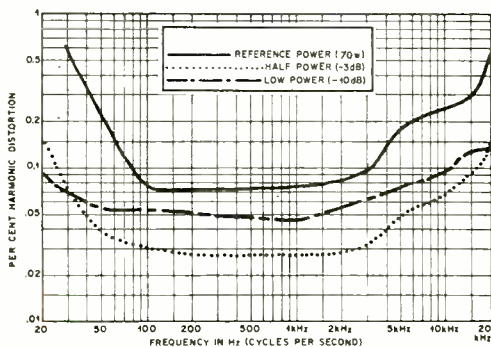
Graphs show harmonic distortion and THD (below left and right), and frequency response and crosstalk (bottom) for Pioneer's SX-2500 receiver.
