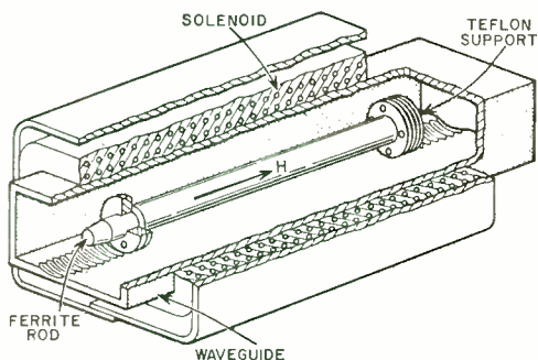
Phase shifter consists of a ferrite rod in waveguide. (Courtesy of Bell Laboratories)
