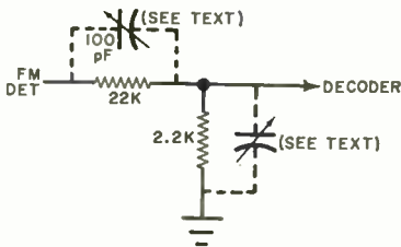
Fig. 4. This compensation network added to the FM detector output can greatly improve the results.
