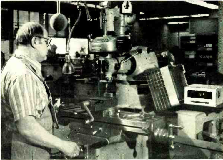
Fig. 3. Milling machine operation is monitored by General Radio 1934 noise exposure meter. Mike is in windscreen right of operator's head.
