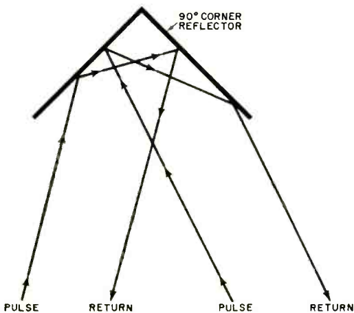
Fig. 6. Theory of the corner reflector that illustrates how this device returns the radar beam along same path on which it came.
