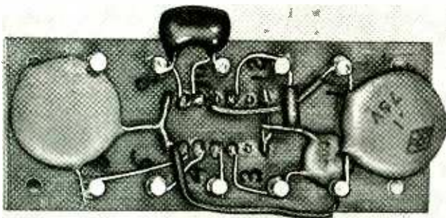
Fig. 3. If you mount a dual-in-line socket on the breadboard, it can be used for both in-line and round IC's.
