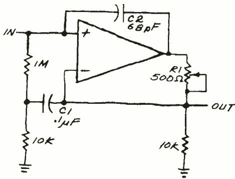
Fig. 7. This circuit, developed by NASA, has an input impedance of several hundred megohms with an input capacitance of less than 1 pF.
