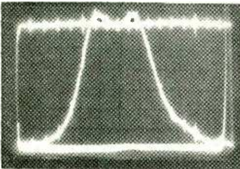
Channel 3 circuit without traps showing the channel 2 aural and channel 4 visual markers down the skirt. Although they are far down the skirt, such carriers cause interference.
