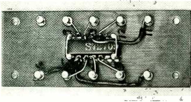
Fig. 2. This simple breadboard approach may be used to connect up an op amp. The layout below shows a circuit fully wired.
