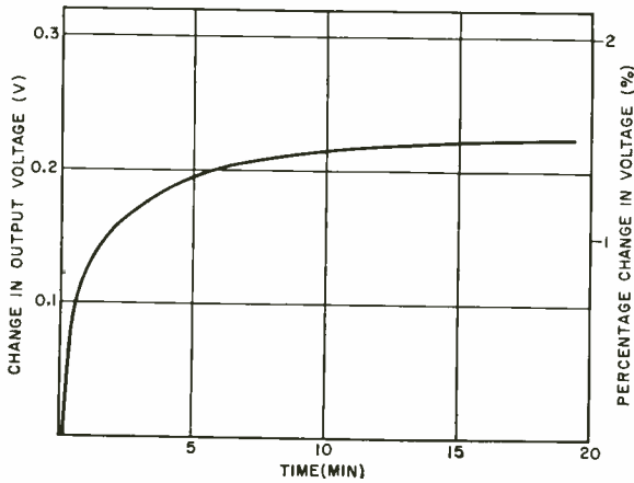
Fig. 2. A typical chart of variation of the output of a homemade power supply over 20-min period.
