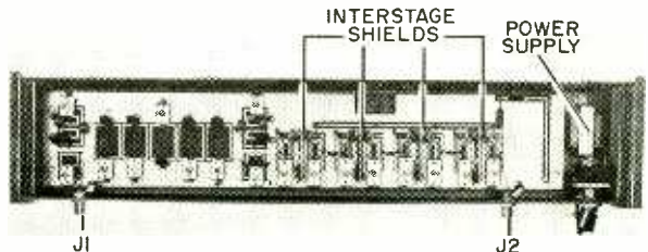
Fig. 10. Overall view of the high-band board showing the shields.
