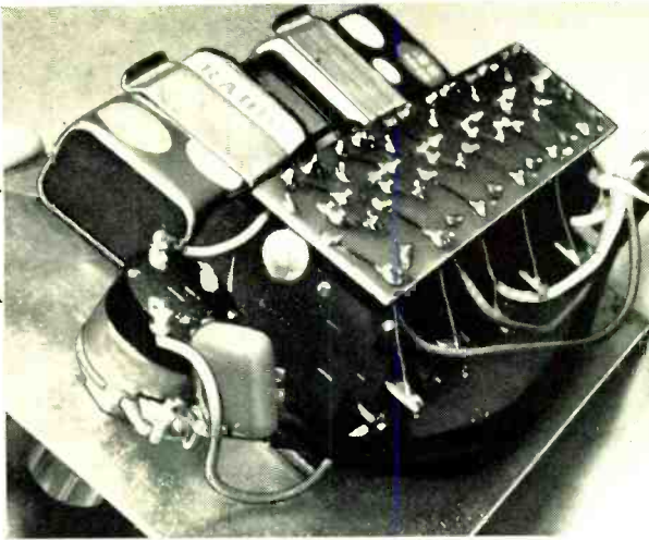
Fig. 7. Six normally open pushbutton switches are connected as shown here, one feeding each tone generator. Dc voltage comes from the same battery that powers the tone generator board.
