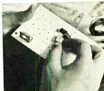
Assembling integrated circuit on a printed circuit board —Circuit is identical to one used in latest IBM System 360 computers. Student is constructing an oscillator combined with a Darlington pair output amplifier.
