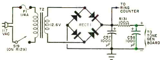
Fig. 4. The power supply, which is chassis mounted, provides a smoother dc to the tone generator than to the pulse counter.
