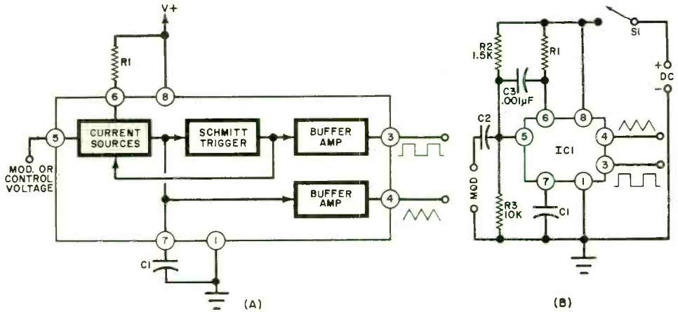
Fig. 5. This new VCO IC can deliver triangle or square wave outputs from 1 Hz to 1 MHz. Frequency is determined by R1 and C1, with modulation applied via pin 5.
