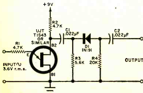
The short positive-going spike from the base-2 terminal of the UJT is eliminated by D1-R4 combination.
