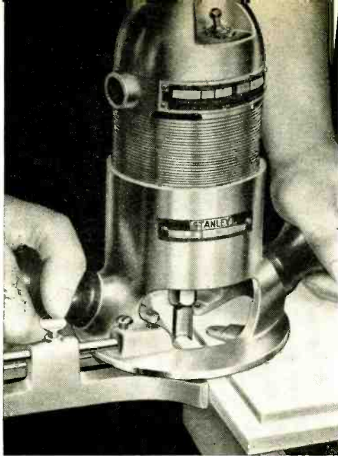
Photo shows the router guide set up for rabbeting to make the tongues. (Photo courtesy of Stanley Works)
