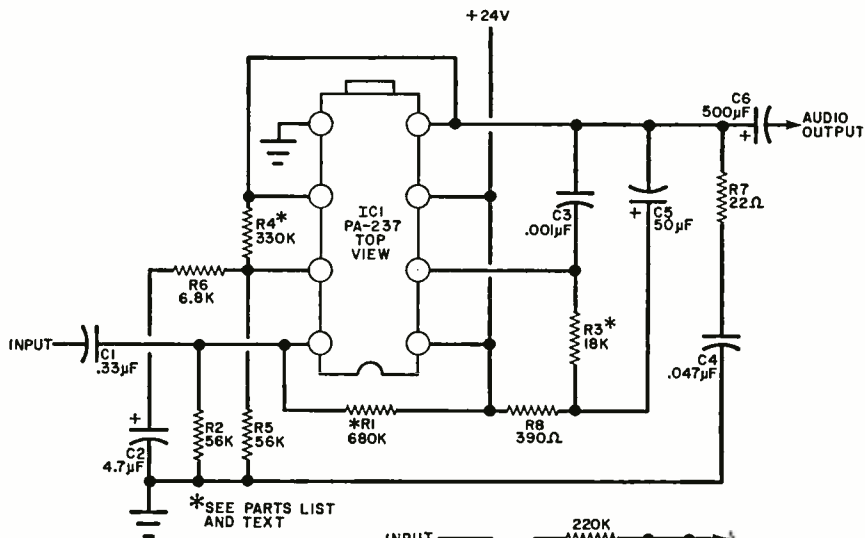
Fig. 1. The IC is a seven-transistor power amplifier requiring 8mV to deliver 2 watts audio control. Tone and volume control circuits at right.
