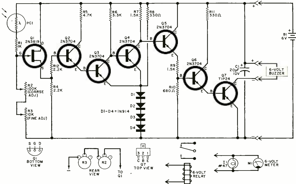
Fig. 1. No power is applied to output indicator until PC1 "sees" a predetermined level of infrared.
