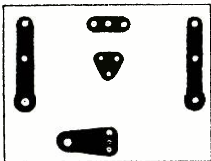
Fig. 5. Actual-size foil pattern for the twin-T PC board. A separate board is used so that, if it is desired to change frequency, you merely remove three screws and insert a new twin-T filter PC board.
