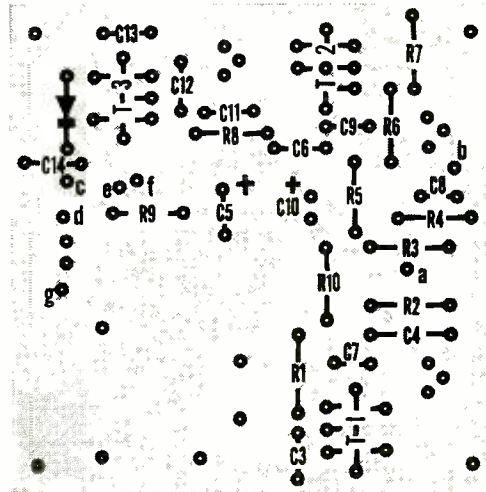
Fig. 3. Transistors are located on circuit board as follows: Q1—to right of R6; Q2—directly above C4; Q3—directly above C11. When mounting transistors, match widely-spaced leads to widely spaced holes in board.
