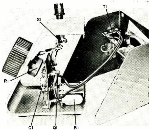
The entire electronic thermometer is contained within a small cabinet. The circuit is not critical, so any other mechanical arrangement can be used. If you wish to measure outside temperature, mount the thermistor out of a window in a weather-protected spot, and connect it to the thermometer via a twisted pair. This pair can enter the cabinet through a rubber grommet.
