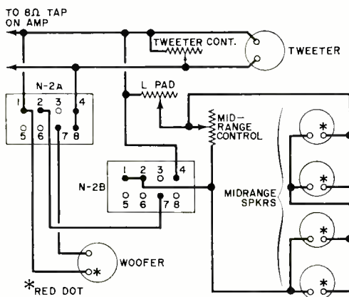
Fig. 2. To obtain proper phasing, be sure to wire all speakers together as shown here. Terminal numbers are stamped right on crossover networks.
