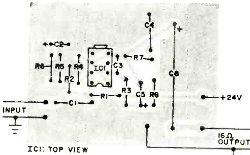
Fig. 3. Install the components as shown here. If you don't have a 16-ohm speaker, use two 8-ohm units in series. Be sure they are phased right.
