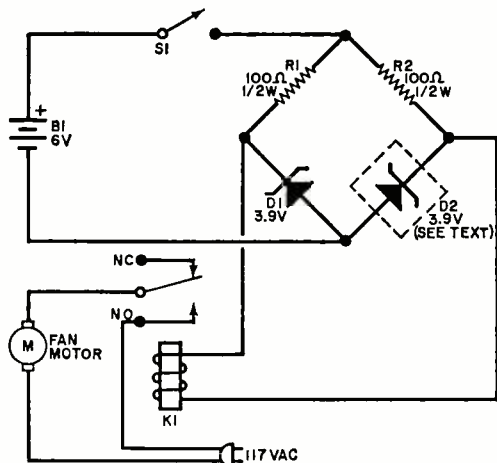
Fig. 1. Zener diode, D2, in electronic equipment, senses heat, unbalances bridge and turns on fan.
