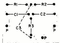
Fig. 6. Capacitor C_3 is mounted on the foil side of the twin-T PC board. The three holes marked "P" mate with similar holes on the main circuit board.
