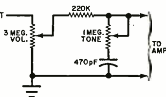
Fig. 1. The IC is a seven-transistor power amplifier requiring 8mV to deliver 2 watts audio control. Tone and volume control circuits at right.
