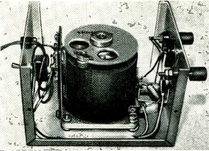
Note how the Variac is mounted in the center of the enclosure with input components on one end, output on the other. This is bottom view of chassis.
