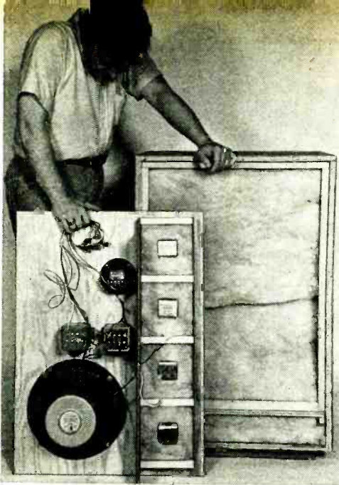
Fig. 3. For proper damping, loosely folded fiberglass wool should fill entire enclosure volume.
