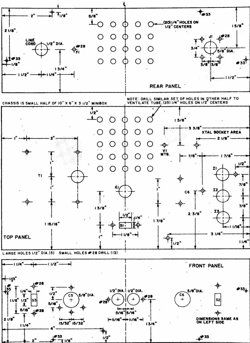
Fig. 2. Drilling specifications for the chassis. The three photos on the opposite page show the various holes and the location of all parts. Don't forget to drill 25 holes in the other half of the chassis, directly opposite the holes on the top panel. Crystal socket holes are drilled as required.
