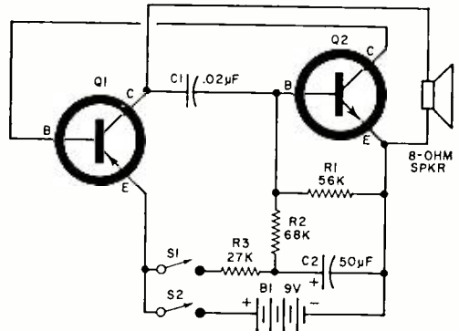
Fig. 1. In John Ramsey's siren, S1 is a push-button type switch. This circuit makes an ideal electronic substitute for those bicycle-wheel-operated sirens.
