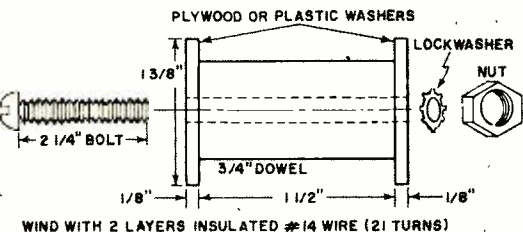
Fig. 3. Construction details for "hash" coil L1. Close-wind 21 turns of #14 insulated wire in two layers. The bolt secures the coil to the chassis.
