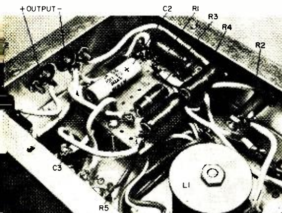
The output end of the "Up-Verter" chassis. Note location of the circuit board and the remainder of the components not visible in the other photos.
