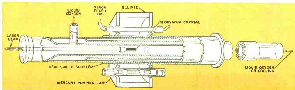
Continuous wave crystal lasers use configurations somewhat like this Bell telephone design. The neodymium crystal is at one focus of an elliptical cavity, and the mercury lamp at the other to concentrate pumping light.
