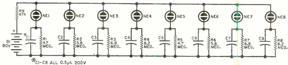
The neon lamps can be arranged in any pattern desired—circle, square, etc.
