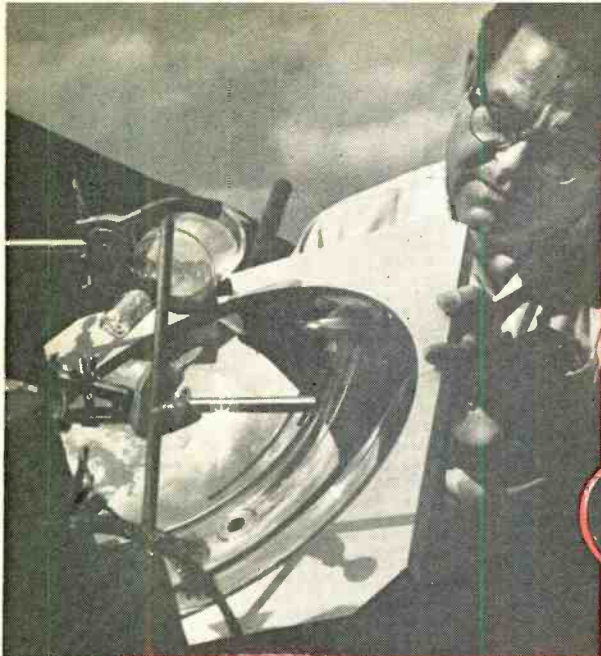
Sunlight pumping of a solid-state laser is a new development which may soon make it possible to put sun-powered lasers aboard satellites for communications, tracking, and geodetic measurements. This device, designed by RCA, uses a 12" hemispherical mirror to focus sun on calcium fluoride crystal rod.
