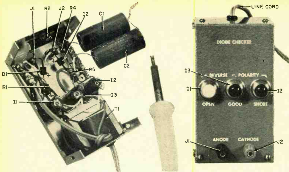
Photographs of diode checker's interior and front panel reveal construction details. Capacitors C1 and C2 (see photo at left) have been partially disconnected and moved aside for a better view.
