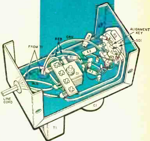
Photograph of power supply's exterior (top) and pictorial diagram of interior (above) show all essential construction details.
