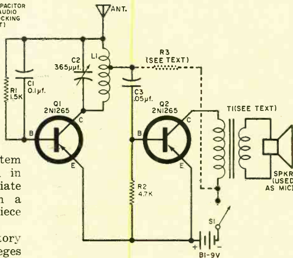
Fig. 6. Wireless microphone circuit submitted by reader Earl Campbell, Jr., WPE8DVK.
