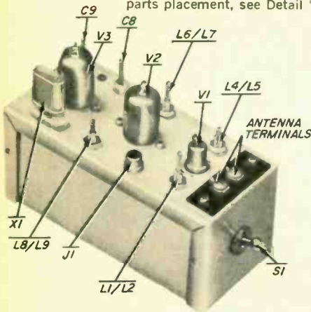
Top view of converter. For exact parts placement, see Detail "B."
