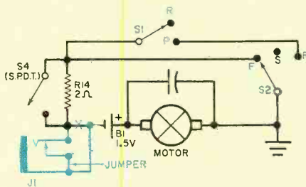
Fig. 4. Subminiature jack J1 permits remote control with a hand- or a foot-switch.
