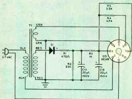
Schematic diagram of the power supply, which utilizes a simple half-wave diode rectifier.
