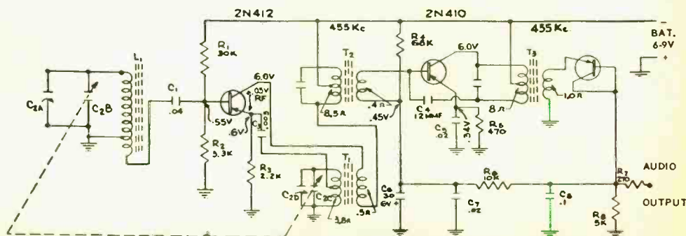
Fig. 4. Schematic diagram of the KB-138 AM tuner. Although the circuit employs three transistors, the one at transformer T3 's output is actually diode-connected.
