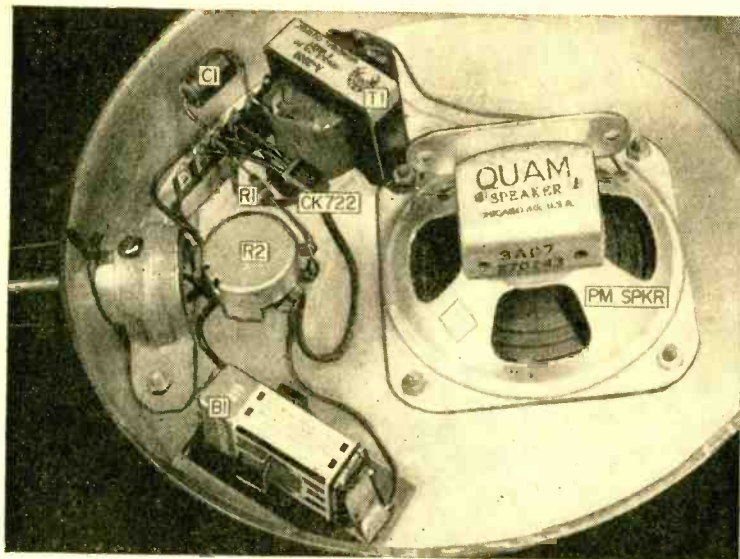
Interior view of banjo with various components identified and their relative positions indicated. The chassis is an aluminum cake pan, which contains all components except the on-off switch S1.
