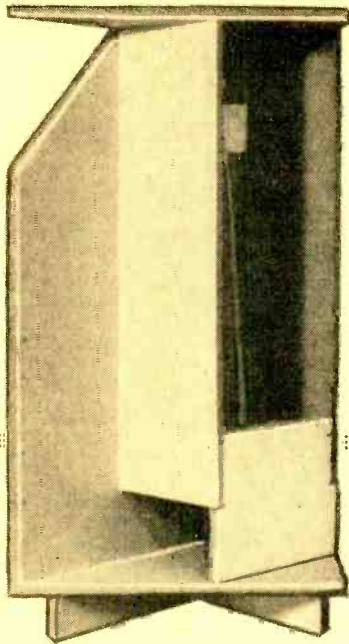
Rear view of enclosure shows placement of the various Celotex sections.
