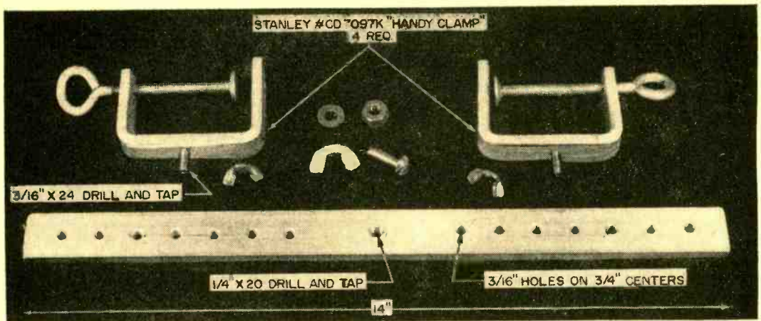
Fig. 3. Basic layout for making a single rocker arm including all necessary parts.
