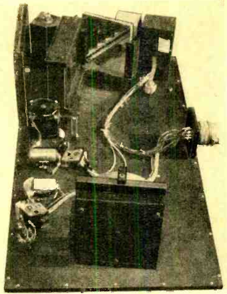
Inside view of receiver. Amplifiers and converter are mounted directly beneath.
