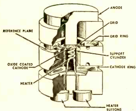
G-E MICRO-MINIATURE CERAMIC TUBE, TYPE 6BY4
