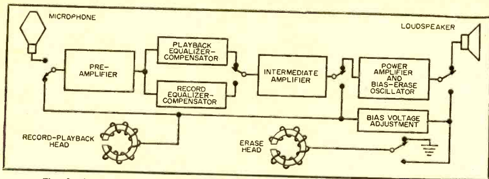
Fig. 2. Single-chassis switching is illustrated in this block diagram of a complete tape recorder. All switches are shown in playback position. Many recorders use separate circuits for power amplifier and bias-erase oscillator. For simplicity of explanation, however, the unit shown here combines these two functions in one stage.
