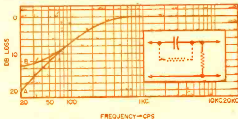
Fig. 3. A high-frequency boost can be produced from a low-frequency roll-off. Shown by curve "A" is the response when a series capacitor is inserted in a circuit without the shunt resistor. Curve "B" illustrates the response when the capacitor is shunted by a medium value resistor.
