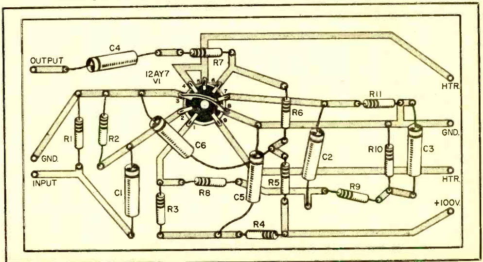
Fig. 4. This pictorial diagram shows the exact size of the mounting board, and may be used as a guide line diagram. Components are not drawn to scale.
