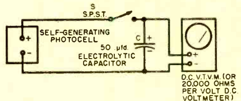
Fig. 4. Charging a capacitor.
