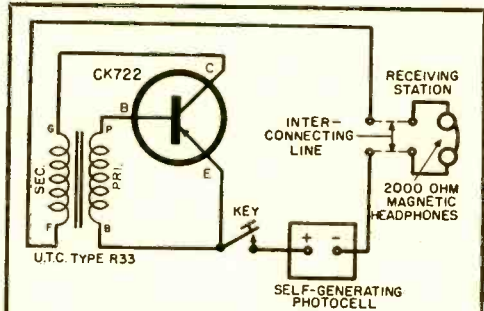
Fig. 6. Transistors enable solar batteries to be used where the voltage demands are very small. This circuit is that of the audio tone generator which is pictured on page 66. Experimenters can also use it as a code practice oscillator. Frequency of tone from the oscillator will vary according to the amount of light on self-generating photocell.
