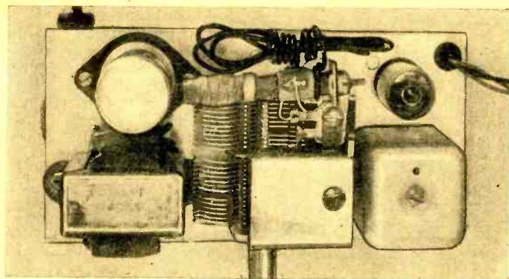
Fig. 2. Above-chassis view shows location of the major components. Note shield over one section of the tuning capacitor, and the three-wire cable to the speaker (right).
