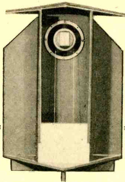
Placement of speaker is obvious from this rear view of the labyrinth baffle.
