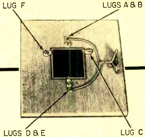
Fig. 1. Mounting of the B15 photocell on a small wooden board. Do not solder directly to the photocell. Use the scheme shown above to contact the surfaces of the cell with small soldering lugs. See text for more details.
