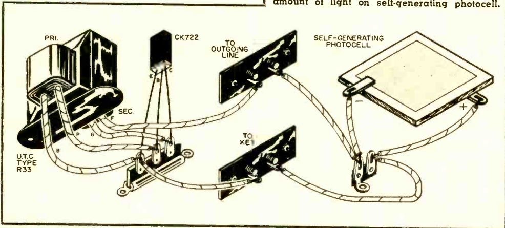
Fig. 6. Transistors enable solar batteries to be used where the voltage demands are very small. This circuit is that of the audio tone generator which is pictured on page 66. Experimenters can also use it as a code practice oscillator. Frequency of tone from the oscillator will vary according to the amount of light on self-generating photocell.
