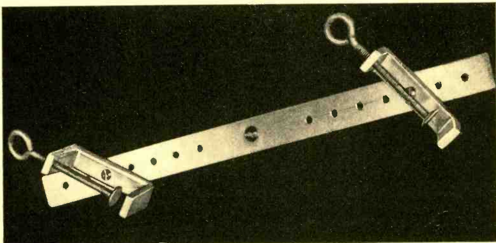
Fig. 4. Completely assembled rocker arm, two of which are required to hold chassis.
