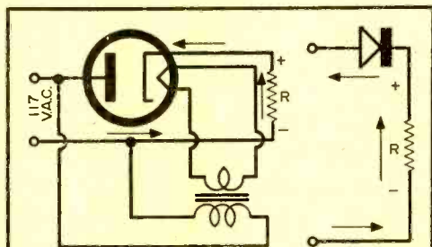
Fig. 1. Schematic of vacuum-tube rectifier (left) and crystal rectifier (right).
