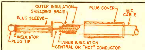
Fig. 1. Sectional view of microphone plug and cable with cover slipped back. Note the cable shield is also ground return conductor. Breakage of cable at this point is often a cause of recorder failure. Hum and noise can be generated by a bad connection. Some microphones use regular phono plug which is inherently smaller and weaker.
