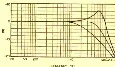
Fig. 9. High-frequency roll-off response curves resulting from different values used in the circuit diagrammed in Fig. 7(B).
