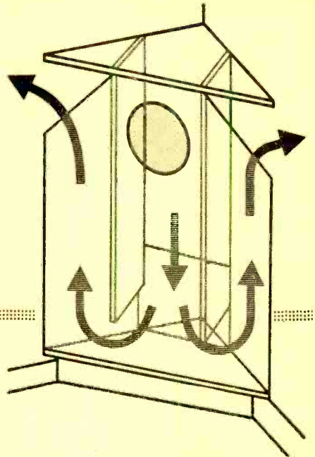
Phantom view of the enclosure shows sound paths from rear of the speaker.
