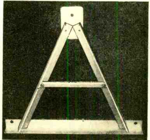
Fig. 2. Assembled A-frame using the pieces shown on the facing page. Two are required.
