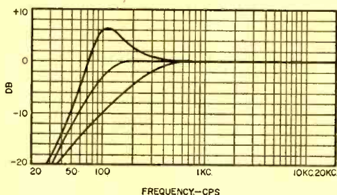
Fig. 8. This variety of responses may be obtained through the use of different component values in circuit shown in Fig. 7(A).
