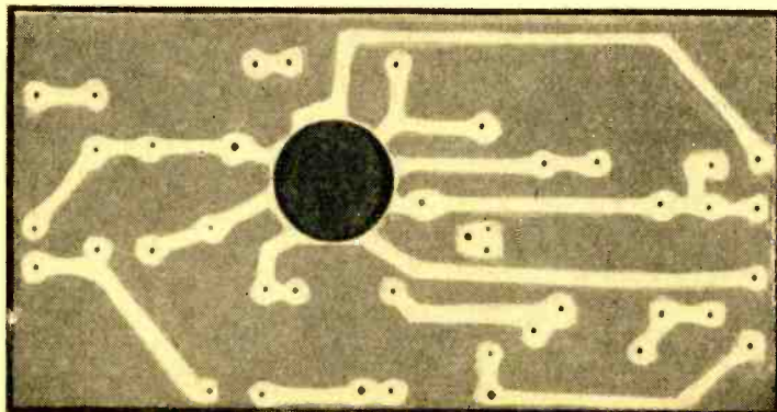
Fig. 2. The etched board, drilled and cleaned, and ready for mounting socket and component parts. Mounting holes for the electrolytic capacitors may have to be enlarged somewhat.
