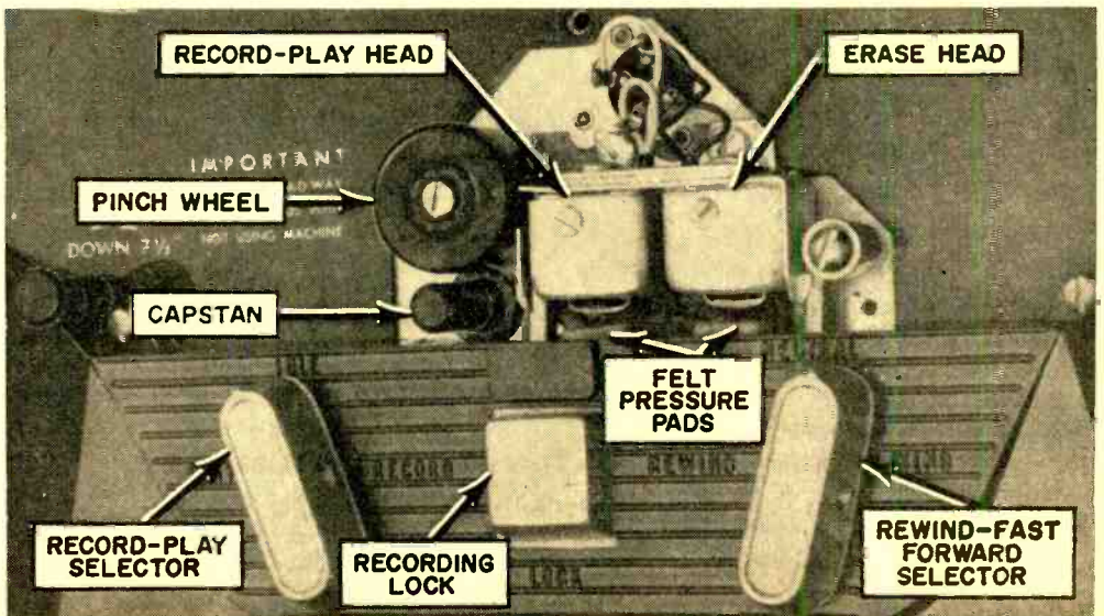
Fig. 2. Close-up view of recorder panel with dust cover over heads and tape drive removed. While various makes of units may differ in style and layout, the Pentron Model 225 illustrated here is a good example of the mechanical arrangement. The tape is pulled past the heads by the friction resulting from the pinch wheel forcing the tape against the motor-driven capstan. The pressure pads, shown here disengaged, press the tape firmly against the heads.
