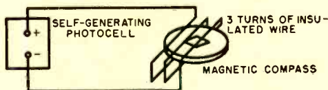
Fig. 3. Compass deflection.
