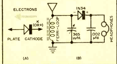
Fig. 2. (A) Schematic representation of crystal. (B) Complete crystal receiver.
