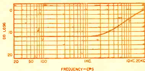
Fig. 4. Using a smaller value of capacitor in circuit of Fig. 3 will shift curve "B" and produce a good high-frequency boost.
