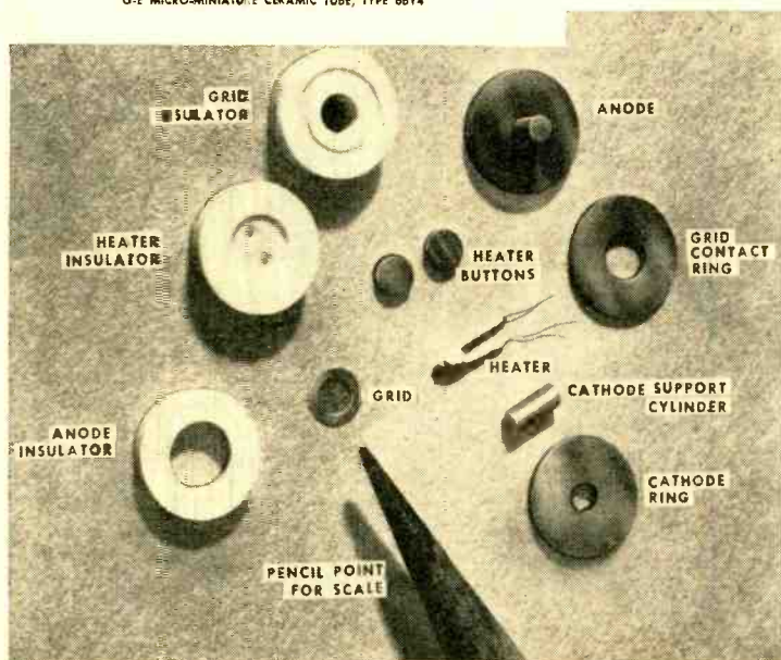
G-E MICRO-MINIATURE CERAMIC TUBE, TYPE 6BY4
