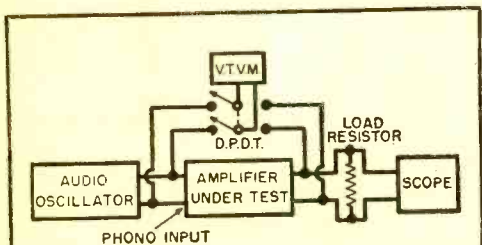
Fig. 1. This is the test arrangement for measuring the power output of a hi-fi amplifier. The vacuum-tube voltmeter must be sensitive enough to read the extremely small voltage input to the amplifier as specified by the manufacturer, which may be only a few millivolts. Output wattage is equal to the square of the voltage as measured by the v.t.v.m. divided by the value of the resistance of the load resistor; this resistor is a substitution for the speaker. The oscilloscope is not required for actual wattage measurements, but enables the sine-wave pattern to be checked for distortion. Power output is measured at various frequencies over the response range of the amplifier. See text for details.
