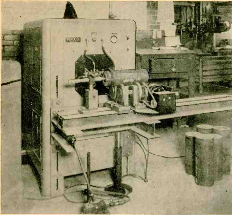
This Tocco heating station with inductor and fixture is used for brazing hydraulic cylinders and cylinder cap assemblies.
