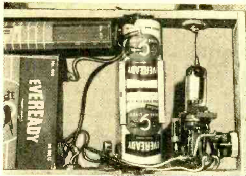
Inside of the transmitter showing the parts layout. The antenna is a side-mounted automobile-type, on the side.
