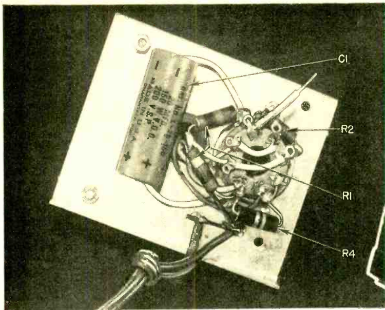
(Left) Subchassis viewed from underneath with the majority of components in place. (Below) Plug with wire soldered to one prong, forming a polarized plug.
