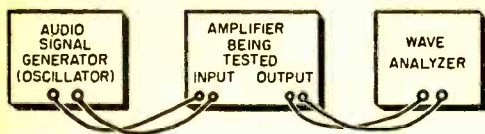
Fig. 2. Setup for using an audio signal generator with a wave analyzer for measuring certain kinds of amplifier distortion.
