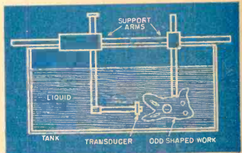
Fig. 4. Pulses of ultrasonic energy are reflected by flaws and displayed on a cathode-ray tube. Fig. 5. (below) Illustration of a method for examining odd-shaped metallic pieces for flaws using ultrasonic waves.
