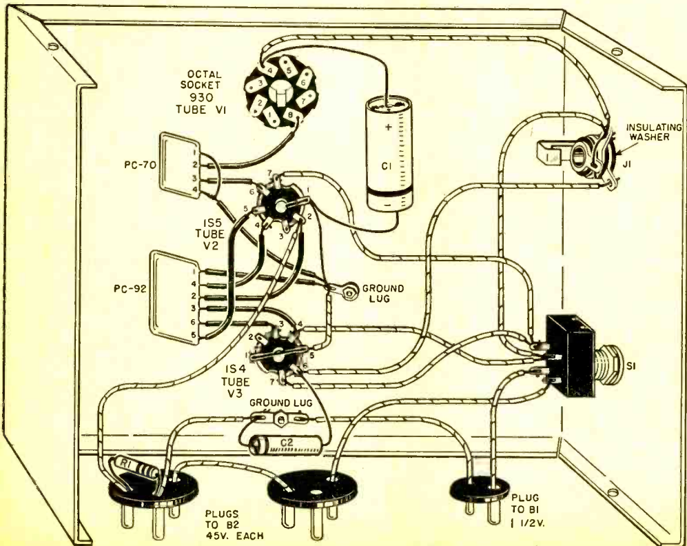
Pictorial wiring diagram of the light-beam receiving unit. Constructors unable to obtain the cheap printed circuit may substitute regular resistors and capacitors with the values shown on page 43.
