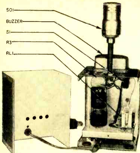
Rear view of control unit with cover removed. Note the subchassis on which the tube and relay are mounted. Holes in back and top are for ventilation.
