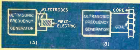
Fig. 1. Two basic transducer designs are shown above. Drawing (A) has a crystal element and drawing (B) a magnetostrictive core. Actual element movement in both cases is extremely small. Fig. 2. (below) shows a simplified block diagram of industrial ultrasonic equipment.
