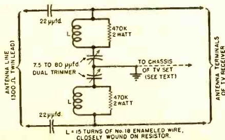
Fig. 4. (Below right) Filter may be tuned as shown schematically in Fig. 5. The text describes how this may be accomplished and why it is necessary when using certain TV receivers.
