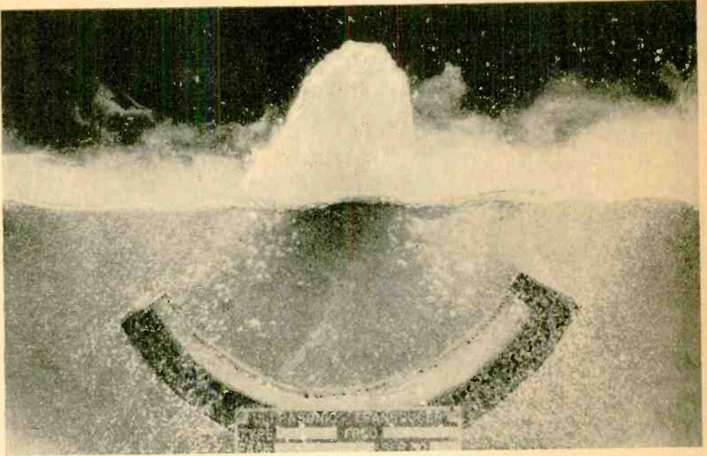
This photo shows the violent agitation of a liquid excited by the curved ultrasonic transducer immersed in the solution.
