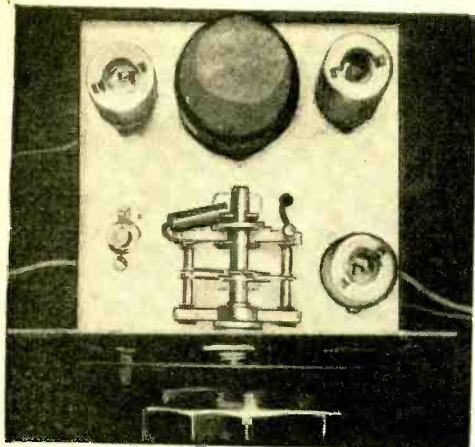
Top (left) and bottom (above) views of chassis, showing location of components.
