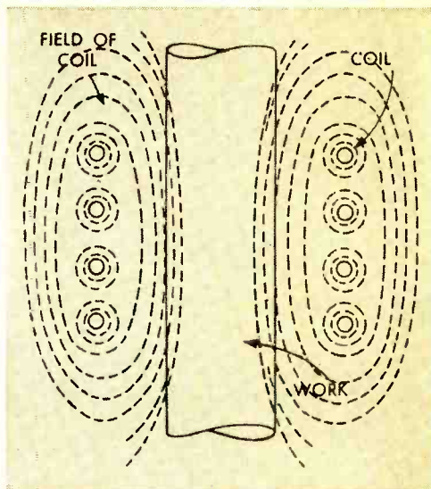
The effect of the electromagnetic field produced by loading the coil is shown above.
