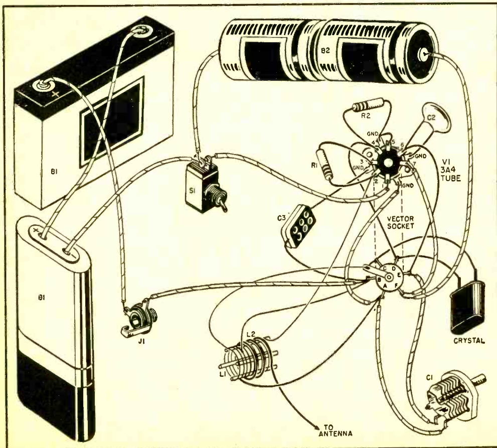
Pictorial diagram of the miniature transmitter described in this article.
