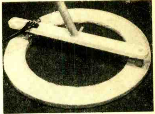
Completely assembled loop, ready for operation. Note terminal strip for connecting the shielded "Twinax" cable, the other end of which connects to a 3-prong plug.
