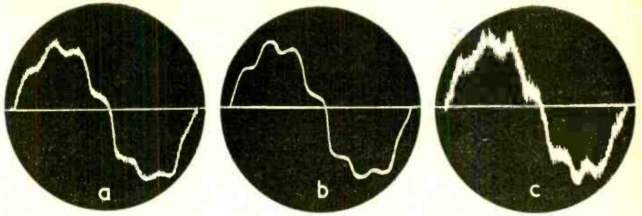
Fig. 5. How frequency response shows up when displaying a sound program on the oscilloscope screen: (a) is the wave presented "flat"; (b) shows high frequency loss; (c) high frequencies over-accentuated; (d) low frequency loss; and (e) low frequencies over-accentuated.
