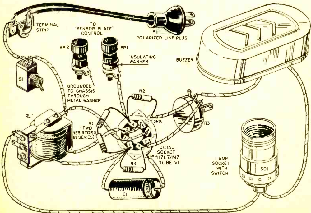
Pictorial diagram of the control unit of the rain alarm.
