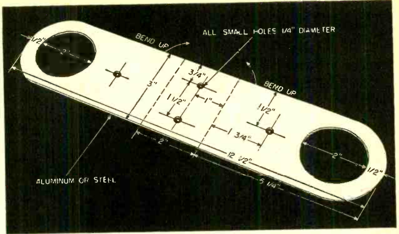
Fig. 1. Layout of the metal frame. The dimensions may be varied to suit the size of the clamp and solid rubber ball.
