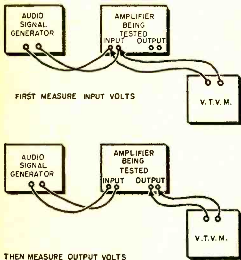
Fig. 3. Method of using an audio signal generator with a vacuum-tube voltmeter to measure amplifier frequency response.
