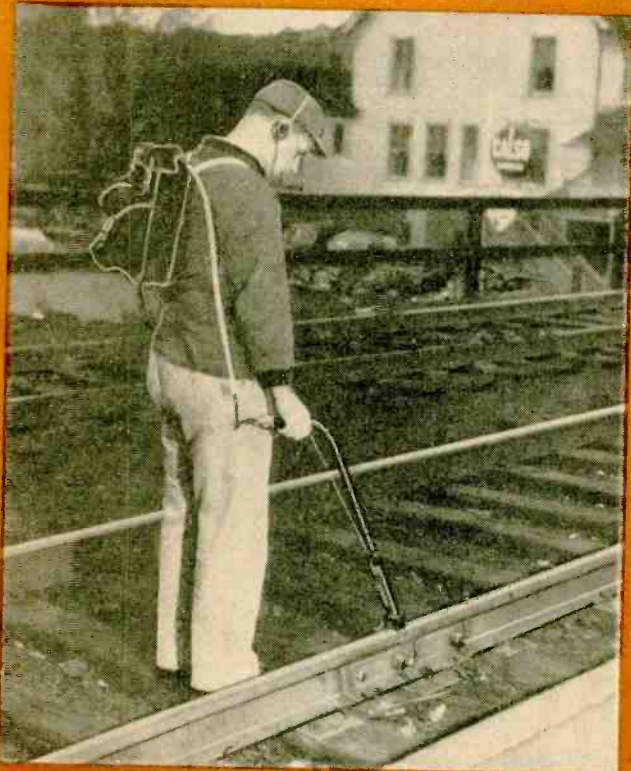
Using a portable ultrasonic flaw detector to check a railroad track rail for defects or cracks.
