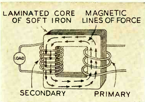
A magnetic field will couple the primary and secondary windings in a transformer.
