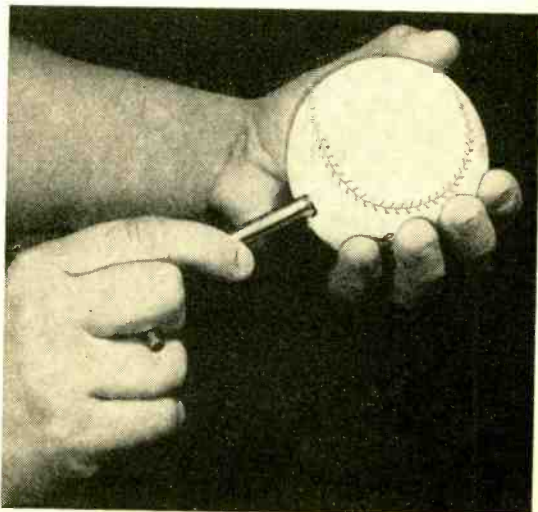
Fig. 2. Drill hole for the shaft in the rubber ball. Use a solid ball and "cork borer."
