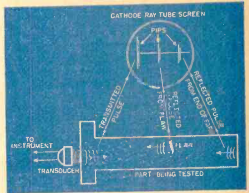
Fig. 4. Pulses of ultrasonic energy are reflected by flaws and displayed on a cathode-ray tube. Fig. 5. (below) Illustration of a method for examining odd-shaped metallic pieces for flaws using ultrasonic waves.
