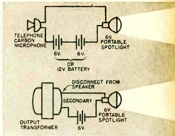
Fig. 1. These two simple transmitters may be used for short-range signaling.
