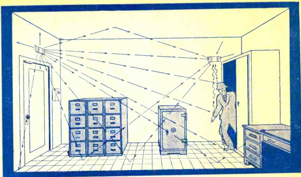
Fig. 6. This sketch illustrates the operation of the ultrasonic alarm system.
