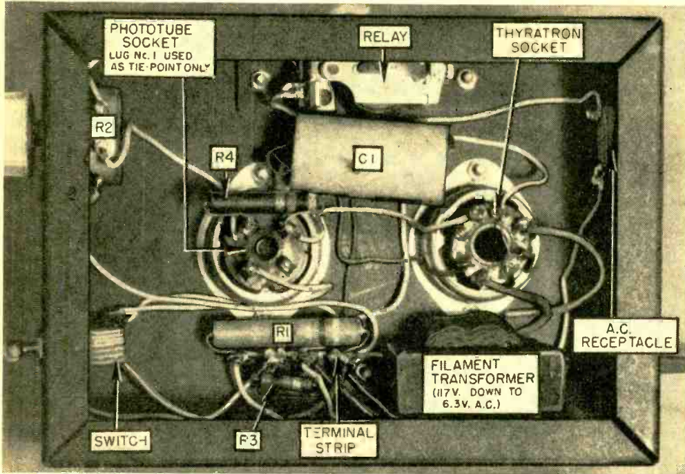
Underchassis view of the control box of the thyatron phototube relay showing the actual placement of parts and wiring details.
