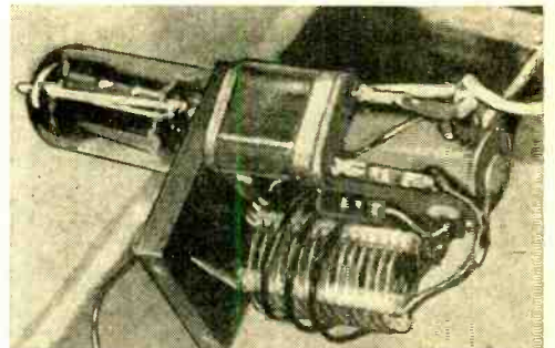
Detailed view of the Vector socket, showing the 27.255 mc. crystal holder made from the terminals of a miniature tube socket.
