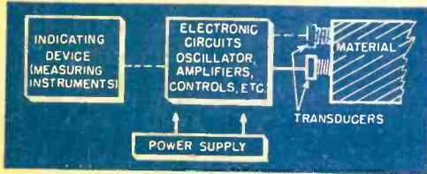
Fig. 1. Two basic transducer designs are shown above. Drawing (A) has a crystal element and drawing (B) a magnetostrictive core. Actual element movement in both cases is extremely small. Fig. 2. (below) shows a simplified block diagram of industrial ultrasonic equipment.
