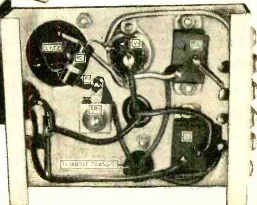
Bottom view of the miniature power supply chassis, showing wiring. See the schematic diagram for proper connections of the rectifier, SR_1 , and the transformer, T_1 .
