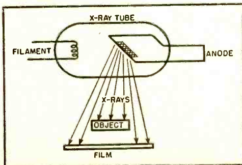
Electrons from filament hit anode at high speed; resultant radiation creates x-rays.
