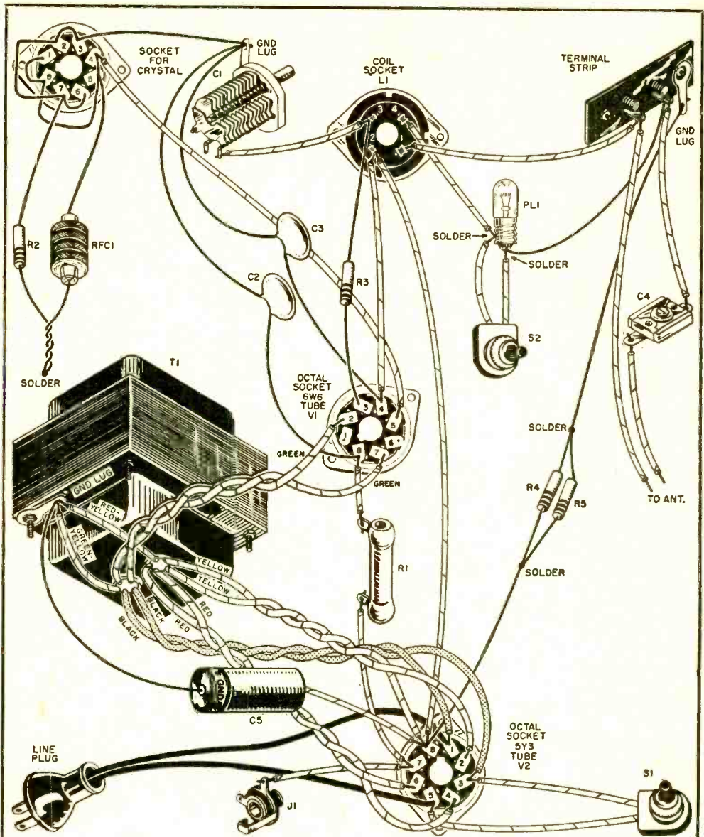
Fig. 4. The pictorial wiring diagram of the transmitter shows how the parts are connected; relative positions of the parts are not the same as on the actual chassis.
