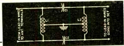
Schematic of high-pass filter for TV interference. Input and output terminals may be reversed since unit is symmetrically made.
