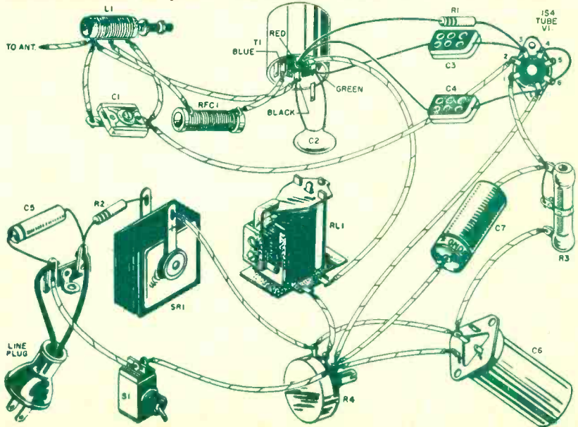
Receiver schematic and pictorial diagrams with complete list of parts required.
