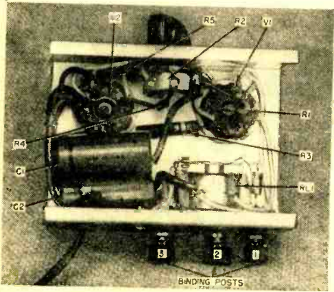
Pictorial wiring diagram. Some terminals on the V2 socket are used as wiring tie-points.
