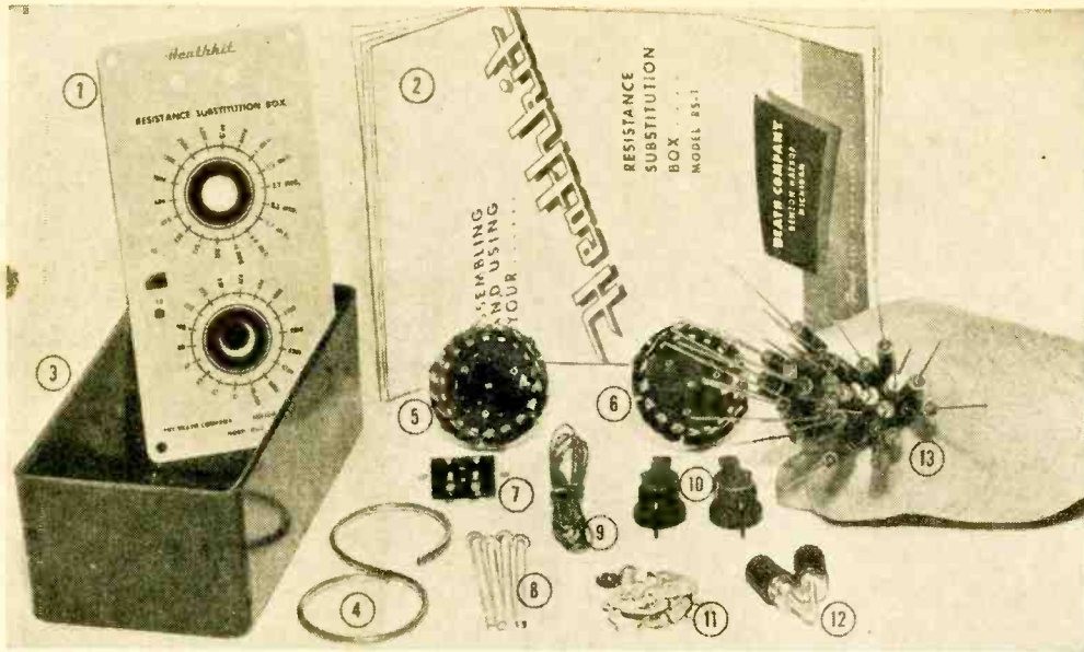
Components comprising the Heath resistance substitution box kit. The stack of 36 resistors is the "heart" of the instrument. (1) Front panel, (2) instruction booklet, (3) case, (4) "S" ring to hold ends of resistors, (5 & 6) rotary switches, (7) slide switch, (8) panel screws, (9) wire, (10) switch knobs, (11) mounting hardware, (12) binding posts, (13) resistors. See article for details.
