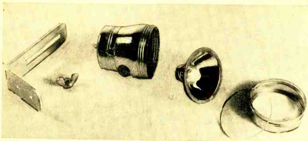
The light source for the annunciator is made from the parts of an ordinary flashlight.
