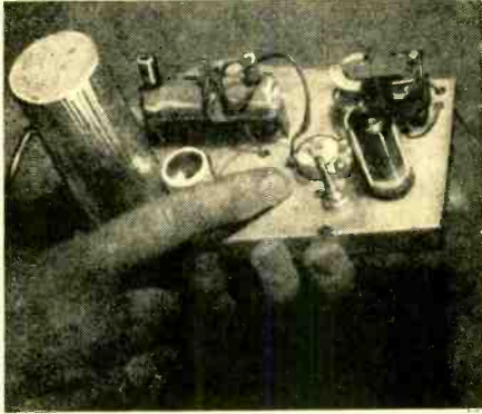
Top view of the receiver showing the arrangement of the parts and the two tuning controls.
