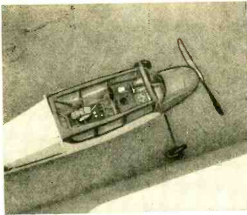
One method for mounting a receiver horizontally is shown here. Batteries and the socket for receiver cable are well forward.
