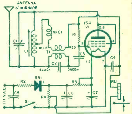
Receiver schematic and pictorial diagrams with complete list of parts required.
