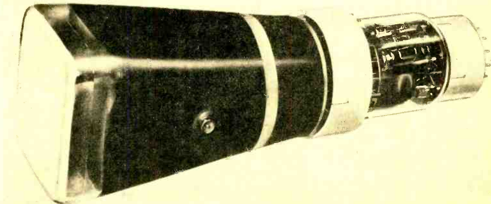
Fig. 6. This industrial multi-gun cathode-ray tube has five electron gun and deflection assemblies.
