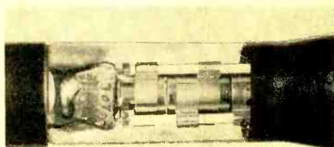
Fig. 3. Photographic illustration of the electron gun assembly of cathode-ray tube.
