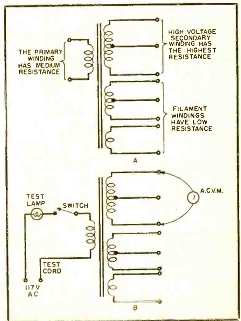
Fig. 2. (A) The general relationship between d.c. resistance and transformer winding. (B) A basic test circuit for checking transformer terminals.
