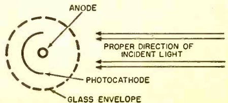
Proper orientation of phototube is with concave side of its cathode toward light source.
