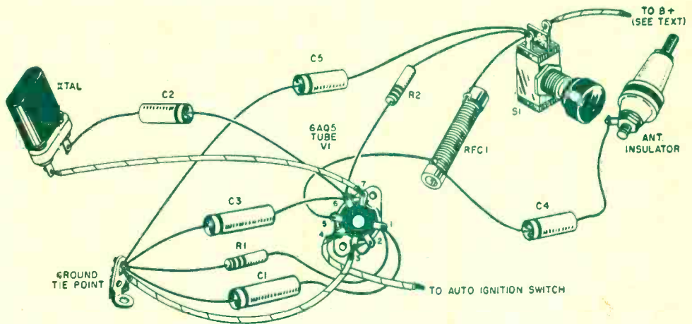
Pictorial diagram of the radio-controlled garage door transmitter.
