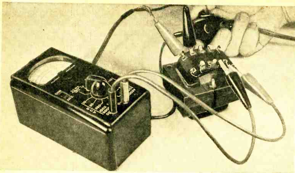
Fig. 3. How an a.c. voltmeter is used for final identification of transformer windings.
