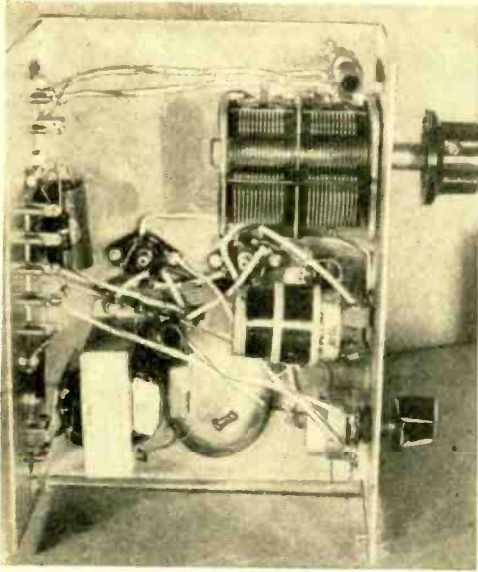
This bottom view of the reflex receiver shows the author's arrangement of the parts. It should be used with the pictorial and schematic wiring diagrams in constructing the set.
