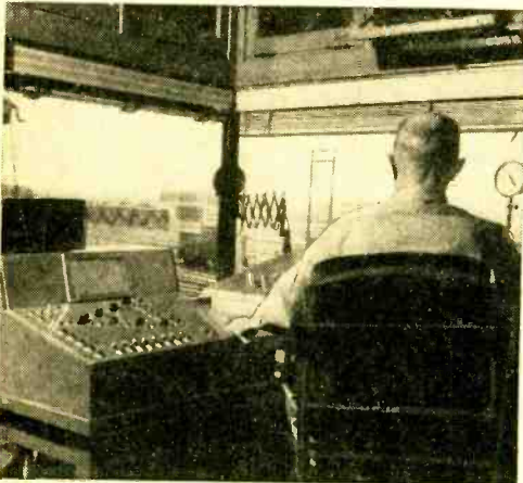
At left is control console for "electronic yardmaster." In front of operator are conventional retarder and switching controls.
