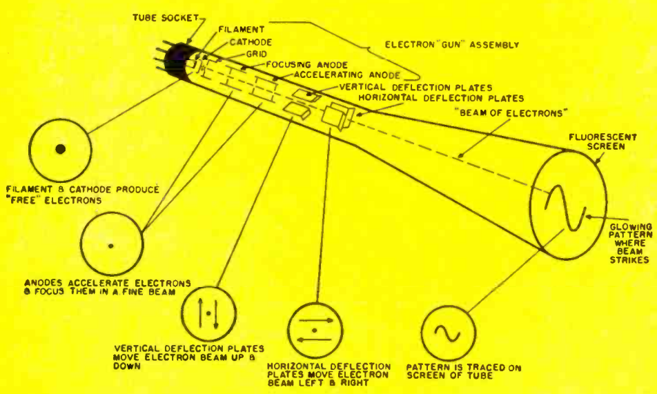
Fig. 2. Construction details of an electrostatic type cathode-ray tube.
