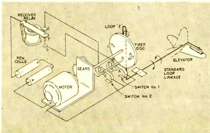
Fig. 5. Physical drawing indicating how a servo may be used in a radio-control model airplane for proportional control of the elevator. It can be used also for the rudder.
