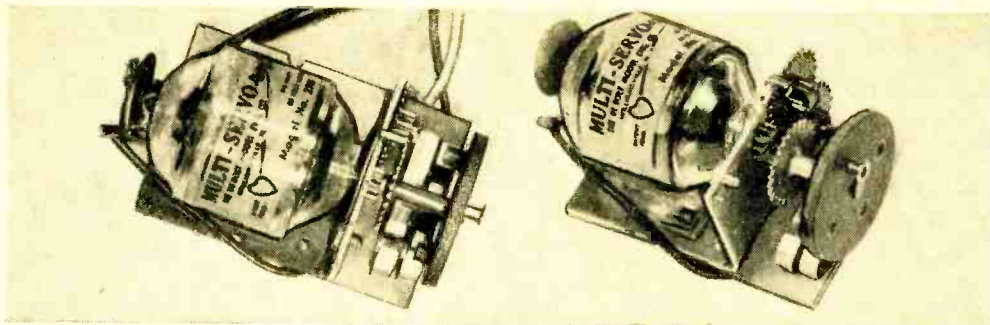
Fig. 4. Top and side views of a typical servo unit for radio control. Motor is about 1" wide.
