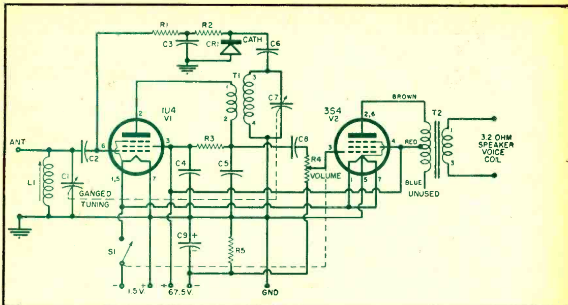
In the circuit shown in the schematic diagram above, V 1 acts as both radio-frequency and audio-frequency amplifier. See the text for an explanation of how this is accomplished.
