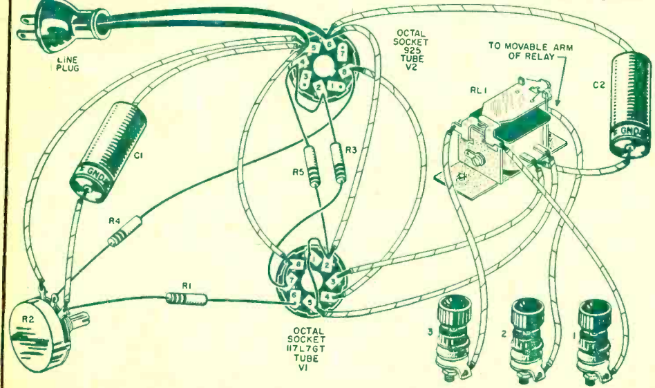
Pictorial wiring diagram. Some terminals on the V2 socket are used as wiring tie-points.
