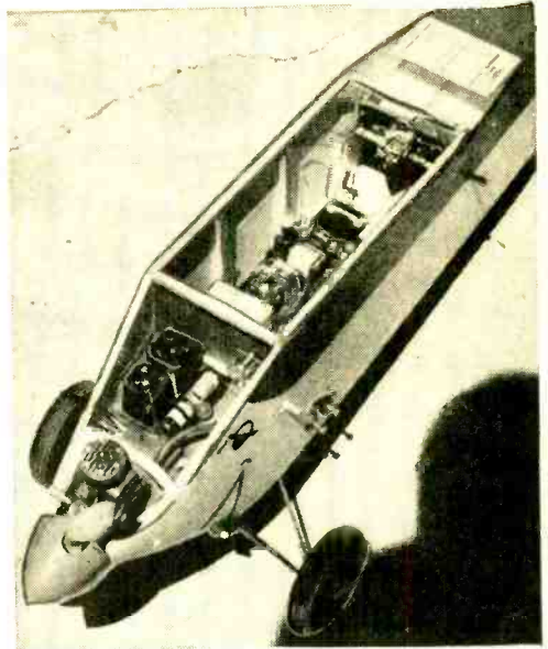
One method for mounting a receiver horizontally is shown here. Batteries and the socket for receiver cable are well forward.
