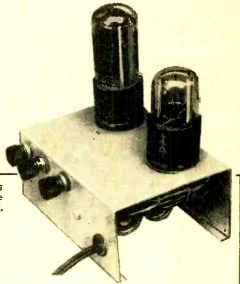
Proper orientation of phototube is with concave side of its cathode toward light source.
