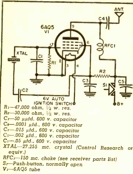
On the left is the schematic diagram of the transmitter and its parts list. Above is a view of the transmitter constructed by the author and added onto his regular auto radio power supply chassis; note the subchassis.
