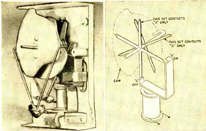
Far left, Fig. 2. Back view of an ECCO compound escapement which uses two four-finger units and two cam wheels to actuate two "Y" yokes, each with its own shaft. This allows two control functions. Left, Fig. 3. Simplified drawing of the ECCO compound escapement showing how the four-finger units operate separately with a single solenoid.
