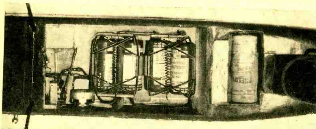
Example of battery installation in the belly of an airplane under the hardwood floor. The forward box contains a hearing-aid "B" battery, the rear compartment contains the batteries for the receiver filaments (1½ volts) and the escapement requiring 3 volts.
