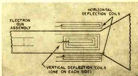
Fig. 4. In an electromagnetic type of tube, deflection coils are placed on the outside.
