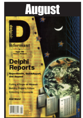
Delphi Reports
