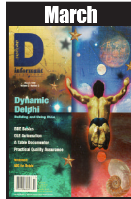
Dynamic Delphi
