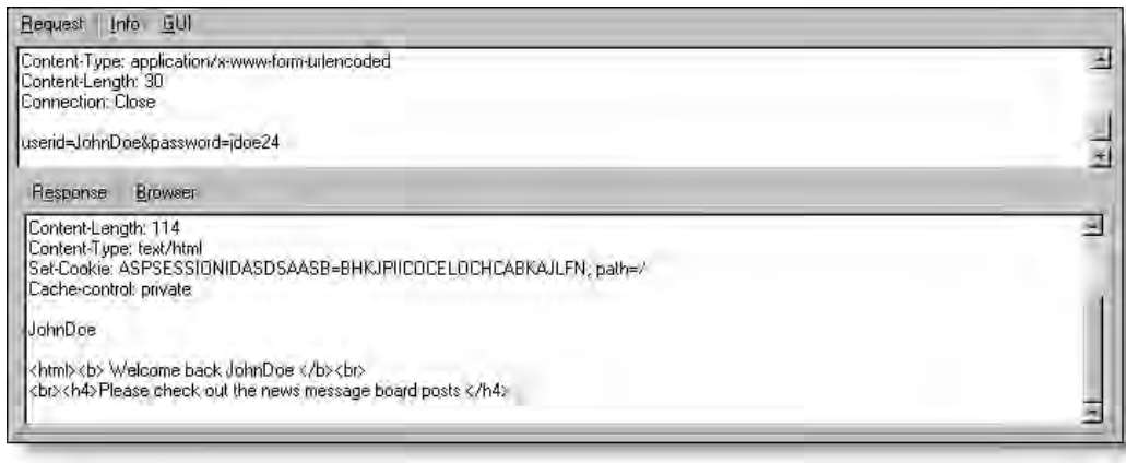
Figure B.17 HTTP Response That Suggests Susceptibility to Cross-Site Scripting
