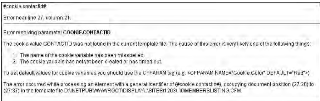
Figure B.4 Error Message Revealing the Web Root and Other Details
