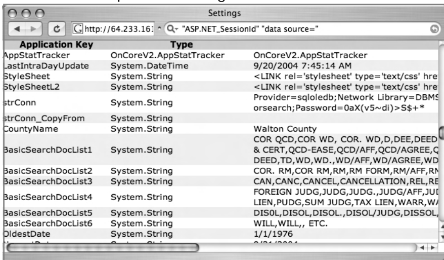
Figure 8.10 ASP Dumps Provide Dangerous Details
