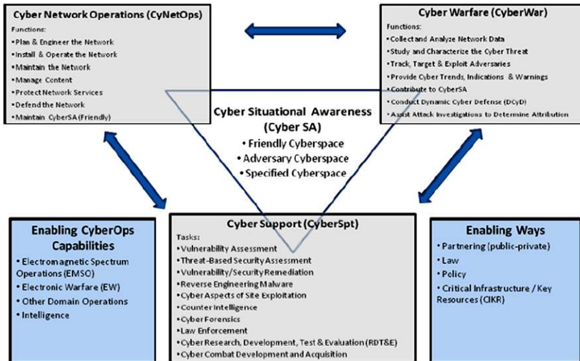
FIGURE 3.3 CyNetOps Framework [8]
