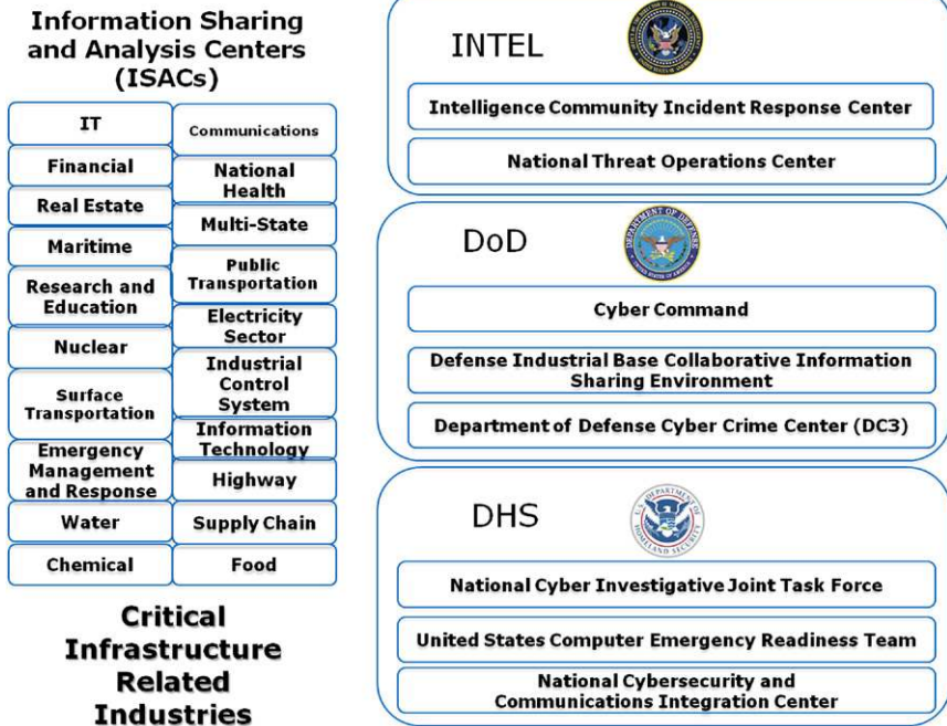
FIGURE 3.2 Cyber Centers
