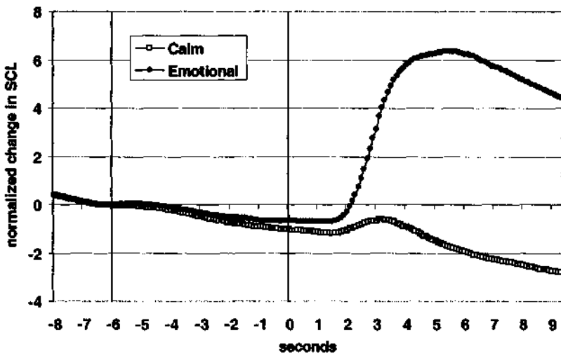
Fig. 4. Average normalized change in skin conductance level (ASCL) for calm and emotional trials in Experiment 3. Each trial was initiated at -6 seconds; stimulus onset was at 0 seconds. A total of 1,410 trials were contributed by 47 participants. Randomized permutation analysis indicates that the difference in pre-stimulus curves is associated with z = 3.34 , p = 0.0004 (one-tailed).
