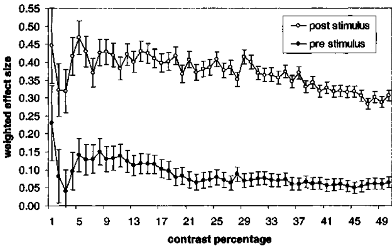
Fig. 6. Weighted mean effect size and one standard error bars for post-stimulus and pre-stimulus ASCL, in terms of emotional contrast percentage. An emotional contrast percentage of 1 % represents those trials with the most emotional 1 % and most calm 1% of the trials, or 2% of all available trials. The 50% contrast level includes all trials.
