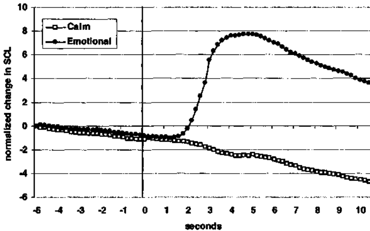
Fig. 3. Average normalized change in skin conductance level (ASCL) for calm and emotional trials in Experiment 2. This experiment consisted of a total of 2,059 trials, contributed by 56 participants. Randomized permutation analysis indicates that the difference in pre-stimulus ASCL curves is associated with z = 1.23 , p = 0.110 (one-tailed).
