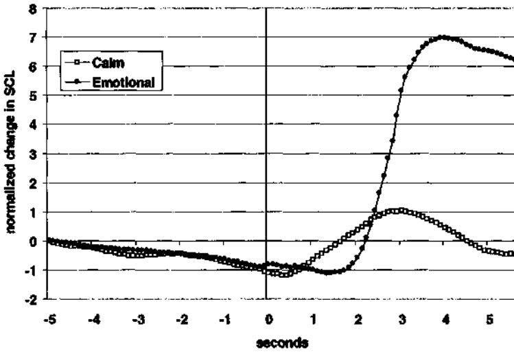
Fig. 5. Average normalized change in skin conductance level (ASCL) for calm and emotional trials in Experiment 4. A total of 240 trials were contributed by six participants. Randomized permutation analysis indicates that the difference in pre-stimulus curves is associated with z = 0.59 , p = 0.28 (one-tailed).
