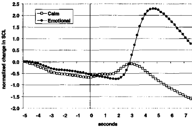
Fig. 2. Average normalized change in skin conductance level (ASCL) for calm and emotional trials in Experiment 1. A total of 860 trials were contributed by 24 participants. The pre-stimulus period is indicated by negative seconds; stimulus onset was at time 0; stimulus offset at 3 seconds. Randomized permutation analysis indicated that the observed difference in pre-stimulus SCL is associated with z = 2.92 , p = 0.002 (one-tailed).
