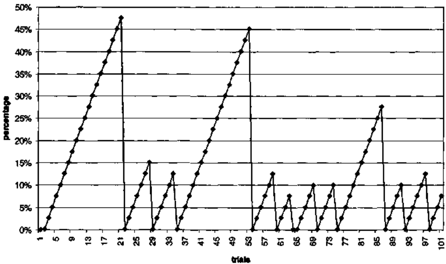
Fig. 7. Simulation of an idealized anticipatory strategy. The y-axis is the degree of autonomic arousal, the x-axis is successive trials. The top of each "arousal" ramp represents an emotional trial; all other trials are calm.
