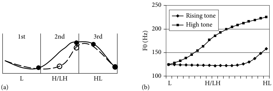
Figure 10.1 Theoretical Mandarin Chinese pitch contours of High tone and Rising tone between Low tone and Falling tone (panel (a)), and actual pitch contours of High tone (■) and Rising tone (◆) after low tone and before falling tone, averaged over 27 tokens (panel (b), from Chen 2008).
