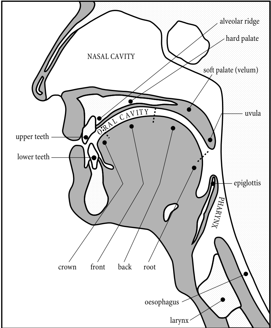
Figure 2.4 Cross-section of the vocal tract.
