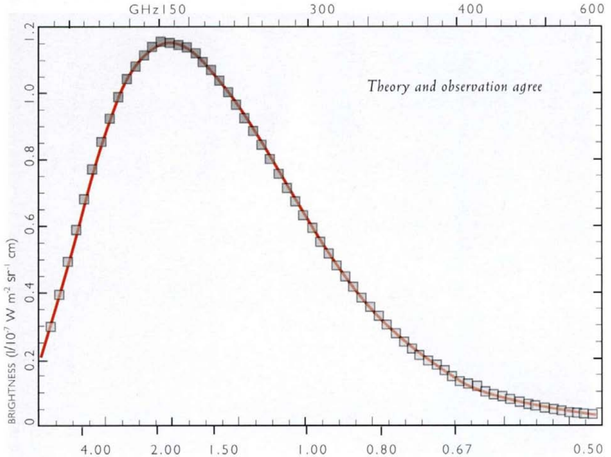
(FIG. 2.6) MEASUREMENT OF THE SPECTRUM OF MICROWAVE BACKGROUND
