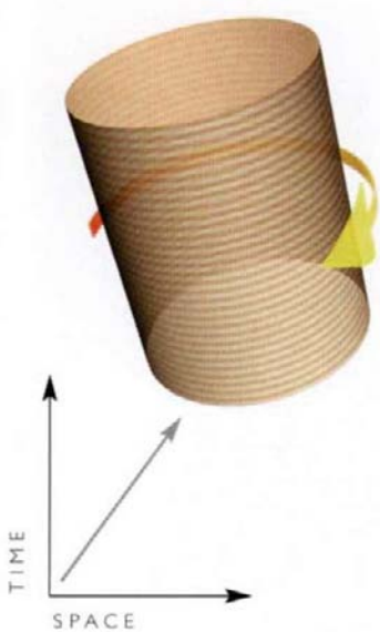
(FIG. 5.16) The Einstein universe is like a cylinder: it is finite in space and constant in time. Because of its finite size, it can rotate at less than the speed of light everywhere.
