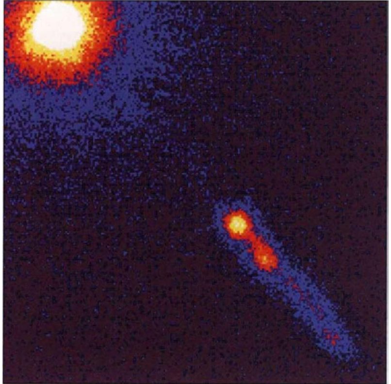
(FIG. 4.10) The quasar 3C273, the first quasi-stellar radio source to be discovered, produces a large amount of power in a small region. Matter falling into a black hole seems to be the only mechanism that can account for such a high luminosity.
