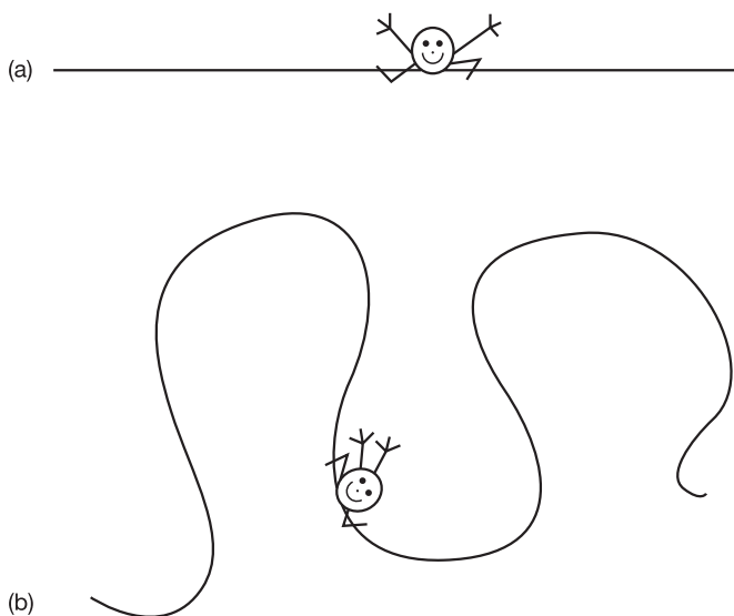
Figure 1.1. Fred the dot living in his one-dimensional universe that is (a) flat and (b) curved.
