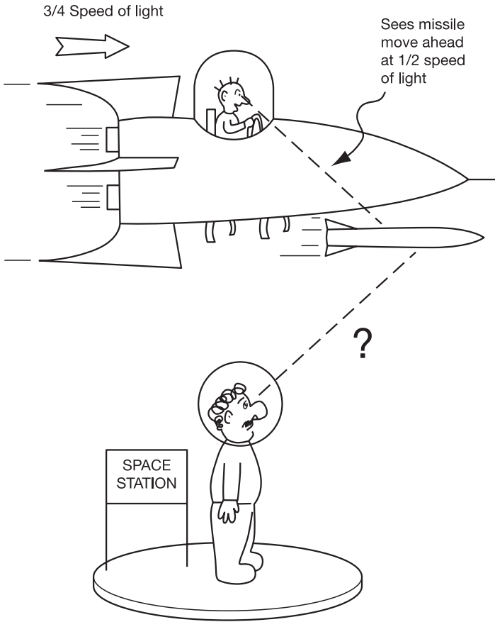
Figure 6.2. According to the normal rules of adding up speeds, the space station observer should see the missile travelling at \frac{3}{4} + \frac{1}{2} = 1\frac{1}{4} times the speed of light. Einstein showed that nothing can go faster than light and the way we add up speeds had to be changed.
