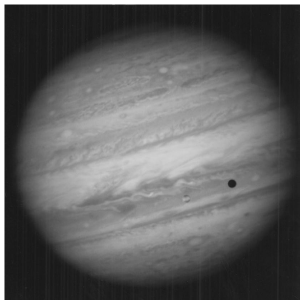
Fig. 1. Telescopic appearance of Jupiter from the Hubble Space Telescope (Space Telescope Science Institute; Jet Propulsion Laboratory; NASA).
