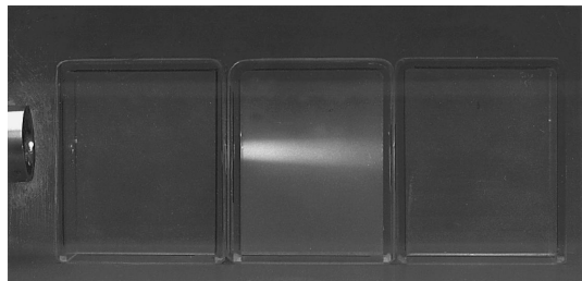
The luminous light path known as the Tyndall cone or Tyndall effect. (Courtesy of H. Steeves and R. G. Babcock)
