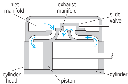
Fig. 2. Single-ported slide valve on counterflow double-acting cylinder.
