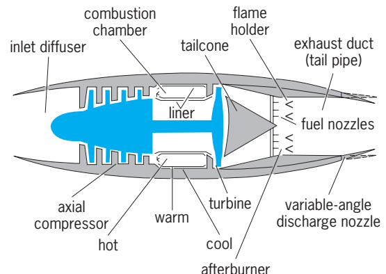
Diagram of turbojet engine showing afterburner.
