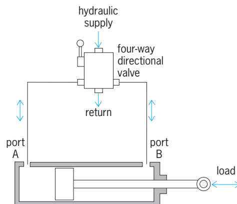
Fig. 1. Function of a hydraulic double-acting cylinder.
