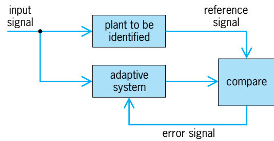
Adaptive system identification.
