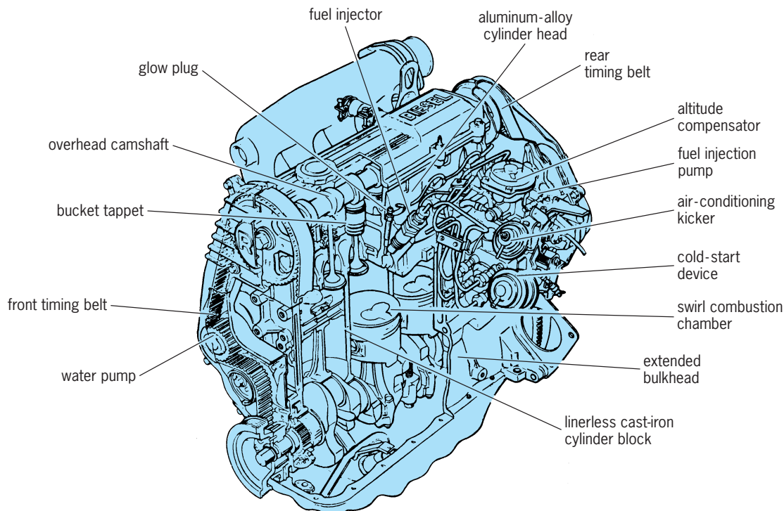
A 2.0-liter, four-cylinder, four-stroke-cycle passenger-car diesel engine which has a distributor-type injection pump and indirect injection. (Ford Motor Co.)
