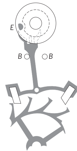
Fig. 2. Detached-lever escapement, often used in modern watches. (After F. J. Britten, Britten's Old Clocks and Watches and Their Makers , 7th ed., Dutton, 1956)
