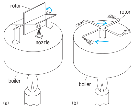
Turbine principles. (a) Impulse. (b) Reaction.
