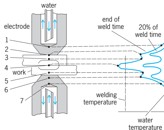
Distribution of temperature in local (numbered) elements of a spot-welding operation.
