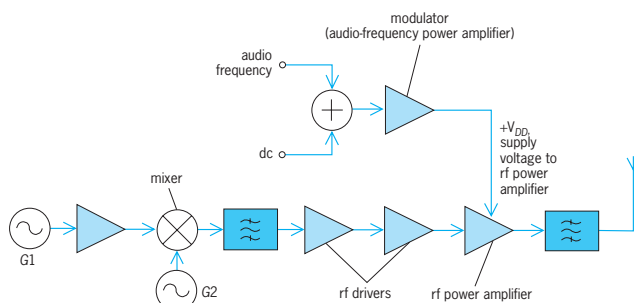
Fig. 2. Amplitude-modulation (AM) transmitter.
