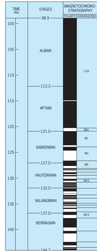
Stages of the Cretaceous Period, their estimated ages in years before present, and polarity chrons representing the alternation between episodes of normal (black) and reversed (white) orientations of the Earth's magnetic field. (After F. M. Gradstein et al., in W. A. Berggren et al., eds., Geochronology, Time Scales and Global Stratigraphic Correlations , SEPM Spec. Publ., no. 54, 1995)
