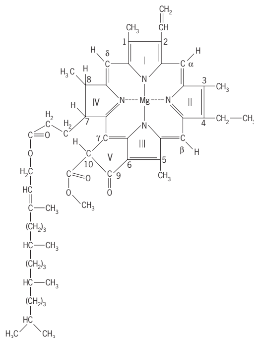
Structure of chlorophyll a (C 55 H 72 O 5 N 4 Mg).
