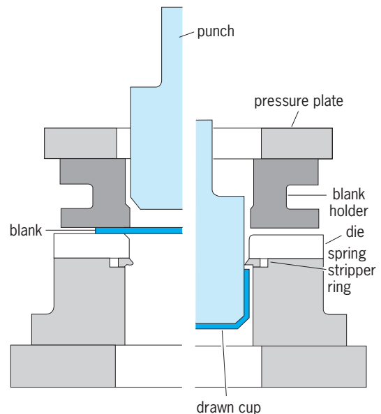
Fig. 3. Deep-drawing process.
