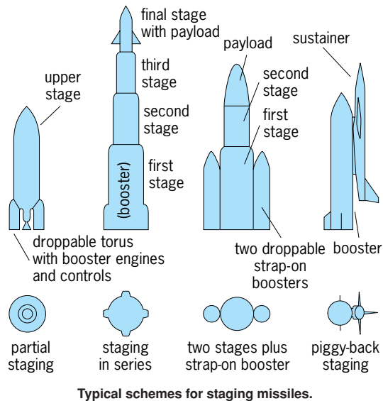
Typical schemes for staging missiles.
