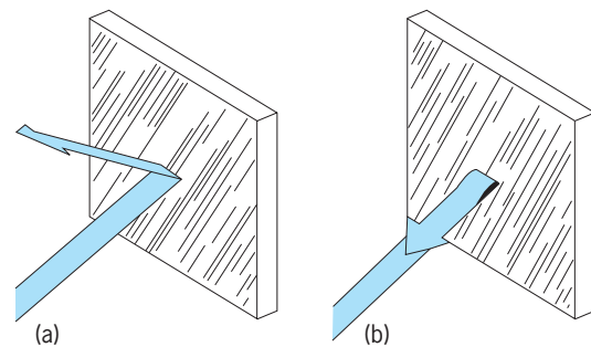
Comparison of reflections (a) from a conventional mirror and (b) from an optical phase conjugator. (After V. J. Corcoran, ed., Proceedings for the International Conference on Laser '78 for Optical and Quantum Electronics , STS Press, McLean, Virginia, 1979)
