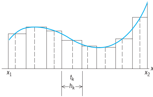
Fig. 2. The definite integral.
