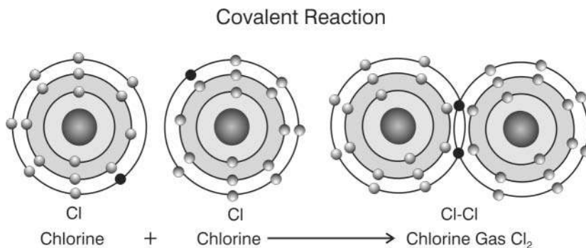
Figure S2. A depiction of a covalent reaction between two chlorine atoms (each with an outer orbit of 7 electrons) sharing two electrons to form a chlorine molecule (Cl 2 ).
