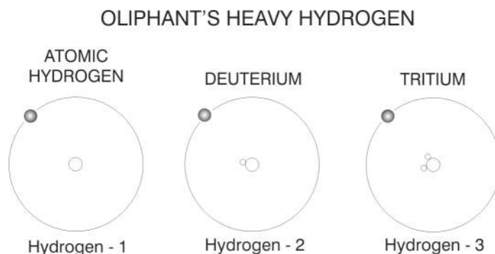
Figure O1. Harold Urey produced heavy hydrogen atoms with one proton and one neutron (deuterons). Marcus Oliphant bombarded deuterons with other deuterons to produce a third isotope of hydrogen—tritium, with two neutrons and one proton. The three isotopes of the hydrogen atom exhibit minor differences in chemical properties due to differences in atomic weights. These differences are minor for chemical reactions involving isotopes of heavier elements. Heavy hydrogen atoms are used to facilitate nuclear reactions.
