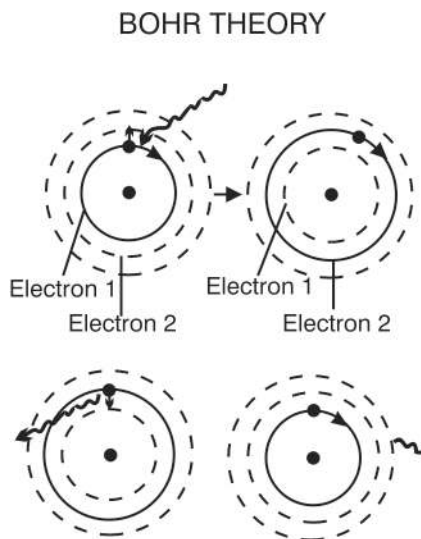
Figure B6. When electrons move from a stable energy level of atoms, they emit discrete packets of energy.
