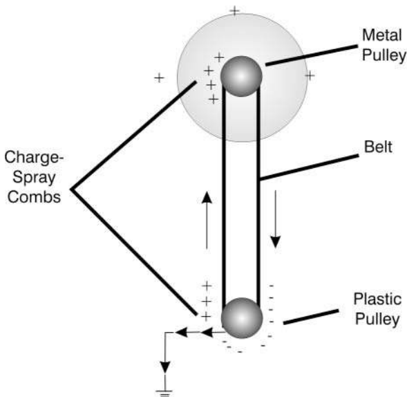
Figure V1. The Van de Graaff electrostatic generator produces an electrical charge from the ground and transfers it by the belt to the metal sphere, where it can be used as an electron source for a variety of research applications.
