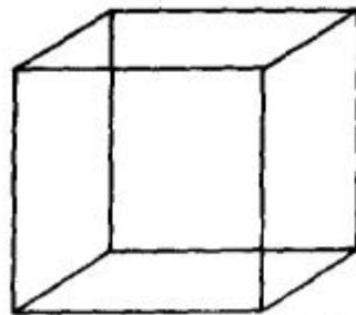
Necker Cube
