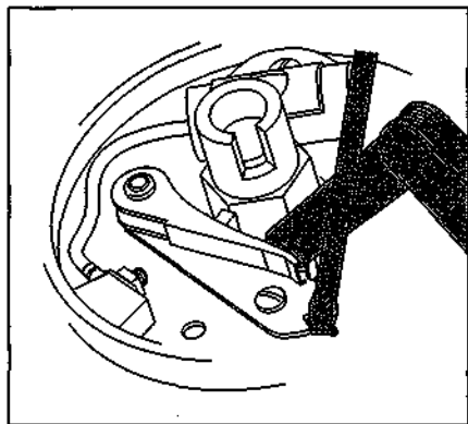
Figure 12-38: Adjusting slot-type points.
