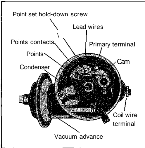
Figure 12-15: The anatomy of a non-electronic distributor.
