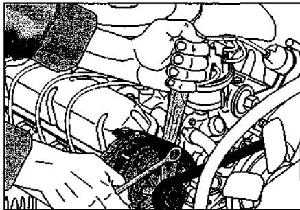
Figure 14-15: •lightening the adjust- ment bolt
