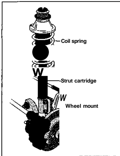
Figure 11-4: Conventional strut suspension.
