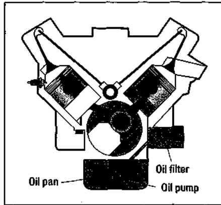
Figure 15-1: Oil is filtered as it circulates through the engine.
