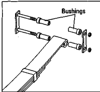
Figure 16-6: Leaf springs have rubber bushings to cushion them.
