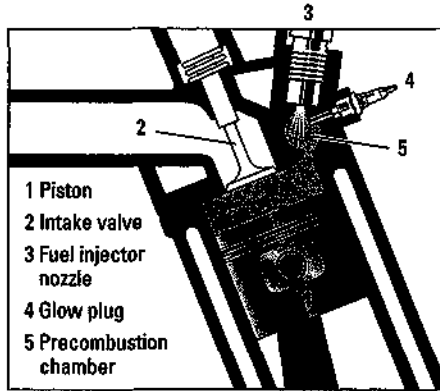
Figure 7-2: Glow plugs warm up the air in the cylinders.
