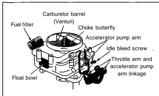
Figure 21-1: Atypical carburetor.
