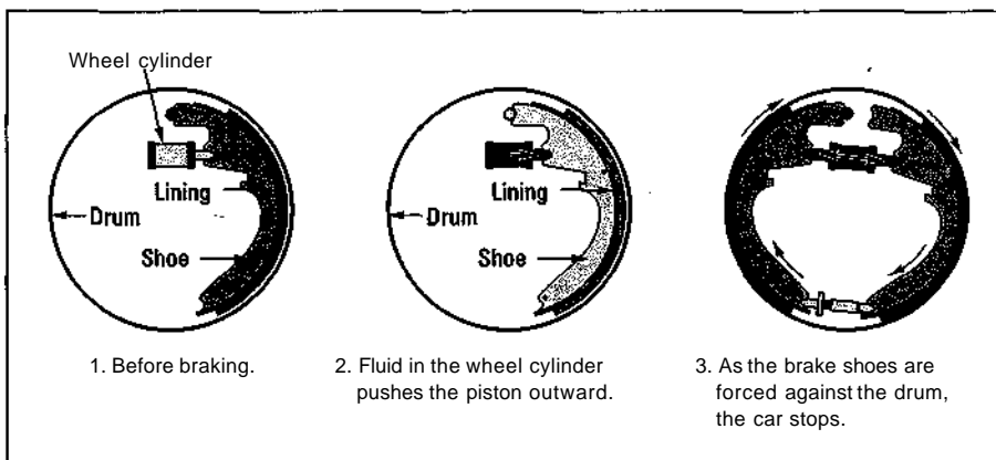
Figure 10-7: A drum brake in action.
