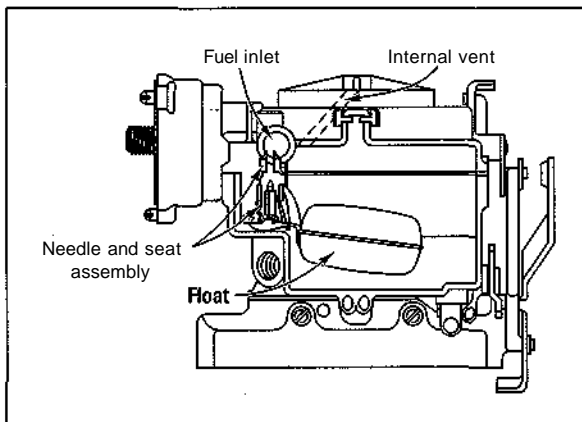
Figure 6-4: The float bowl is inside the carburetor.
