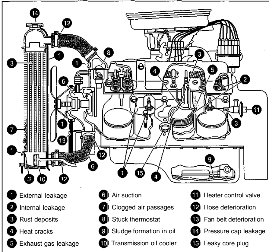
Figure 14-4: Where to check for leaks and other problems.
