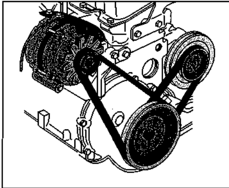
Figure 3-2: Accessory belts.
