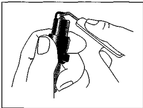
Figure 12-12: Gapping a plug with a wire gauge.
