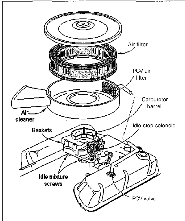
Figure 6-3: The carburetor.
