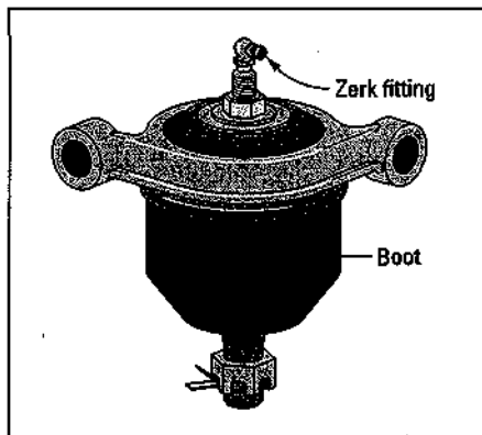
Figure 16-3: A zerk fitting on a ball joint.
