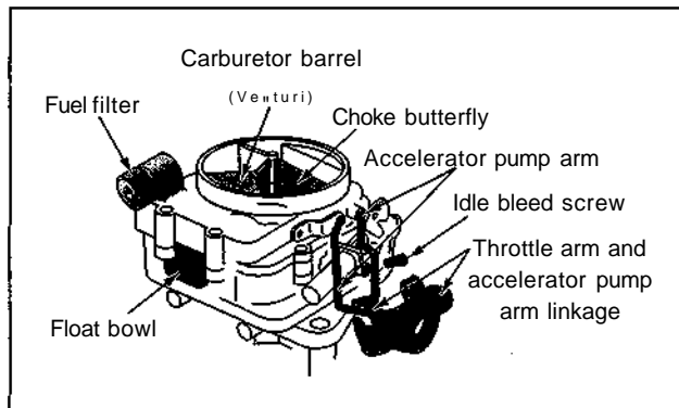
Figure 13-9: Atypical carburetor.
