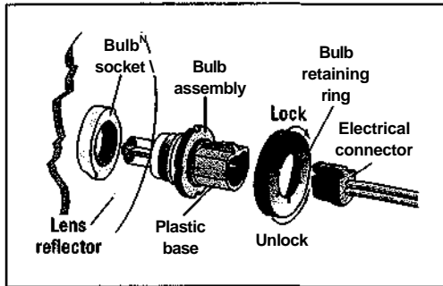
Figure 12-53: Replacing a halogen bulb.
