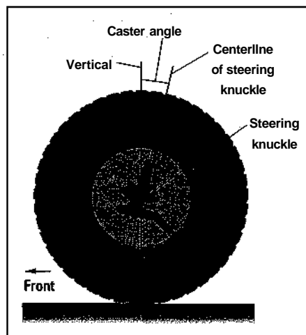
Figure 19-4: Caster.
