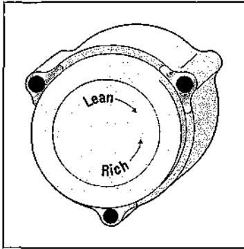
Figure 13-16: The three screws you need to loosen when you adjust a thermostatic spring choke.
