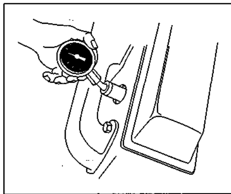
Figure 13-19: Checking compression.
