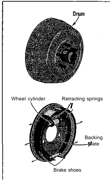
Figure 10-5: Anatomy of a drum brake.
