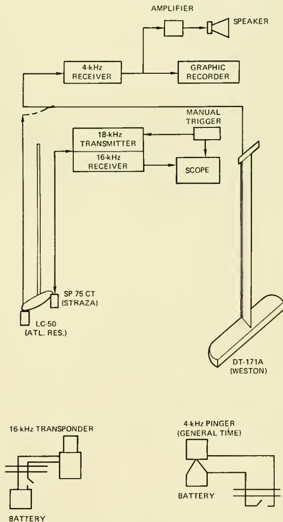
Fig. 10.17 Tracking system block diagram.
