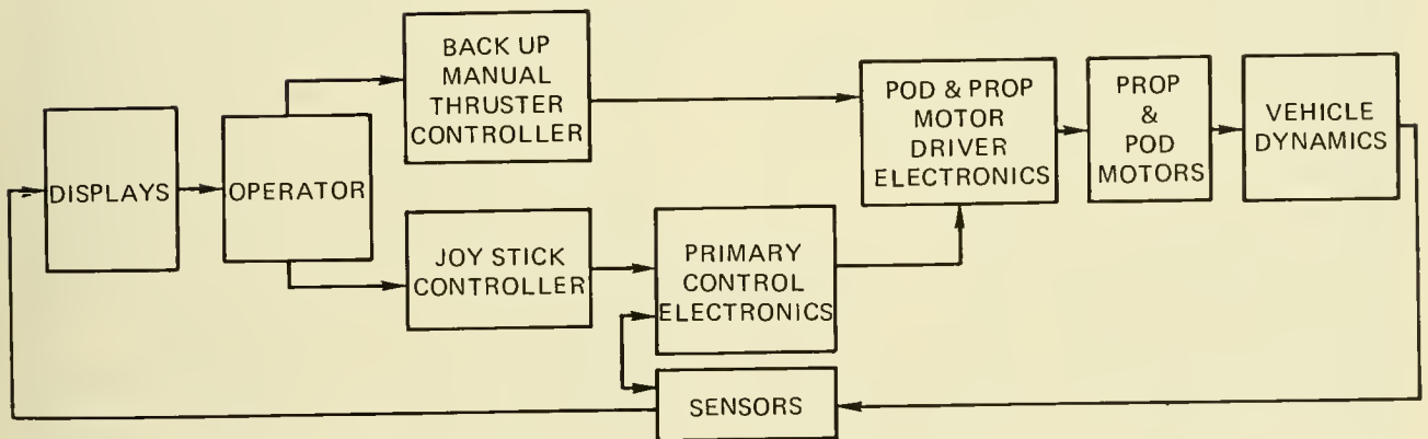
Fig. 8.32 Primary and backup control components of BEAVER.
