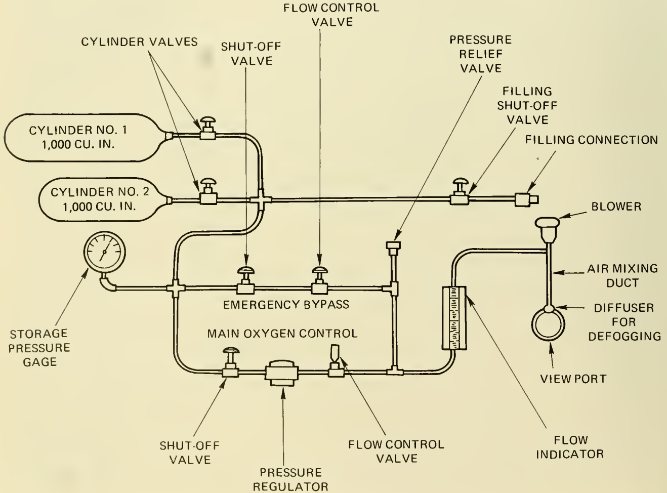
Fig. 9.2 Oxygen supply system schematic. [From Ref. (10)]
