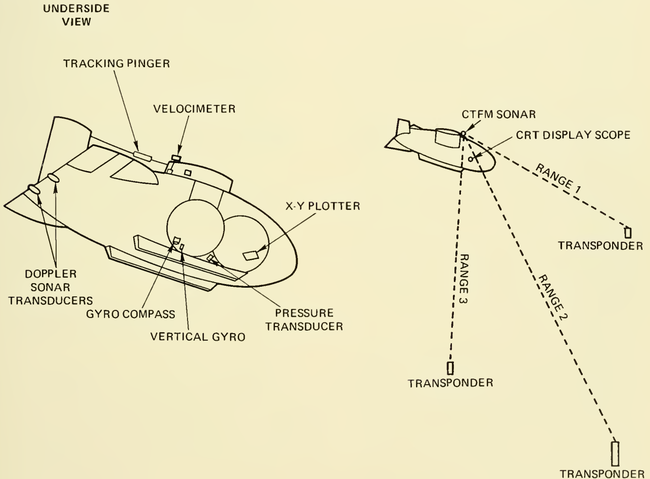
Fig. 2.8 DEEP QUEST 's navigational components.
