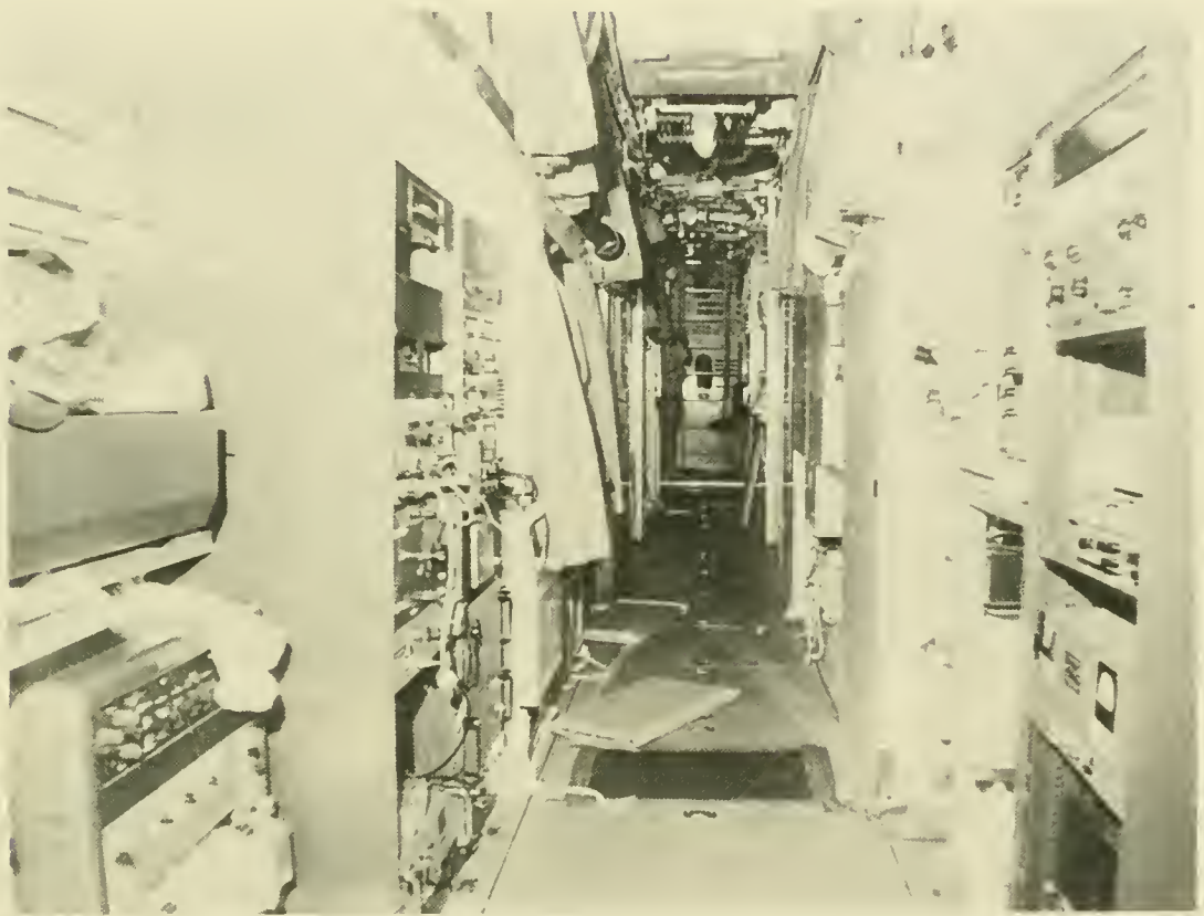
Fig 9 19 Assorted activities aboard BEN FRANKLIN during and prior to its 30-day drift in July-August 1969. a) Interior view looking forward from the aft hemi-head. (Grumman Aerospace Corp.)
