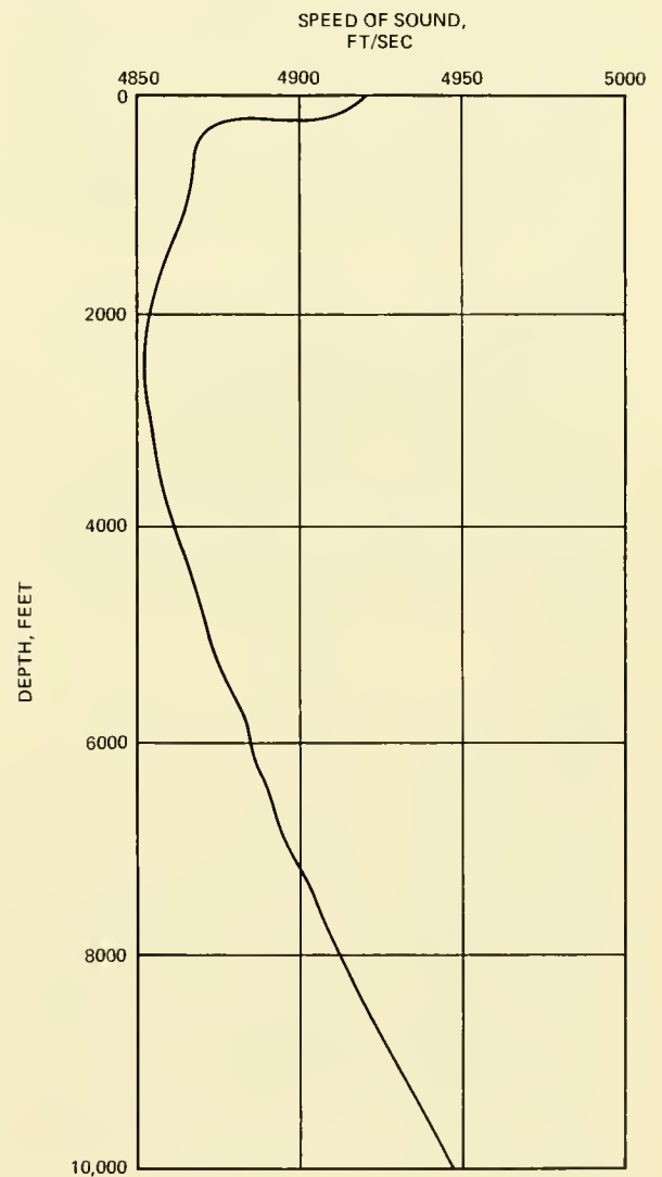
Fig. 2.2 Typical variation of speed of sound with depth in the ocean.
