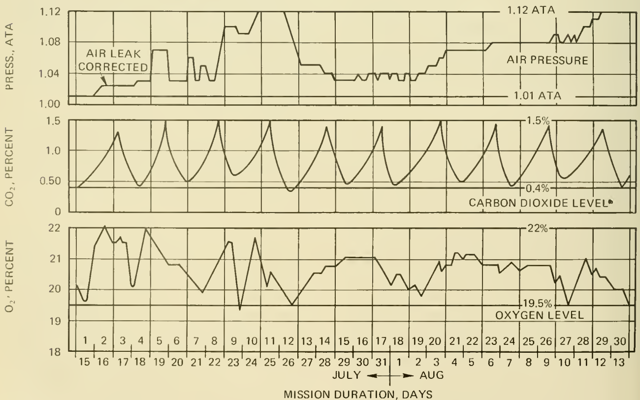
Fig. 9.22 Log of air pressure, CO 2 and O 2 inside BEN FRANKLIN. [From Ref. (16)]
