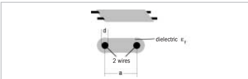
Fig. 13: Twin line
