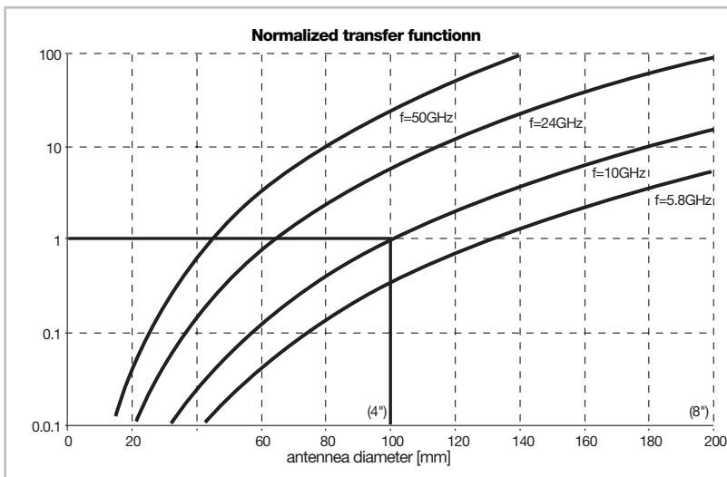
Fig. 27: Transfer function of radar systems using different frequencies and antenna sizes (normalized to D = 100 \text{ mm} (4") at 10 GHz)
