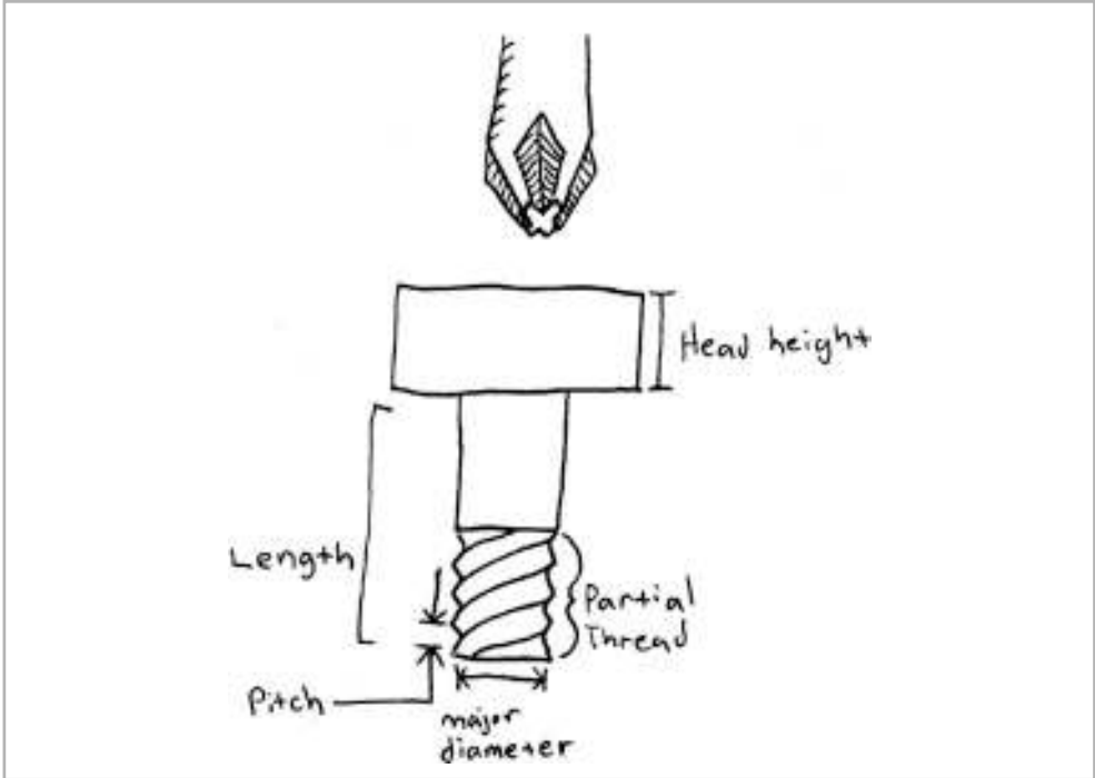
FIGURE 3-2 Screw anatomy
