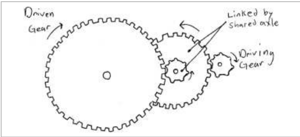
FIGURE 7-39 Compound gear system
