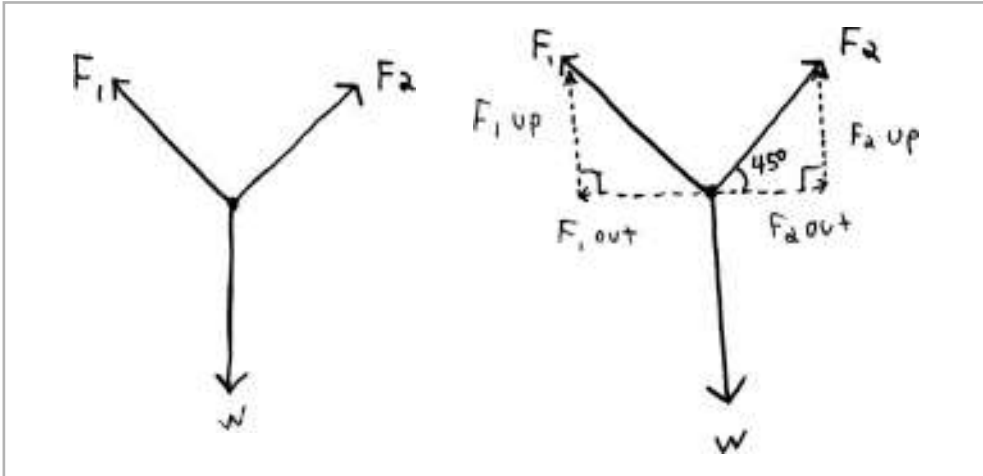
FIGURE 4-11 Free body diagram of paint can platform in Graffbot (left) and rope forces broken up into components (right)
