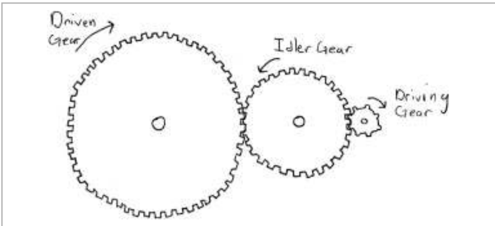
FIGURE 7-38 Idler gears change the direction of rotation without changing the gear ratio.
