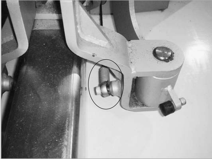
FIGURE 7-11 Spherical bearings are used on gym equipment to accommodate misalignment in the cable pull direction.
