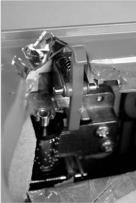
FIGURE 7-44 A compression spring returns the latch in a jack-in-the-box.
