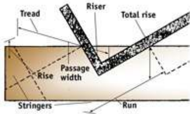
FIG. 2 - The components of a stairway, with basic stair-building terms. From the Sunset book, Decks , © Sunset Publishing Corporation
