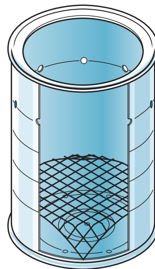
▲ Fuel shelf made with \frac{1}{4} " hardware cloth
