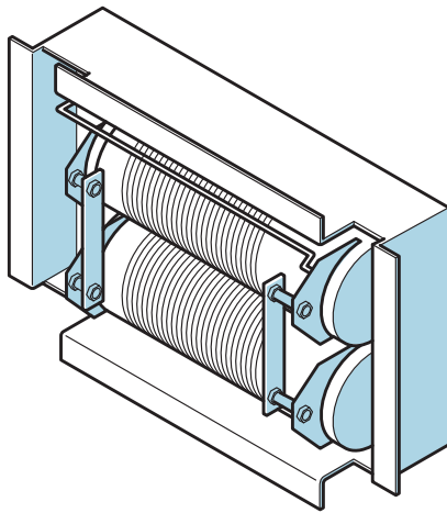
Typical dump loads: low-voltage water heater element (top) and electric resistance air heater (bottom) ▶
