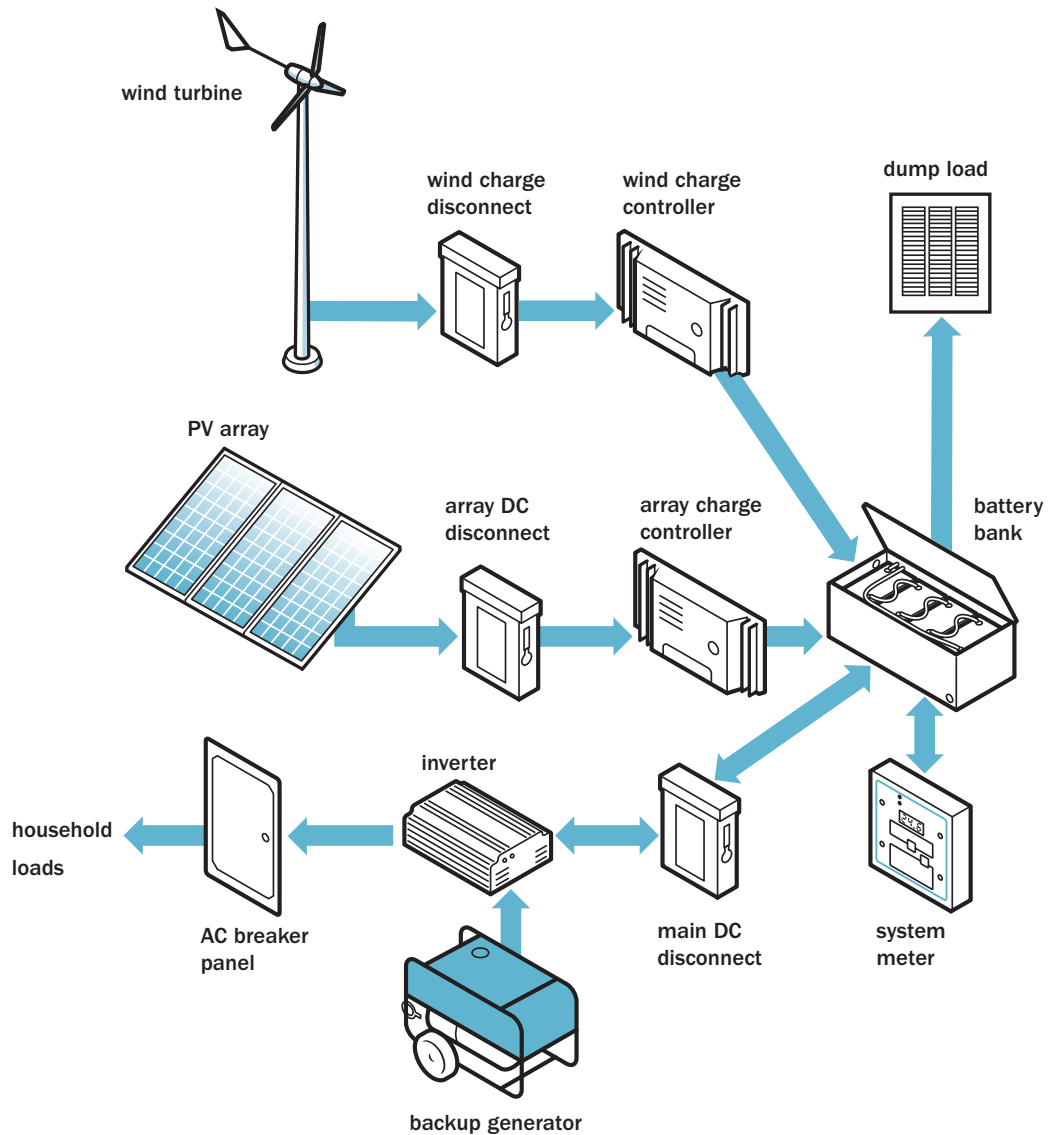
◀ A hybrid wind and solar electric power system that is grid-connected with battery backup
