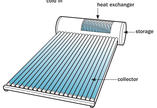
▲ Indirect ICS with separate collection and storage
