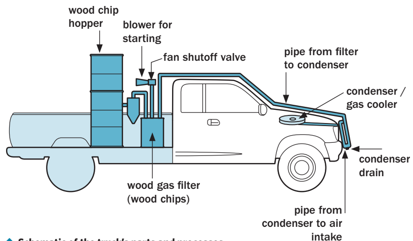
▲ Schematic of the truck's parts and processes
