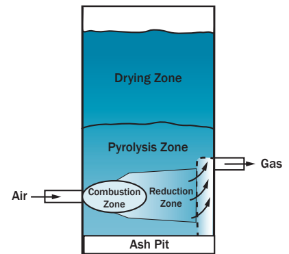
▲ Schematic of crossdraft gasifier
