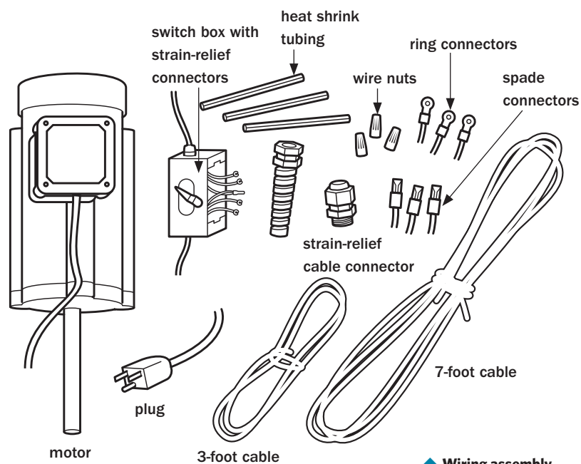
▲ Wiring assembly for motor, switch, and plug
