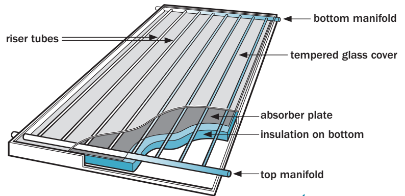
◀ Flat plate collector, cutaway view
