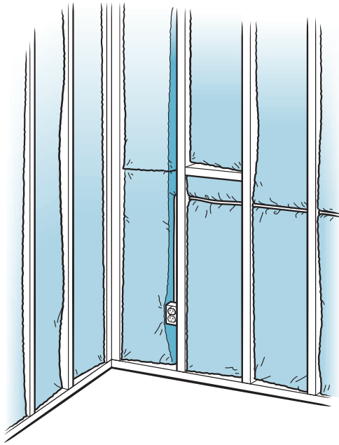
▲ Poorly installed wall insulation with compression, gaps, and voids
