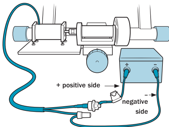
▶ Completed wiring between generator and battery. Cover the connections with wire loom for protection.
