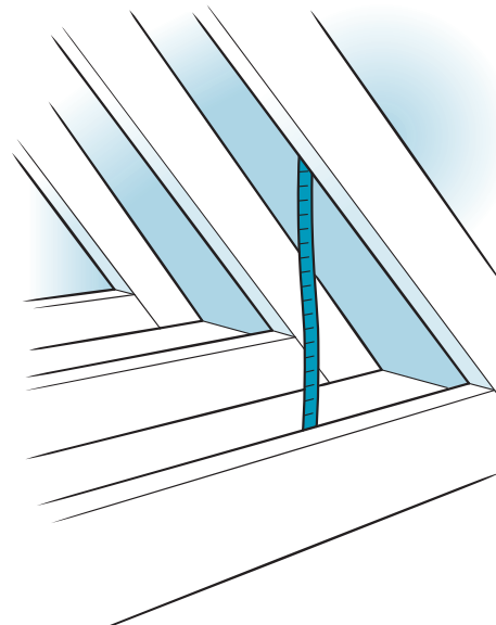
▲ Insulation properly cut to fit around wires and fit snugly into wall framing
