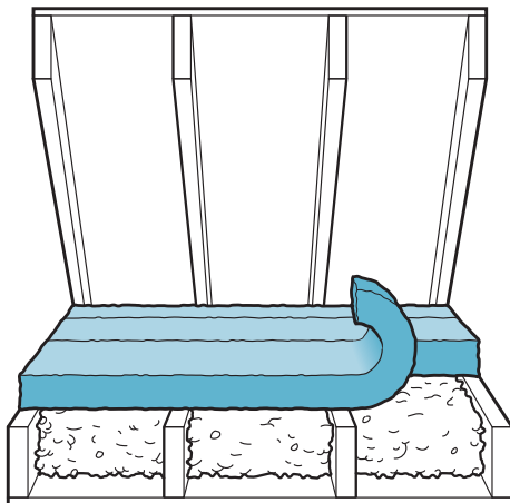
▲ Properly installed fiberglass insulation in an attic. There are two layers of insulation: the first lies between the framing members on the attic floor; the layer on top is perpendicular to the one on the bottom, eliminating the thermal bridge of wood framing.
