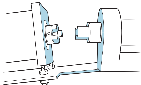
▲ Fitting the generator and plate into position, with the couplings loosely fitted onto the generator and roller shafts
