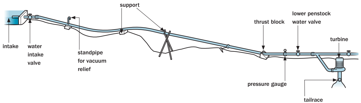
▲ Micro-hydro system components and layout.
