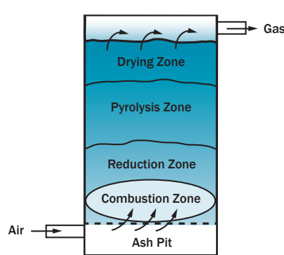
▲ Schematic of updraft gasifier
