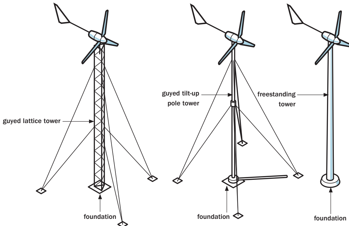
◀ Types of towers
