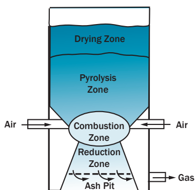
▲ Schematic of downdraft gasifier
