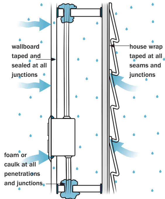
▲ This cutaway shows a simple wall assembly with elements to stop airflow while allowing for the movement of water vapor. A well-sealed drywall finish on the inside stops airflow and slows water vapor. On the exterior, sheathing and building wrap keep air out of the wall cavity and let water vapor drain away to keep the cavity dry.
