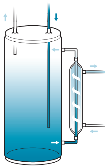
◀ Tube-in-shell (“side-arm”) heat exchanger. Fluid is pumped from the collector to the heat exchanger, but a thermosiphon provides the pumping action from the bottom of the storage tank, up through the heat exchanger, and out to the top of the tank.
