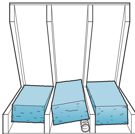
▲ How not to install insulation. Insulation must be in contact with the surface it is intended to insulate, or it will be less effective. There is also the potential to crush the flexible vent duct under the insulation.
