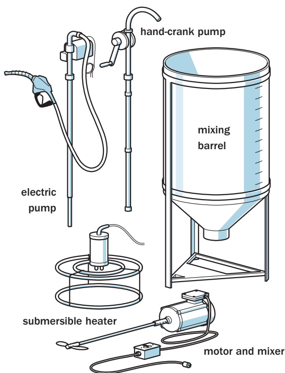
◀ Basic equipment needed to mix a batch of biodiesel
