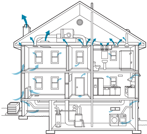
▲ Common paths for air leakage
