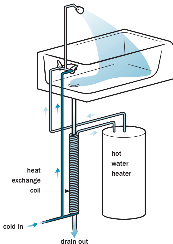
Drain water heat recovery system ▶
