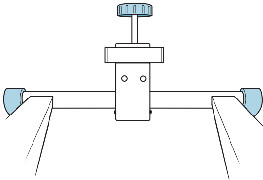
▲ Top view: 1/4" holes drilled through roller bearing mount
