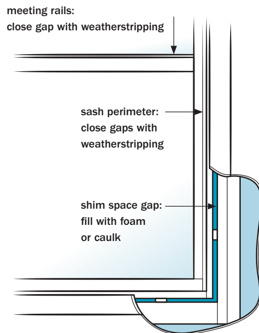
▲ Where windows leak air
