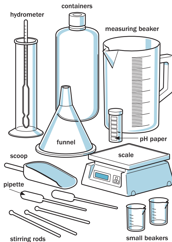
▲ Lab ware required for titration, measuring, weighing, mixing, and testing biodiesel
