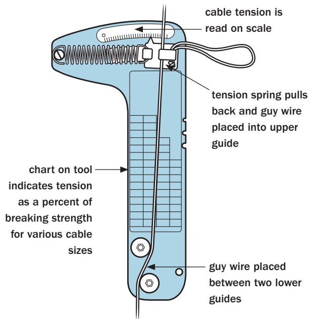
▲ Loose cable tension gauge
