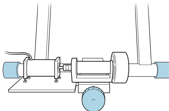
▲ Completed generator and roller assembly
