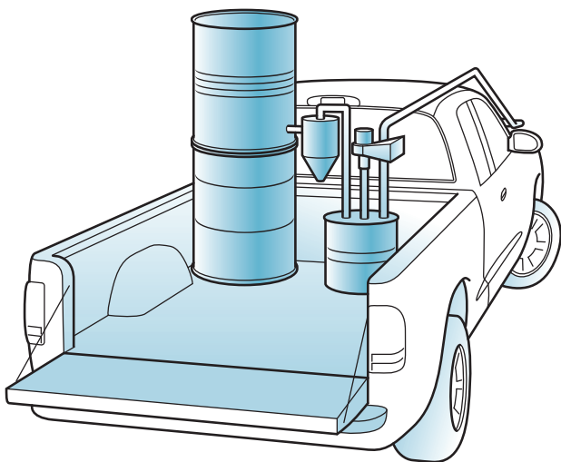
▲ John's gasifier truck
