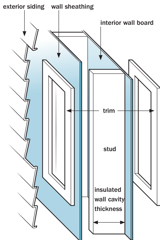
▲ Cutaway of a framed, insulated wall
