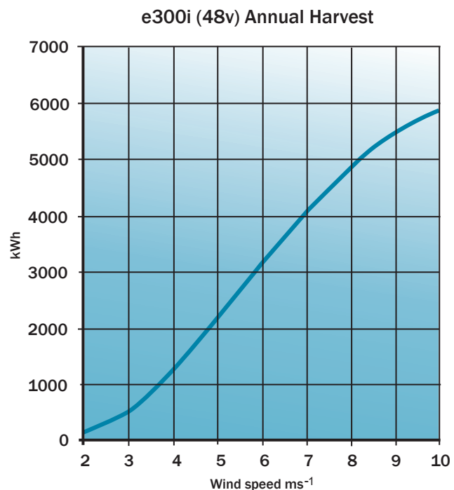
▲ Average energy produced as a function of average annual wind speed for a Kestrel e300i. Image courtesy of Kestrel Renewable Energy, kestrelwind.co.za
