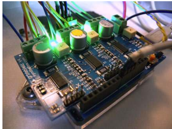
Figure 7-22. The GRBLShield, in addition to an Arduino running one of many 3D printer-compatible firmwares, provides an easy to use 3-stepper driver that can quickly become the basis for your 3D printer's control system.
