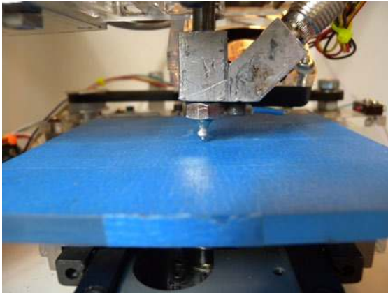
Figure 7-30. Finding the center point of your build platform ensures that your prints are positioned as intended.
