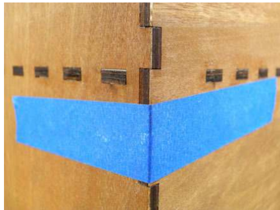
Figure 3-18. Glue works best when it is compressed and undisturbed until it sets.
