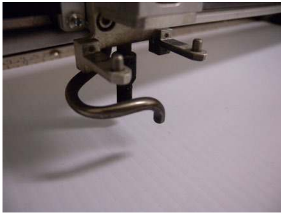
Figure 6-17. The air-assist tube directs a jet of air at the laser's focal point. This helps to prevent flare-ups and directs soot away from the lens assembly.
