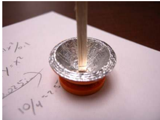
Figure 8-49. The focuser.
