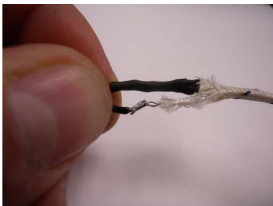
Figure 7-40. You can solder nichrome to copper wire using some fluxes that are designed for stainless steel and chrome. Thoroughly clean away the flux after use as it will corrode the wires.
