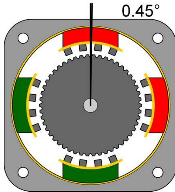
Figure 7-24. Half-step mode.
