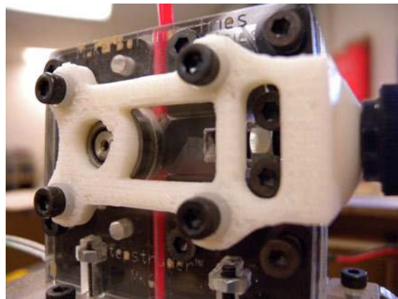
Figure 7-36. The tensioner ensures that the filament is grabbed by the feed wheel. If the tensioner is too loose, the filament will slip. If it is too tight, the filament may jam and the stepper will skip steps.
