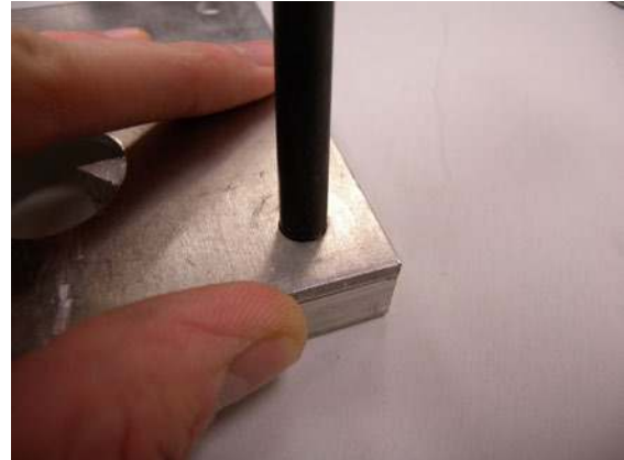
Figure 2-63. Choose a transfer punch that matches the size of the hole. This will ensure a correctly transferred center.
