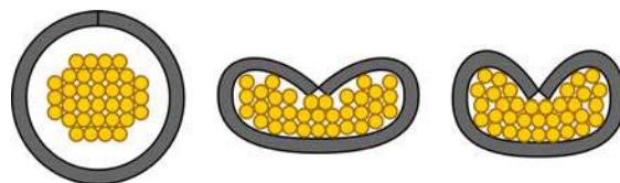
Figure 2-17. Wire crimps use compression to secure an electrical connector to the conductor and require a multistep crimping process.
