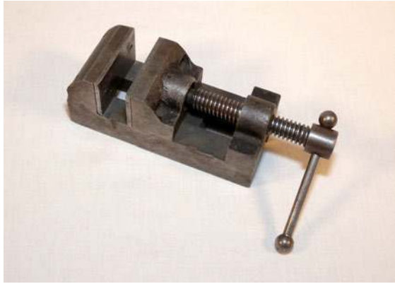
Figure 3-6. Table vise.
