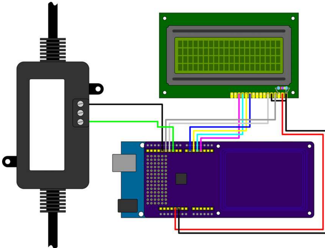
Figure 5-53. Wiring diagram for Arduino RFID power control.
