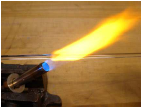
Figure 8-11. Remove the glass from the flame as soon as you create a 3 to 4 mm ball lens. If the lens grows too big, it might fall off of the filament.
