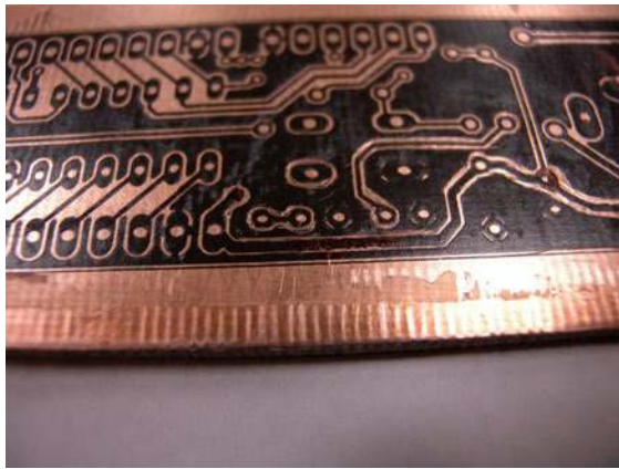
Figure 5-36. Repairing the toner traces.
