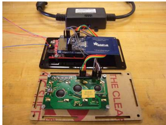
Figure 5-52. The lockout circuit.
