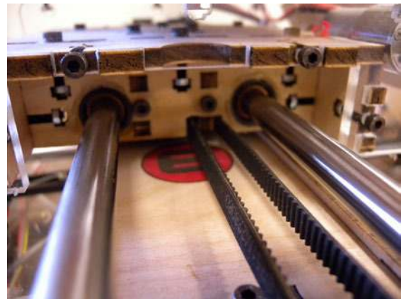
Figure 7-15. Belt-drive mechanism.
