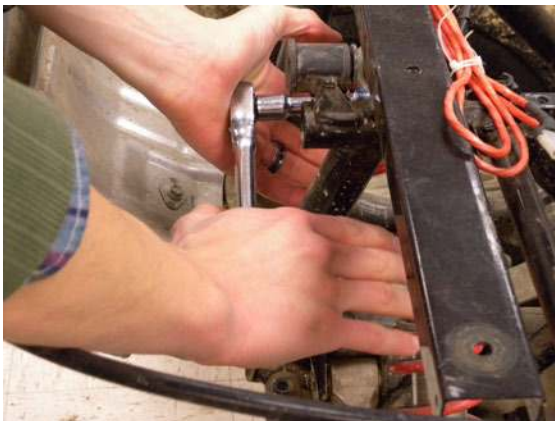
Figure 2-29. When you are attempting to loosen a stuck fastener and you are in close quarters, never wrap your hand completely around the handle. Rather push with your palm and leave your fingers extended. This greatly
