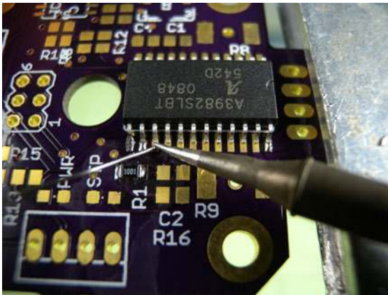
Figure 4-42. Visually inspect the joints as you go to ensure they are properly formed and connected.
