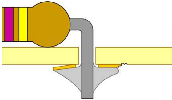
Figure 4-23. An overheated joint.
