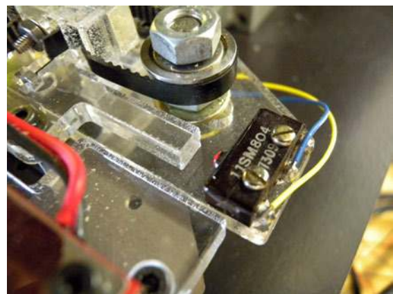
Figure 7-27. Mechanical limit switch.
