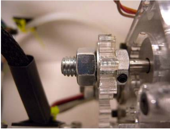
Figure 7-13. A simple nut/bolt shaft coupler.
