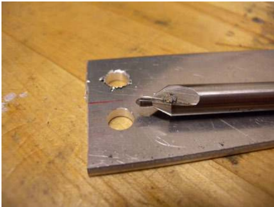
Figure 2-72. Drill centers can be used to clean burs from smaller diameter holes.
