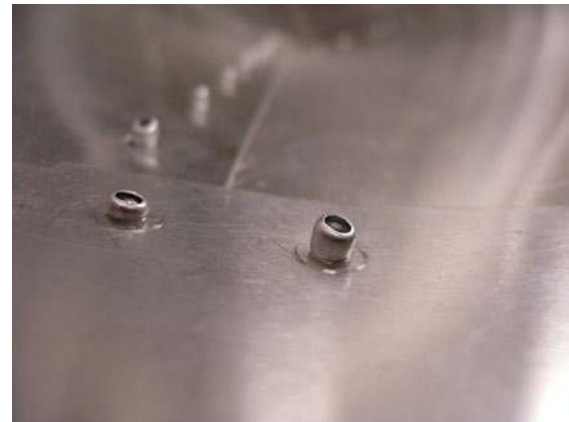
Figure 3-24. After the rivet is compressed, a small piece of the mandrel is left behind, securing the fastener.
