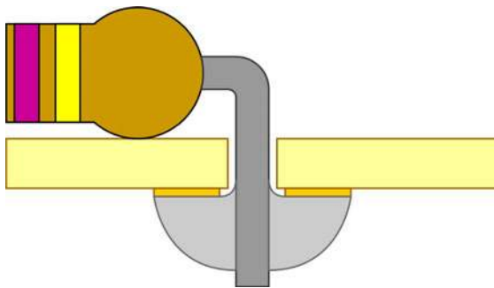
Figure 4-26. Too much solder.
