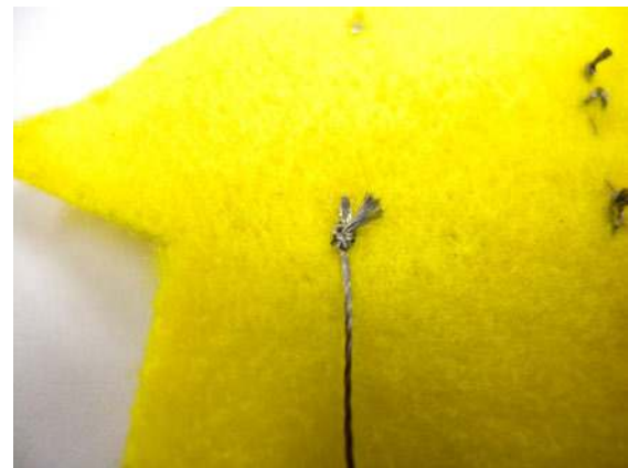
Figure 5-29. Secure components with legs by using a simple two half-hitch knot.
