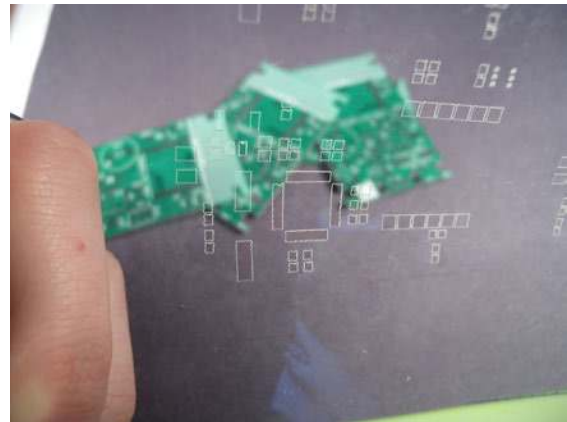
Figure 4-48. A solder stencil.
