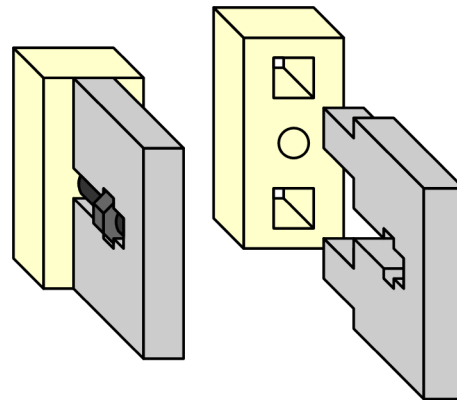
Figure 6-6. Nested-fastener joint.
