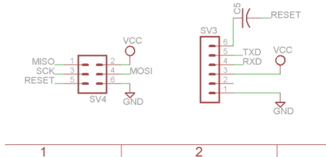
Figure 5-11. Attach the interfaces by using the Wire tool.
