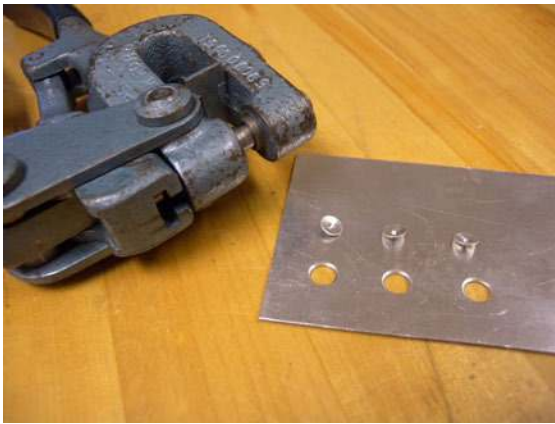
Figure 2-61. Sheet metal punches should be used in lieu of drilling as they are less likely to distort the metal.
