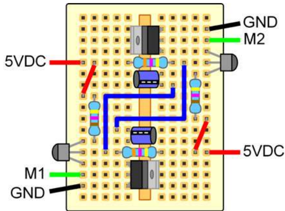
Figure 8-23. Breadboard layout for brushless DC motor controller.
