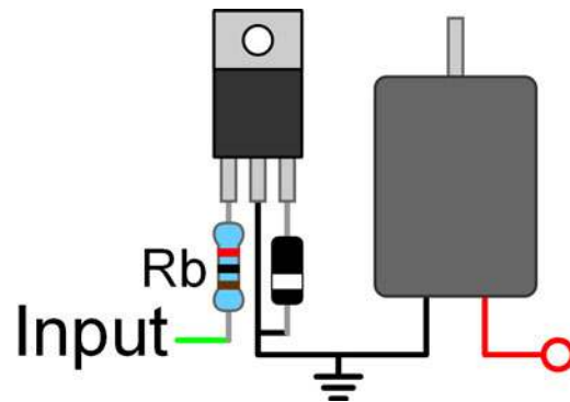
Figure 5-47. Transistor-based motor controller.
