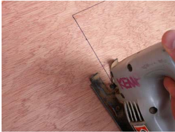
Figure 2-83. A jig saw can be used to make a cutout within a piece of material. This is accomplished by outlining the desired shape and then drilling a hole within the shape that is larger than the saw's blade. The saw can then be guided around the outline, leaving the outside edges of the material untouched.
