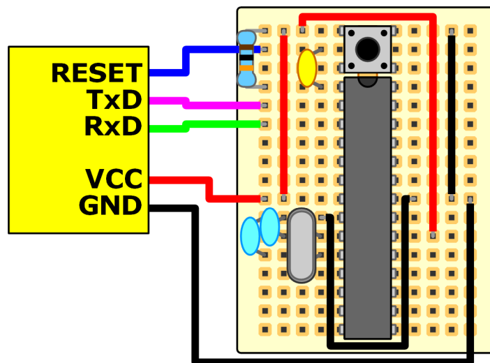
Figure 5-49. Wiring diagram for the breadboard Arduino.
