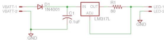
Figure 4-30. Constant-current LED tester schematic.
