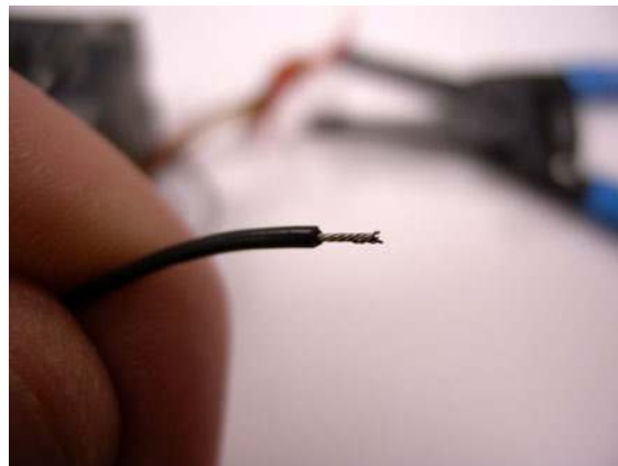
Figure 2-21. Remove only enough insulation to make a proper connection. This is usually between 1/8 and 1/4 in.
