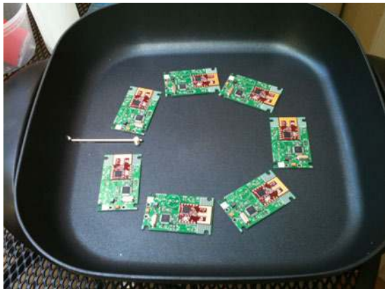
Figure 4-50. Skillet reflow.
