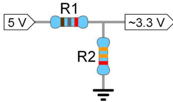
Figure 5-39. The voltage divider.
