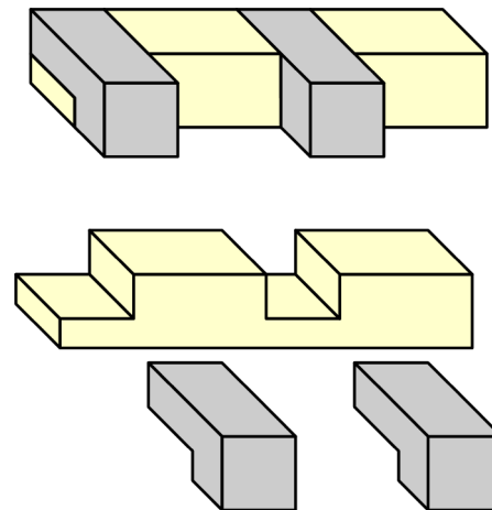
Figure 6-2. Rabbit and lap joints.
