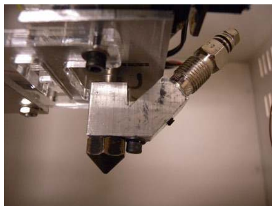
Figure 7-42. Diesel heater.
