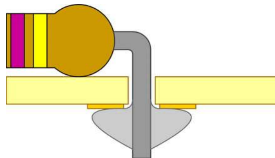
Figure 4-25. Too little solder.
