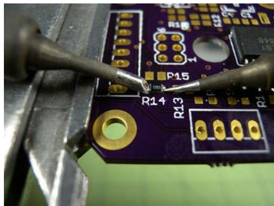
Figure 4-47. Place the component using both irons.
