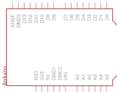
Figure 5-4. Eagle symbol.
