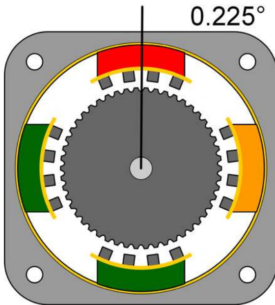
Figure 7-25. Microstep mode.
