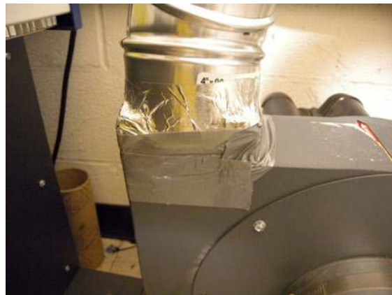
Figure 3-13. Use the correct tape for the job.
