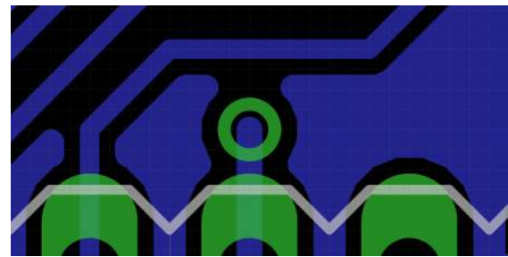
Figure 5-13. A solid ground pour on two-layer designs helps to reduce cross-talk between signal lines and requires less etchant if made by hand. Correct breaks and gaps by adjusting the position of components and traces.
