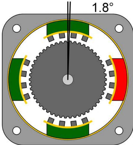
Figure 7-23. Full-step mode.
