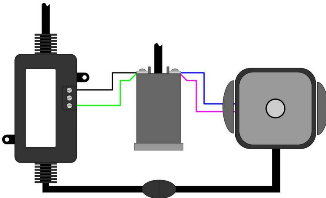
Figure 4-54. Connect the components according to the diagram.
