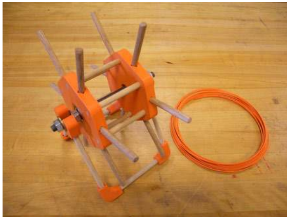
Figure 7-2. Filament spool holder.
