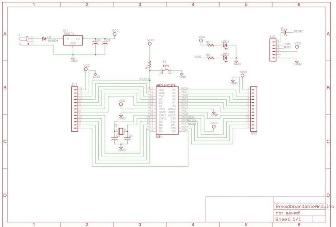
Figure 5-9. The completed schematic.
