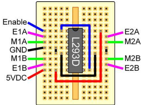
Figure 8-21. L293D breadboard layout.
