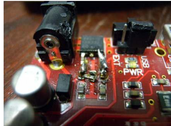
Figure 4-22. A scorched circuit board.
