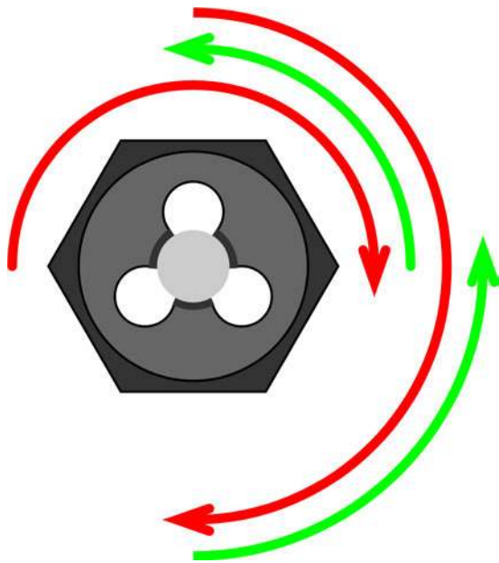
Figure 2-41. Thread Cutting Procedure.
