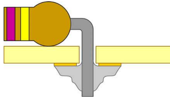
Figure 4-24. Cold solder joint.
