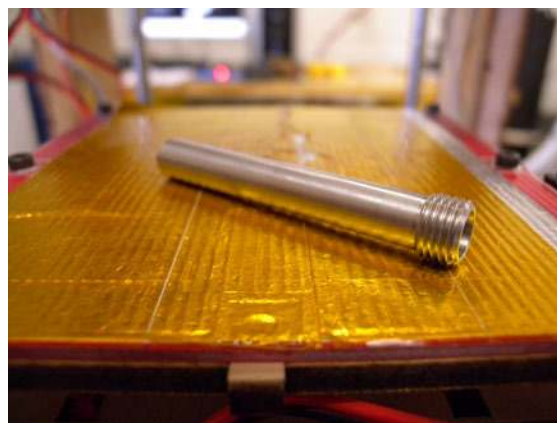
Figure 7-37. Heater barrel.
