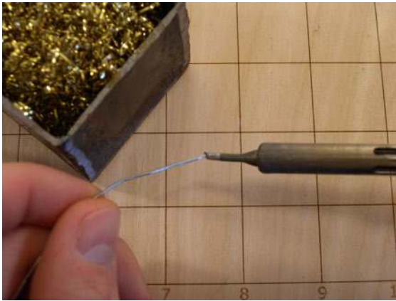
Figure 4-9. Soldering iron tips work better and last longer when tinned using a small amount of solder.
