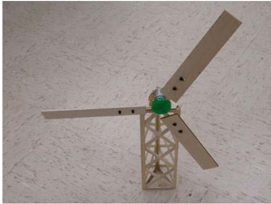
Figure 8-26. The completed turbine.
