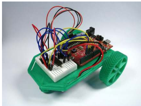
Figure 8-19. The completed robot.
