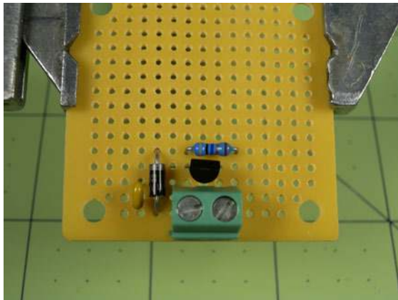
Figure 4-31. Position the components as shown.
